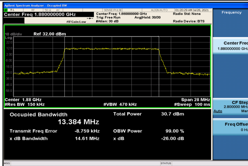
Band2-15MHz-QPSK-18900-75RB#0-13.384
