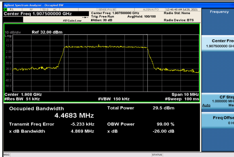
Band2-5MHz-16QAM-19175-25RB#0-4.4683
