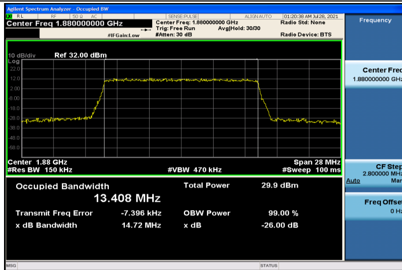
Band2-15MHz-16QAM-18900-75RB#0-13.408
