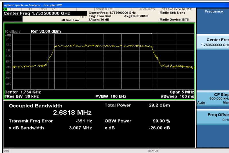
Band4-3MHz-16QAM-20385-15RB#0-2.6818
