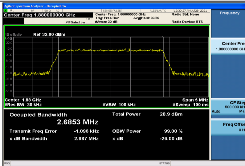
Band2-3MHz-16QAM-18900-15RB#0-2.6853
