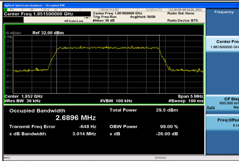
Band2-3MHz-16QAM-18615-15RB#0-2.6896
