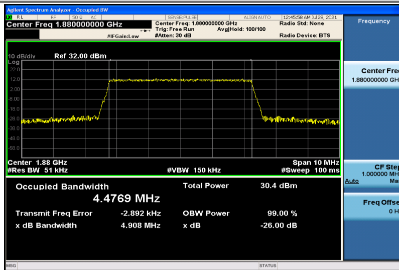
Band2-5MHz-QPSK-18900-25RB#0-4.4769
