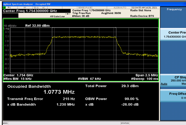
Band4-1.4MHz-QPSK-20393-6RB#0-1.0773
