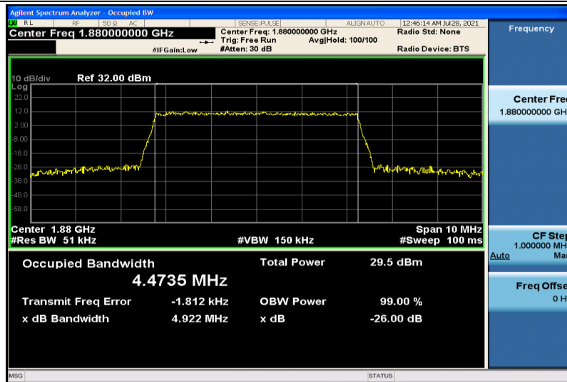
Band2-5MHz-16QAM-18900-25RB#0-4.4735
