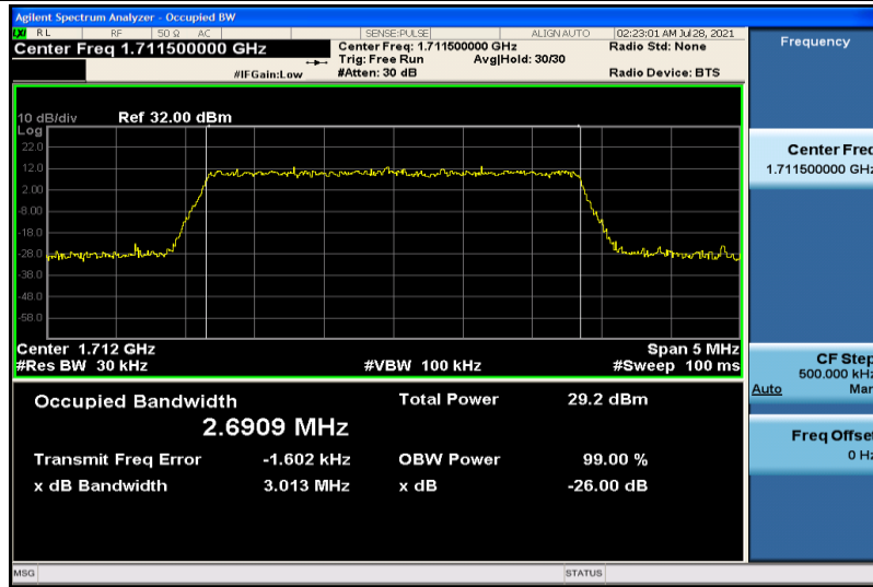
Band4-3MHz-16QAM-19965-15RB#0-2.6909
