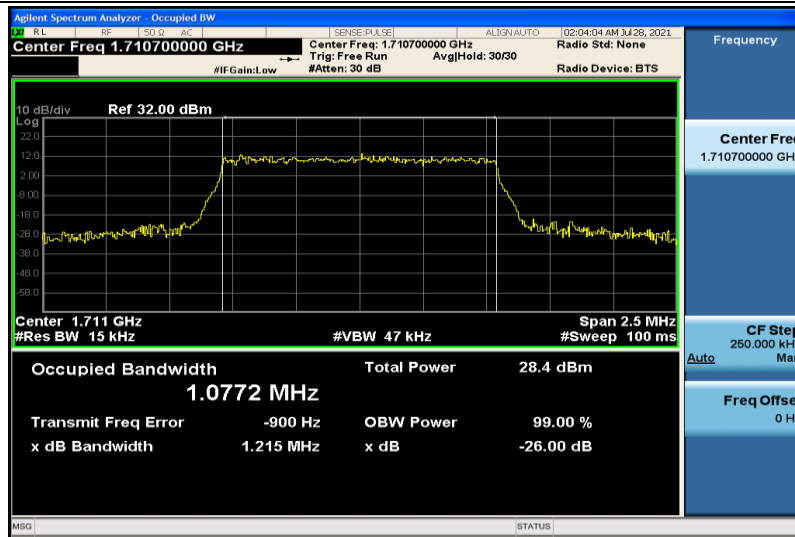
Band4-1.4MHz-16QAM-19957-6RB#0-1.0772
