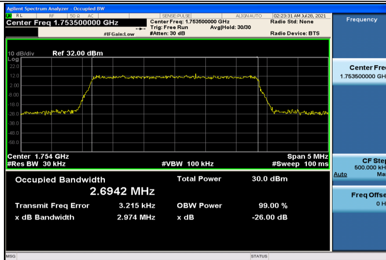
Band4-3MHz-QPSK-20385-15RB#0-2.6942
