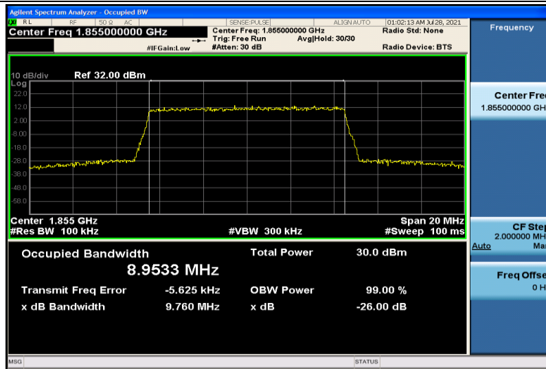
Band2-10MHz-16QAM-18650-50RB#0-8.9533
