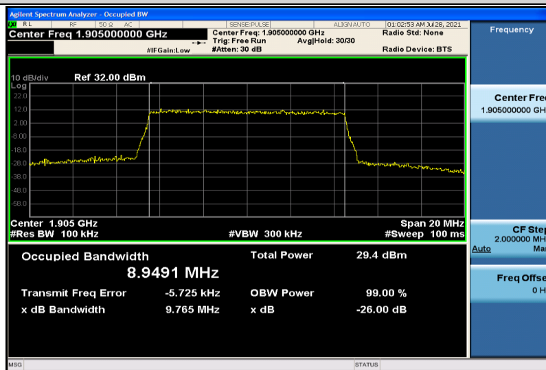
Band2-10MHz-16QAM-19150-50RB#0-8.9491
