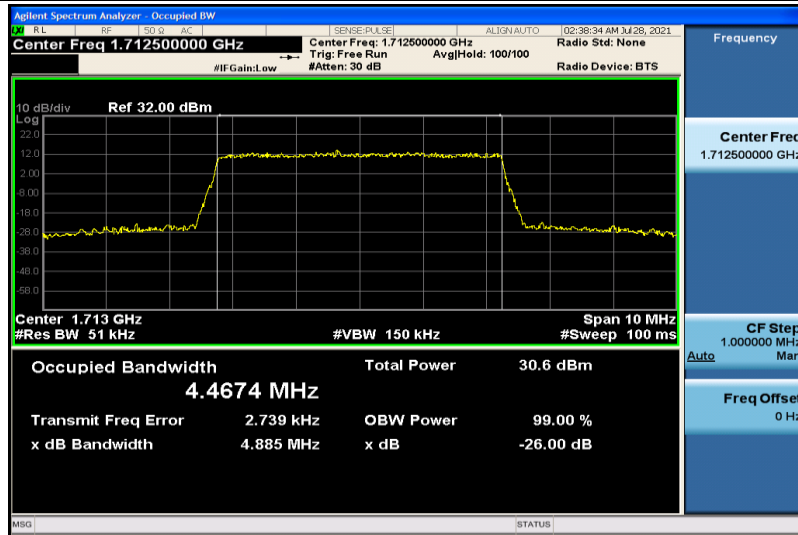
Band4-5MHz-QPSK-19975-25RB#0-4.4674
