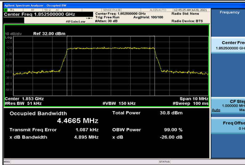
Band2-5MHz-QPSK-18625-25RB#0-4.4665
