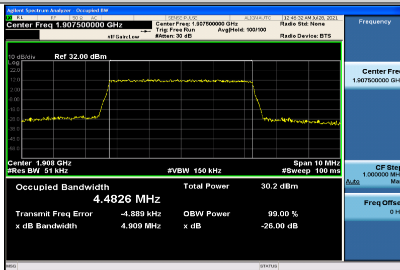
Band2-5MHz-QPSK-19175-25RB#0-4.4826
