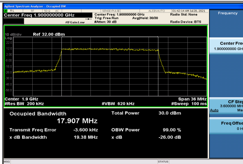
Band2-20MHz-16QAM-19100-100RB#0-17.907
