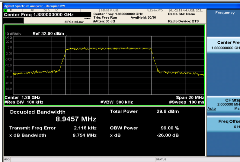
Band2-10MHz-16QAM-18900-50RB#0-8.9457
