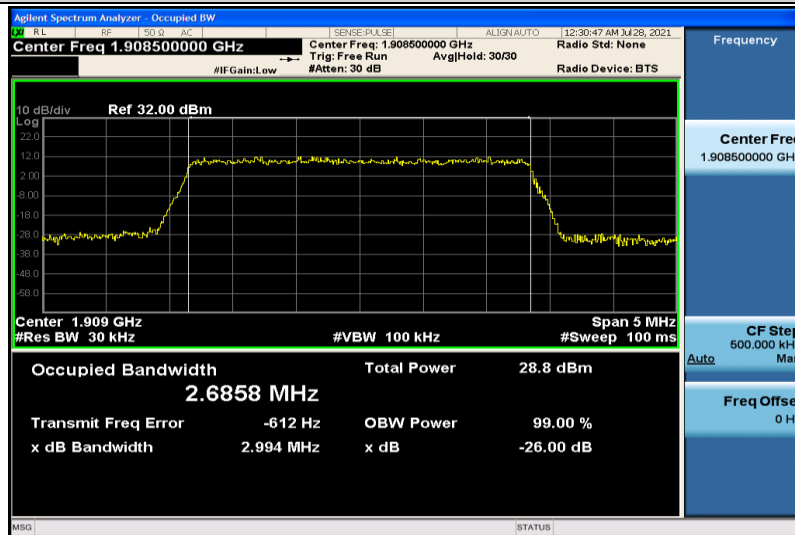
Band2-3MHz-16QAM-19185-15RB#0-2.6858
