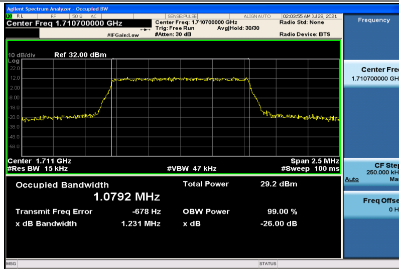
Band4-1.4MHz-QPSK-19957-6RB#0-1.0792
