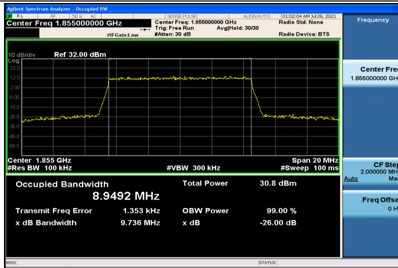
Band2-10MHz-QPSK-18650-50RB#0-8.9492
