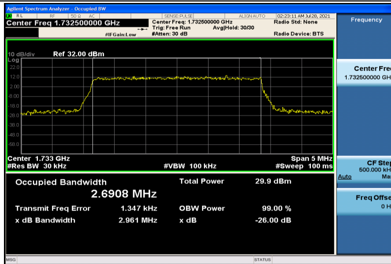
Band4-3MHz-QPSK-20175-15RB#0-2.6908
