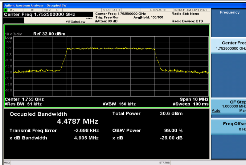
Band4-5MHz-QPSK-20175-25RB#0-4.4787
