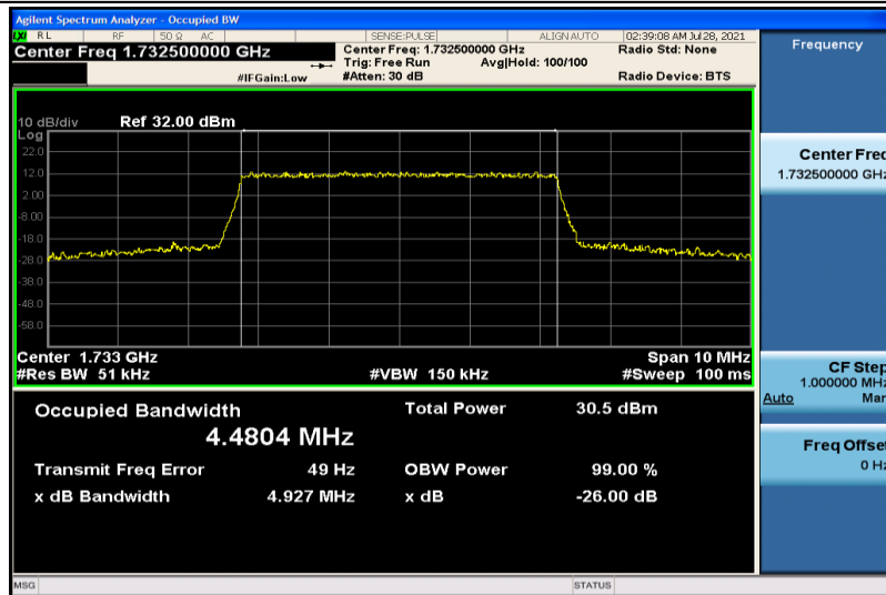
Band4-5MHz-QPSK-17325-25RB#0-4.4804
