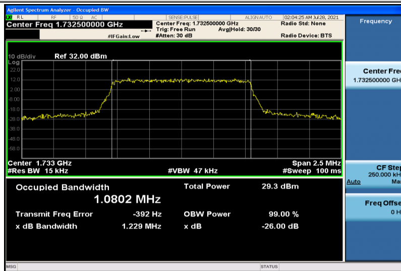
Band4-1.4MHz-QPSK-20175-6RB#0-1.0802
