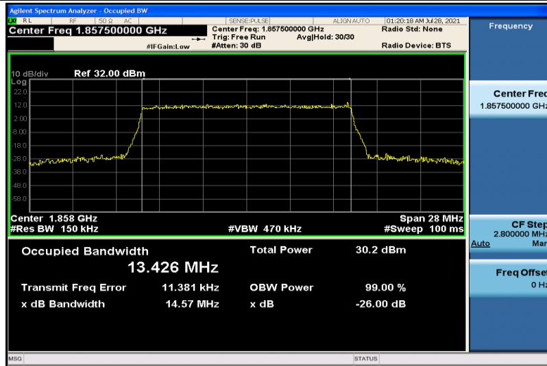
Band2-15MHz-16QAM-18675-75RB#0-13.426
