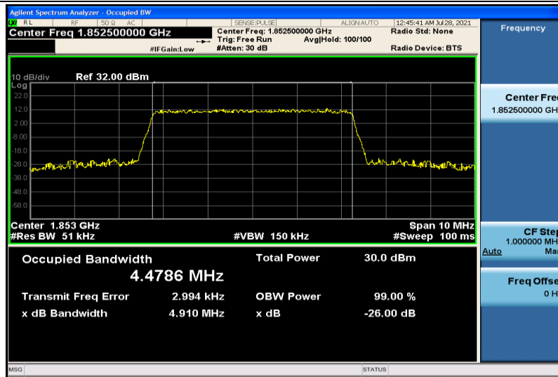
Band2-5MHz-16QAM-18625-25RB#0-4.4786
