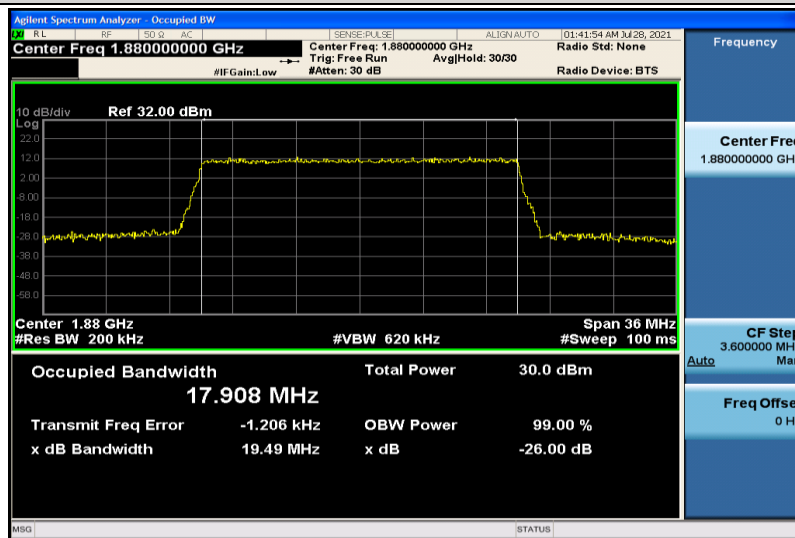
Band2-20MHz-16QAM-18900-100RB#0-17.908
