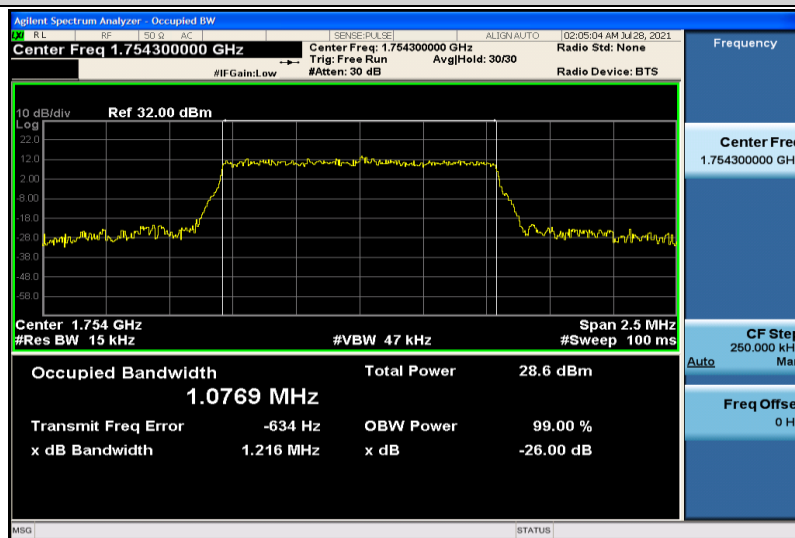
Band4-1.4MHz-16QAM-20393-6RB#0-1.0769
