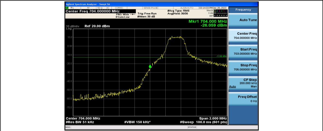
Band17-5MHz-16QAM-23755-1RB#0
