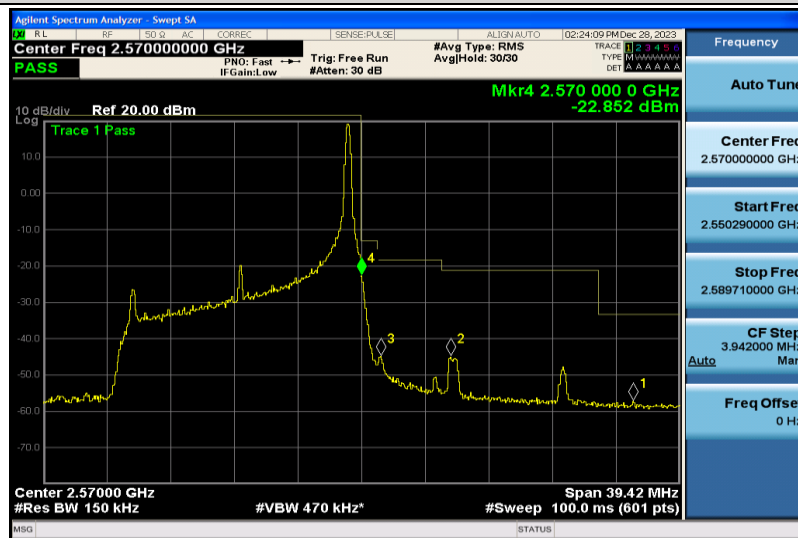
Band7-15MHz-QPSK-21375-1RB#74
