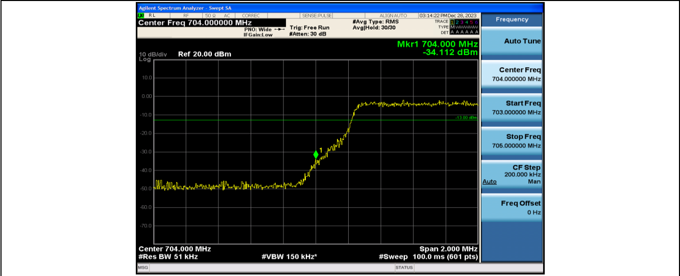
Band17-5MHz-16QAM-23755-25RB#0
