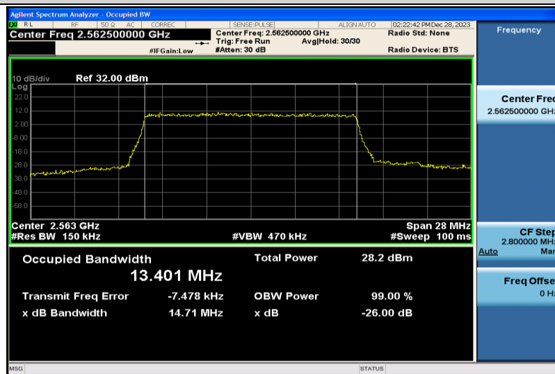
Band7-15MHz-QPSK-21375-75RB#0-13.401
