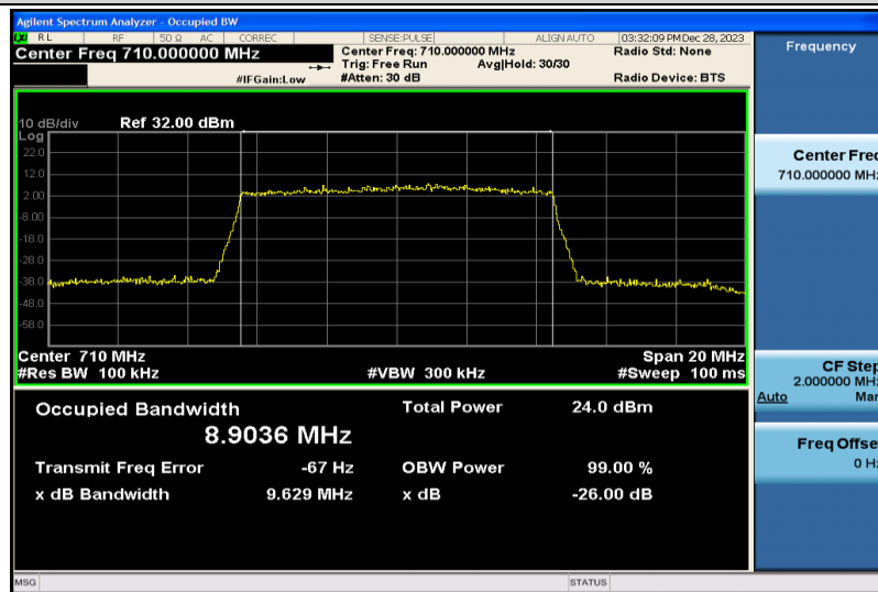
Band17-10MHz-QPSK-23790-50RB#0-8.9036
