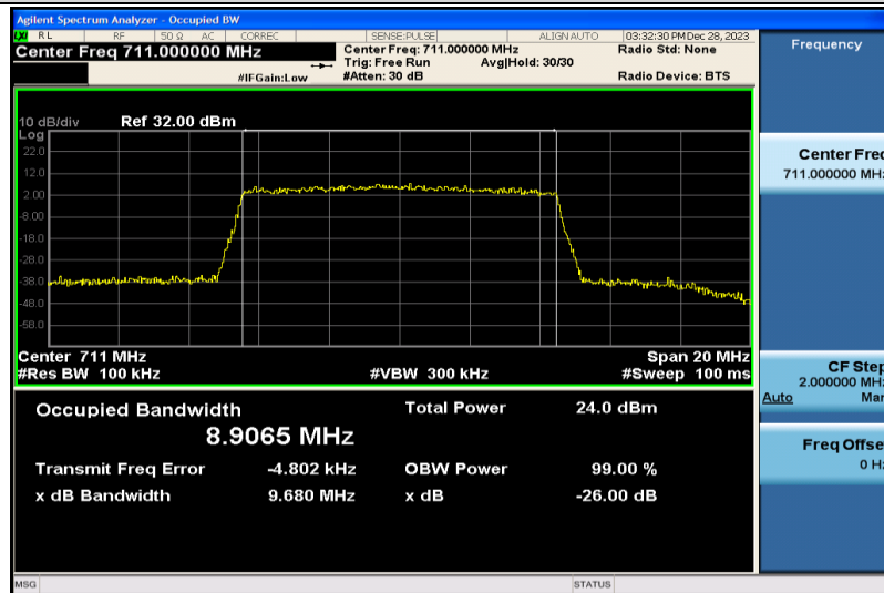
Band17-10MHz-QPSK-23800-50RB#0-8.9065
