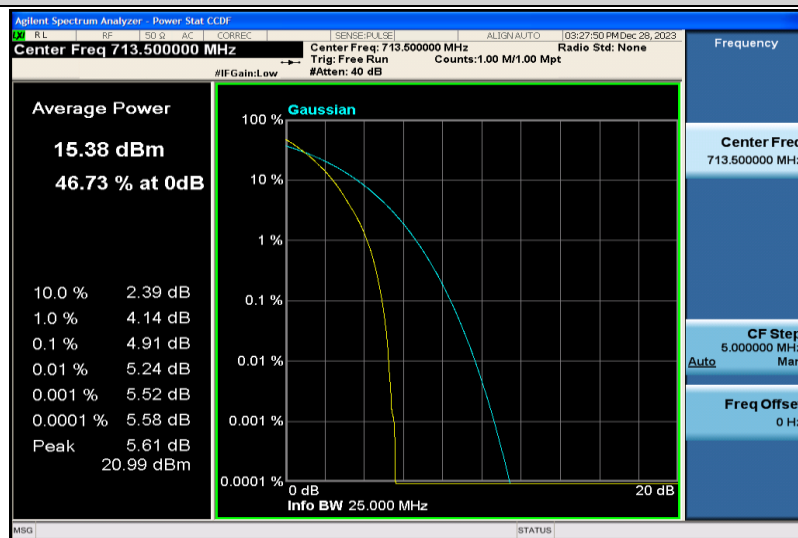
Band17-5MHz-QPSK-23825-25RB#0
