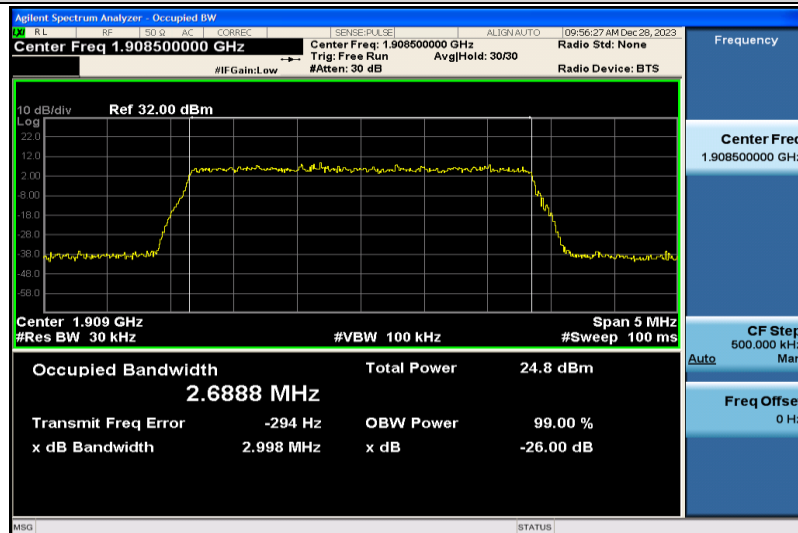
Band2-3MHz-16QAM-19185-15RB#0-2.6888
