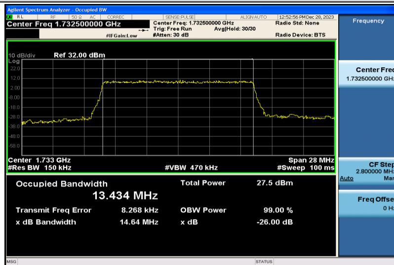
Band4-15MHz-QPSK-20175-75RB#0-13.434
