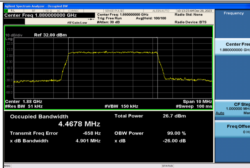
Band2-5MHz-QPSK-18900-25RB#0-4.4678
