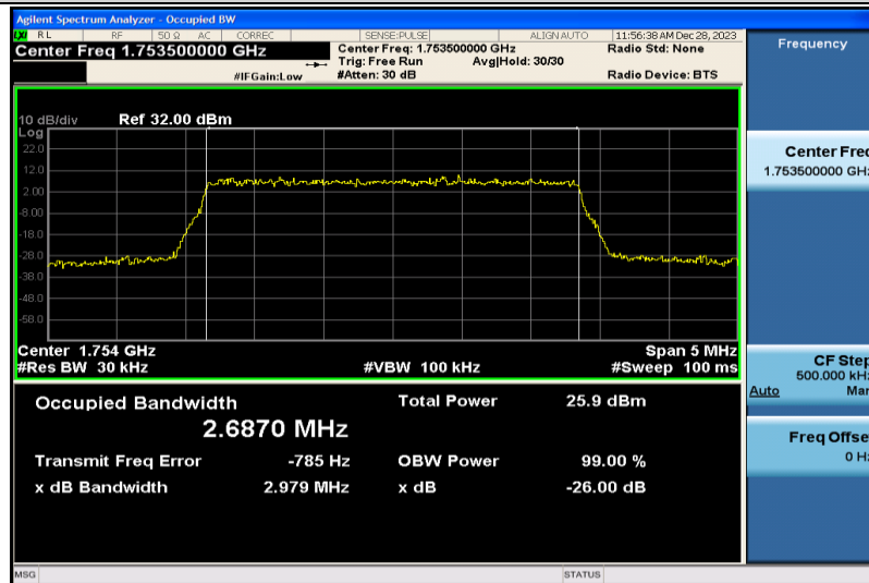
Band4-3MHz-QPSK-20385-15RB#0-2.6870
