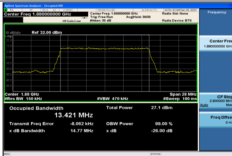
Band2-15MHz-QPSK-18900-75RB#0-13.421
