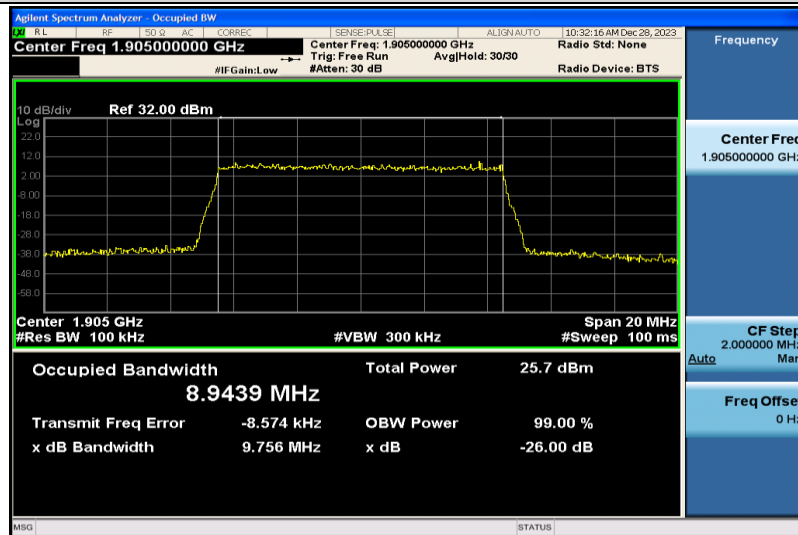
Band2-10MHz-16QAM-19150-50RB#0-8.9439
