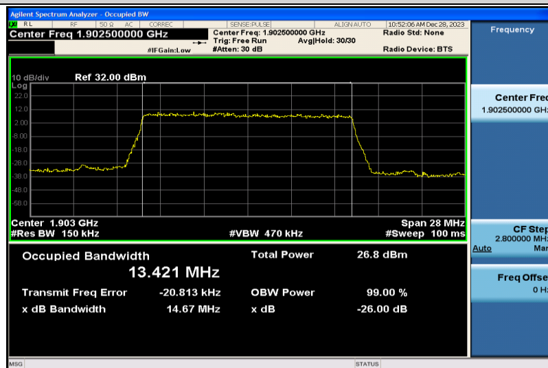
Band2-15MHz-QPSK-19125-75RB#0-13.421
