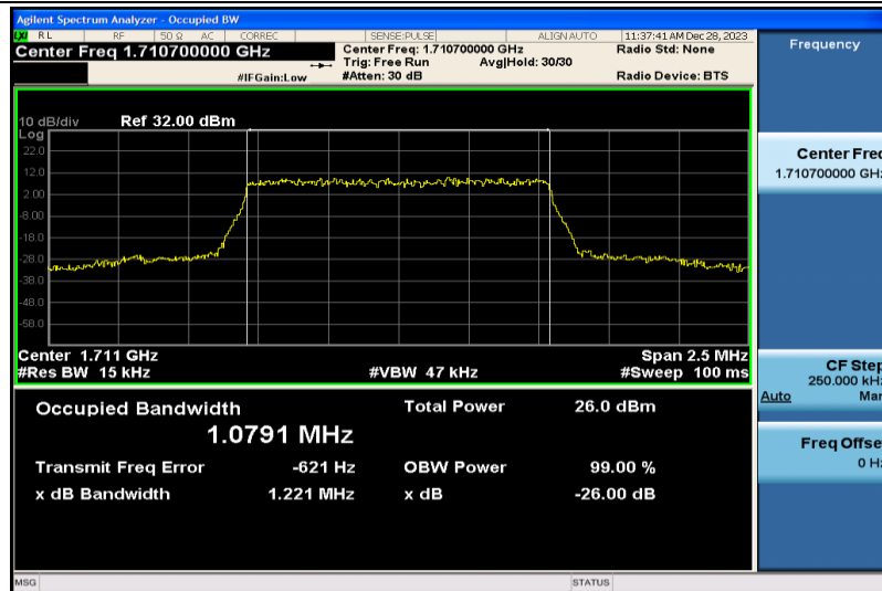
Band4-1.4MHz-QPSK-19957-6RB#0-1.0791
