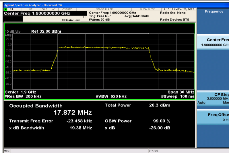
Band2-20MHz-16QAM-19100-100RB#0-17.872
