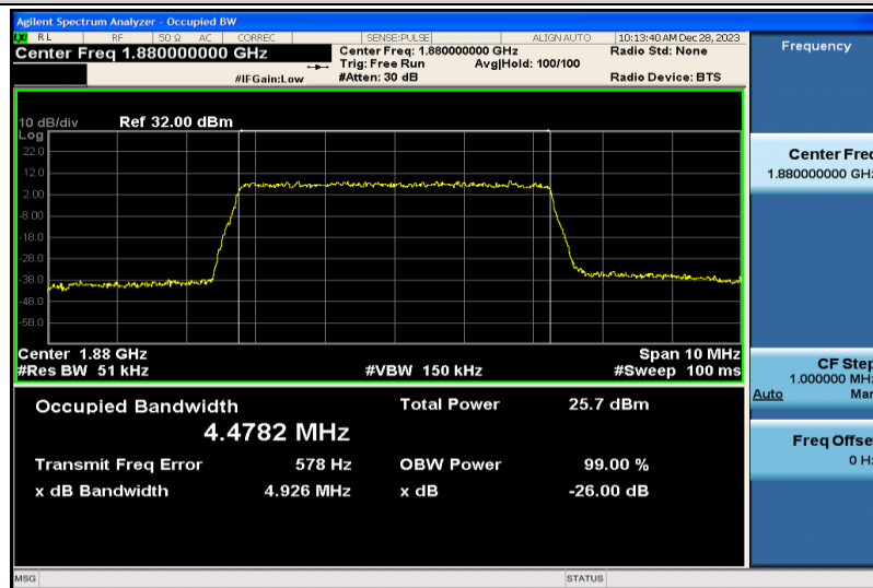
Band2-5MHz-16QAM-18900-25RB#0-4.4782
