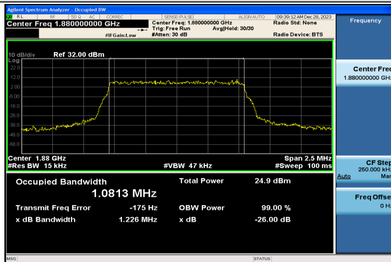
Band2-1.4MHz-QPSK-18900-6RB#0-1.0813
