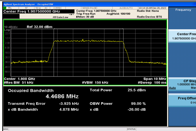
Band2-5MHz-16QAM-19175-25RB#0-4.4686
