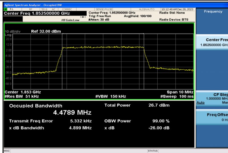
Band2-5MHz-QPSK-18625-25RB#0-4.4789
