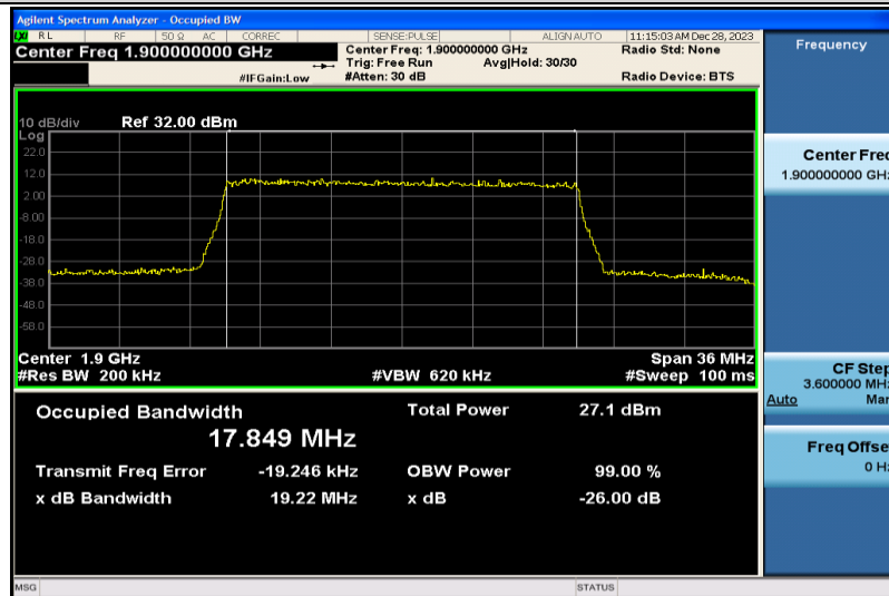
Band2-20MHz-QPSK-19100-100RB#0-17.849
