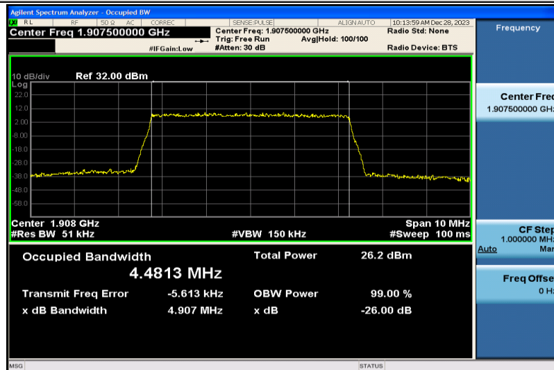
Band2-5MHz-QPSK-19175-25RB#0-4.4813
