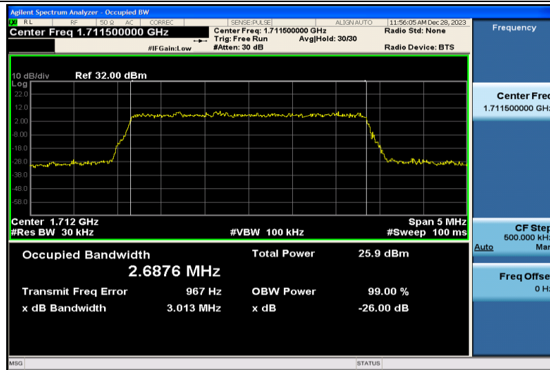
Band4-3MHz-16QAM-19965-15RB#0-2.6876
