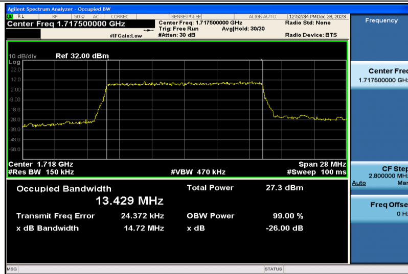
Band4-15MHz-QPSK-20025-75RB#0-13.429
