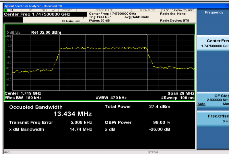
Band4-15MHz-QPSK-20325-75RB#0-13.434
