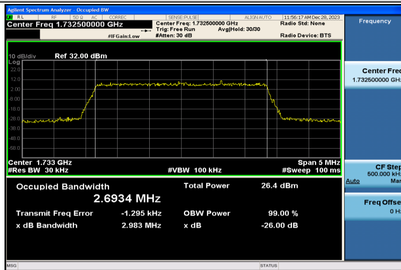
Band4-3MHz-QPSK-20175-15RB#0-2.6934
