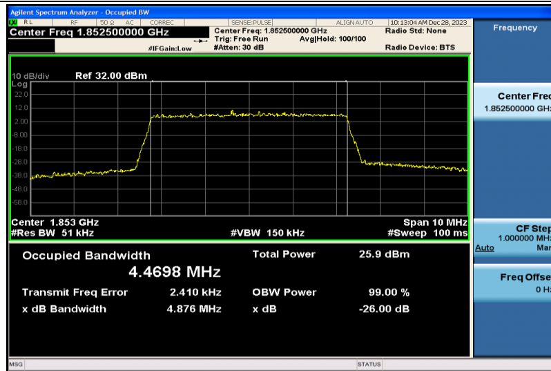
Band2-5MHz-16QAM-18625-25RB#0-4.4698
