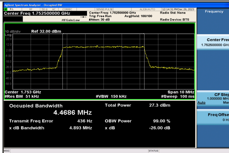
Band4-5MHz-QPSK-20375-25RB#0-4.4686
