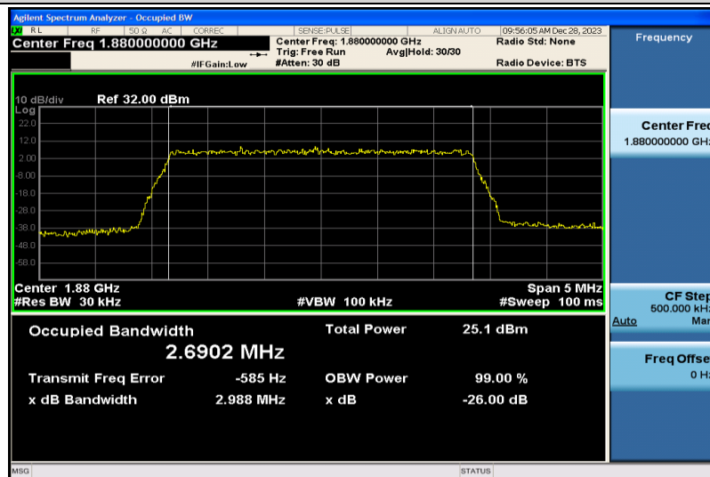
Band2-3MHz-16QAM-18900-15RB#0-2.6902
