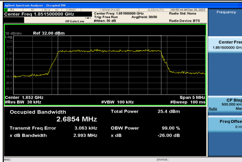
Band2-3MHz-16QAM-18615-15RB#0-2.6854
