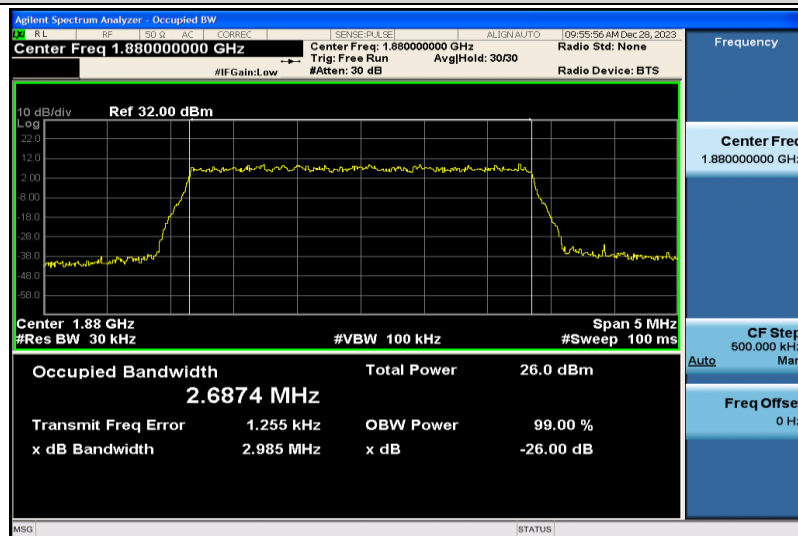
Band2-3MHz-QPSK-18900-15RB#0-2.6874
