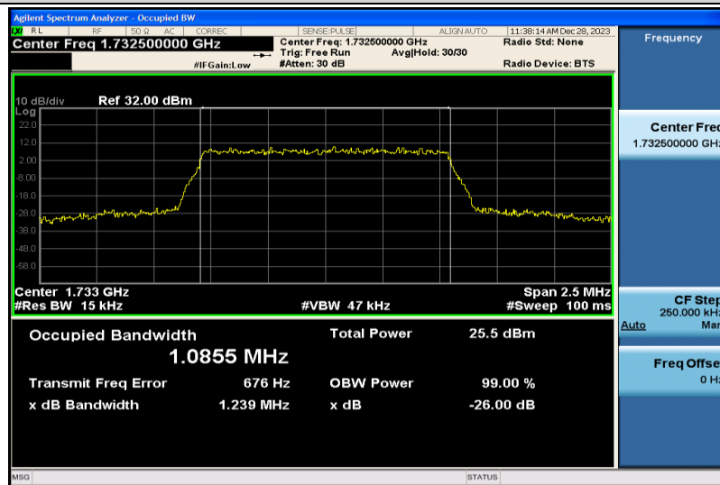
Band4-1.4MHz-16QAM-20175-6RB#0-1.0855
