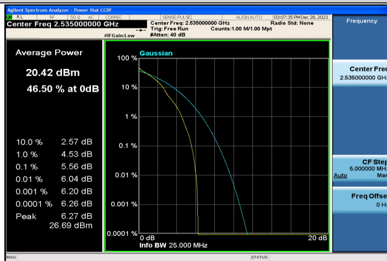
Band7-20MHz-QPSK-21100-1RB#0
