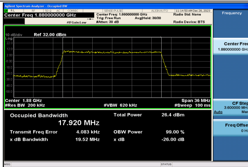
Band2-20MHz-16QAM-18900-100RB#0-17.920
