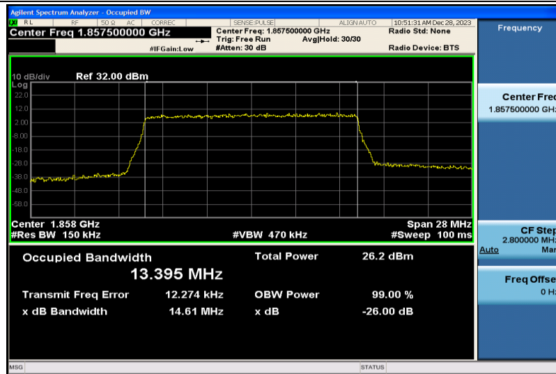
Band2-15MHz-16QAM-18675-75RB#0-13.395
