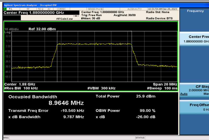
Band2-10MHz-16QAM-18900-50RB#0-8.9646
