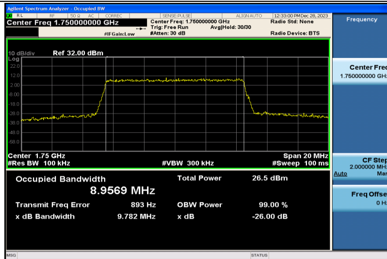
Band4-10MHz-16QAM-20350-50RB#0-8.9569
