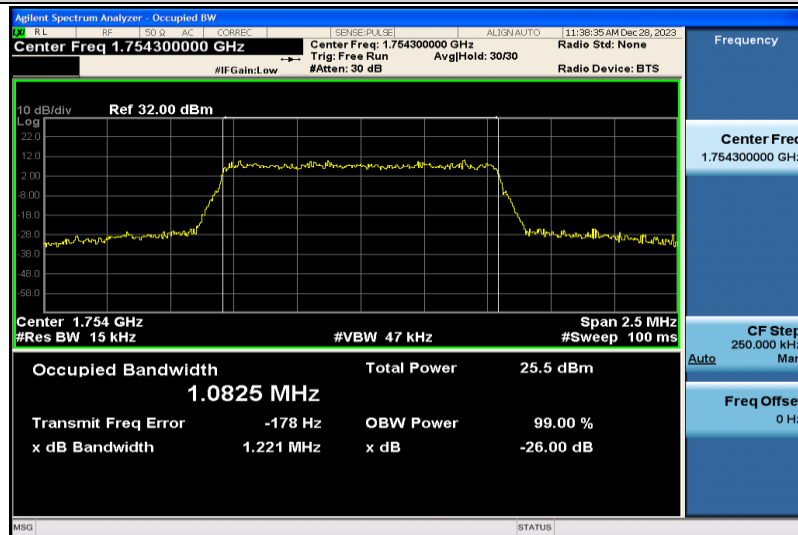
Band4-1.4MHz-16QAM-20393-6RB#0-1.0825
