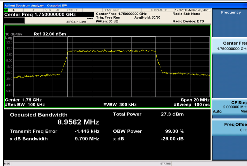
Band4-10MHz-QPSK-20350-50RB#0-8.9562
