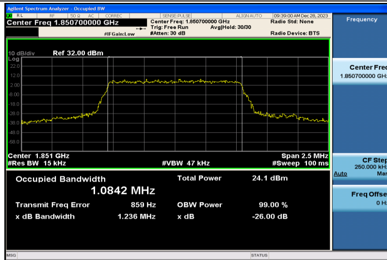
Band2-1.4MHz-16QAM-18607-6RB#0-1.0842
