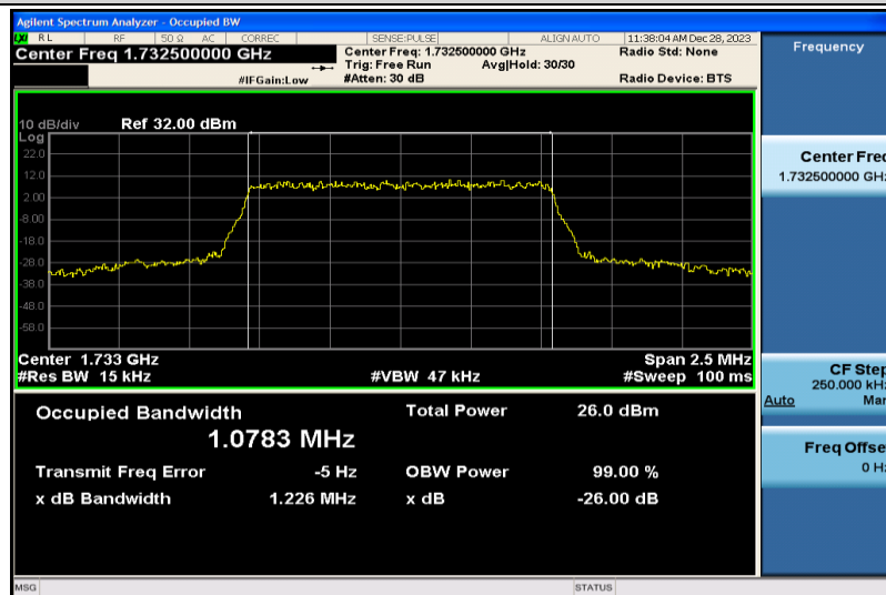
Band4-1.4MHz-QPSK-20175-6RB#0-1.0783
