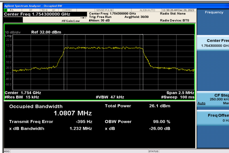
Band4-1.4MHz-QPSK-20393-6RB#0-1.0807
