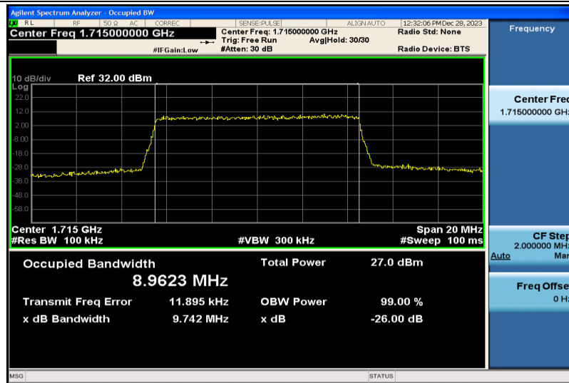
Band4-10MHz-QPSK-20000-50RB#0-8.9623
