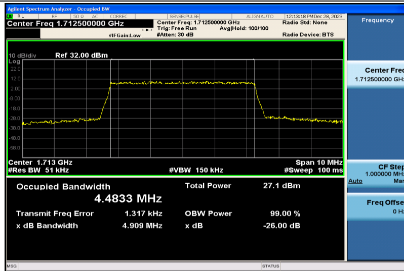
Band4-5MHz-QPSK-19975-25RB#0-4.4833
