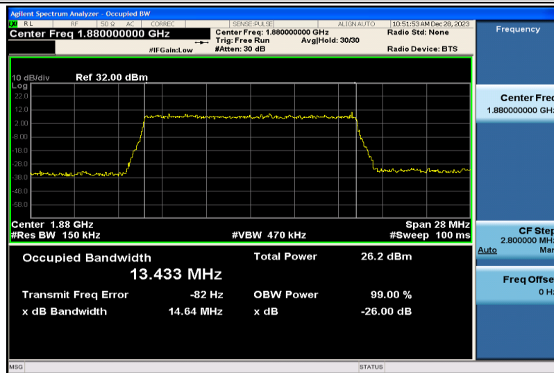
Band2-15MHz-16QAM-18900-75RB#0-13.433
