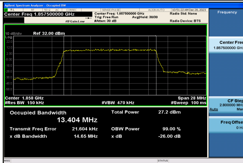
Band2-15MHz-QPSK-18675-75RB#0-13.404
