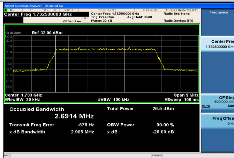
Band4-3MHz-16QAM-20175-15RB#0-2.6914
