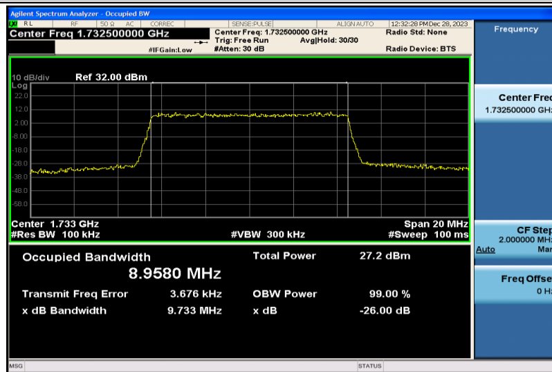
Band4-10MHz-QPSK-20175-50RB#0-8.9580
