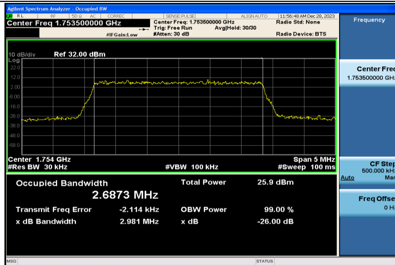
Band4-3MHz-16QAM-20385-15RB#0-2.6873
