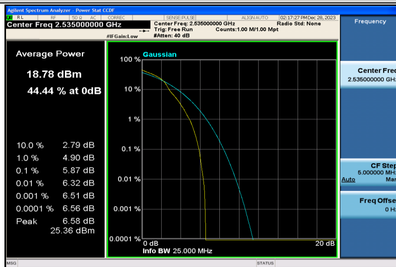
Band7-10MHz-16QAM-21100-1RB#0
