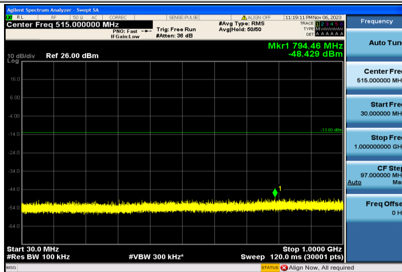
Band4-20MHz-16QAM-20300-1RB#0-30~1000MHz
