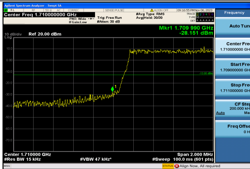
Band4-1.4MHz-QPSK-1957-6RB#0
