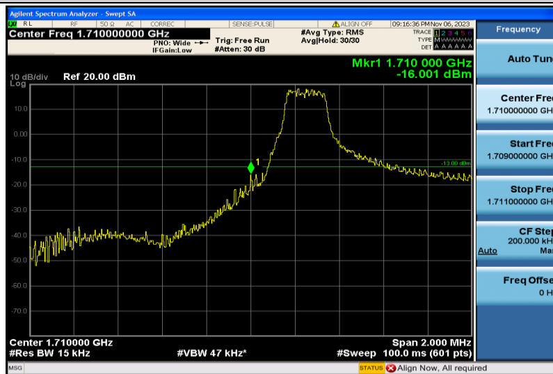
Band4-1.4MHz-QPSK-1957-1RB#0
