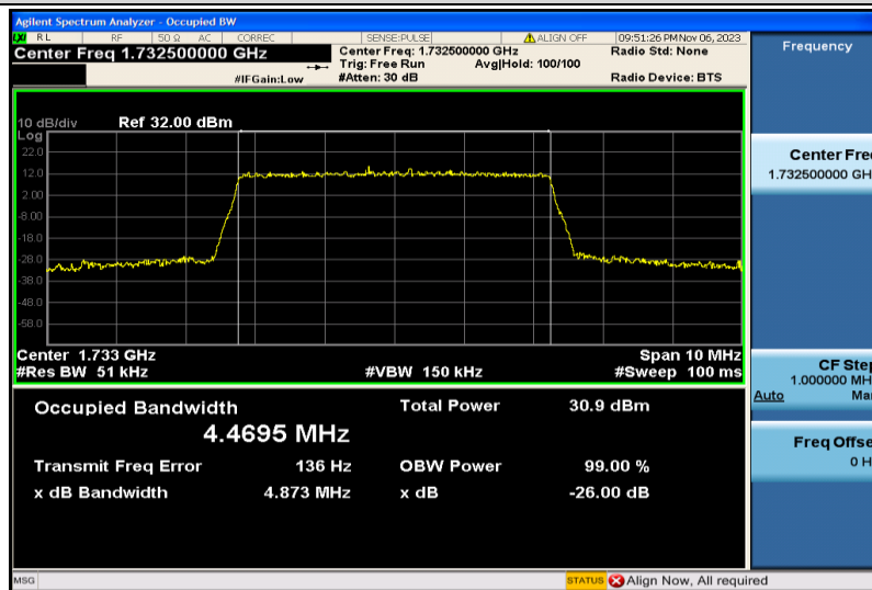
Band4-5MHz-16QAM-20175-25RB#0-4.4695
