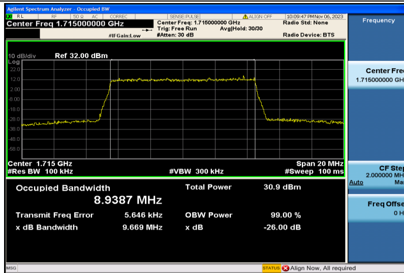
Band4-10MHz-16QAM-20000-50RB#0-8.9387
