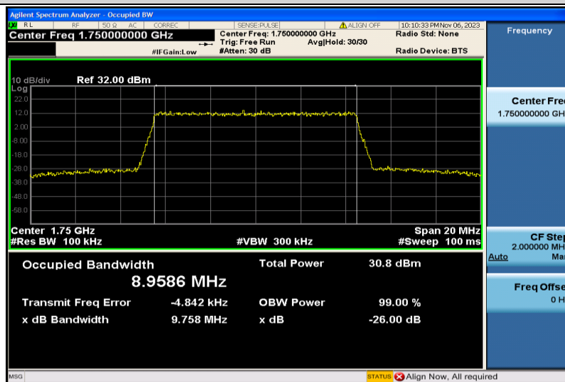
Band4-10MHz-16QAM-20350-50RB#0-8.9586
