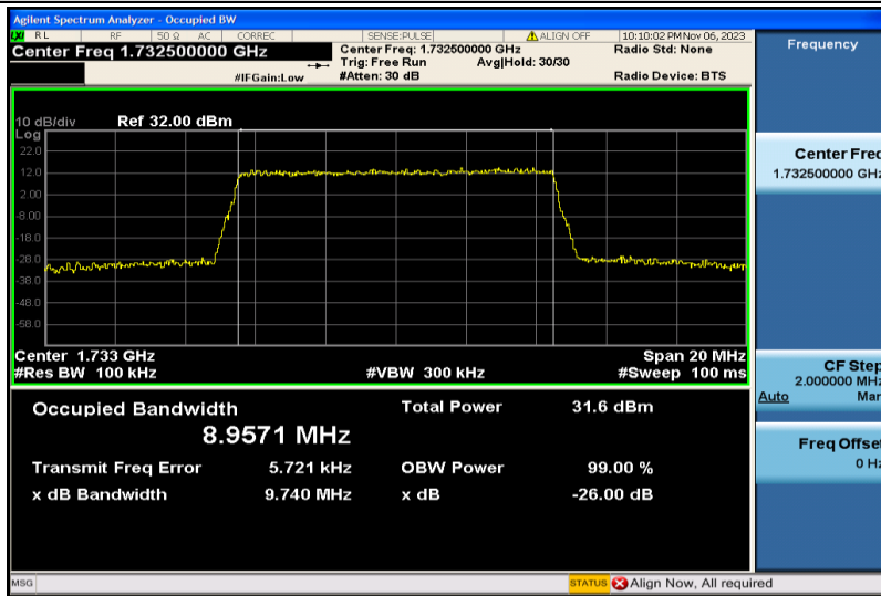
Band4-10MHz-QPSK-20175-50RB#0-8.9571
