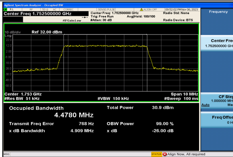
Band4-5MHz-16QAM-20375-25RB#0-4.4780
