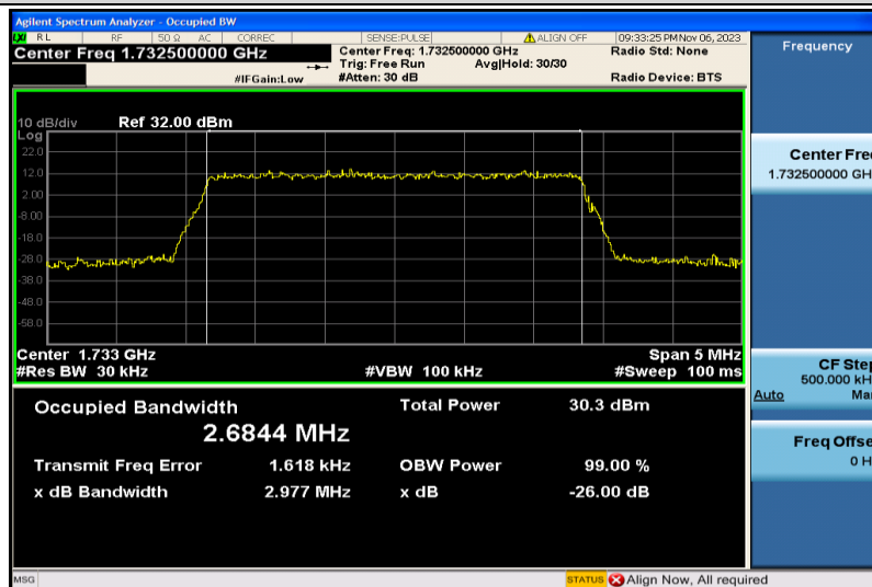
Band4-3MHz-16QAM-20175-15RB#0-2.6844
