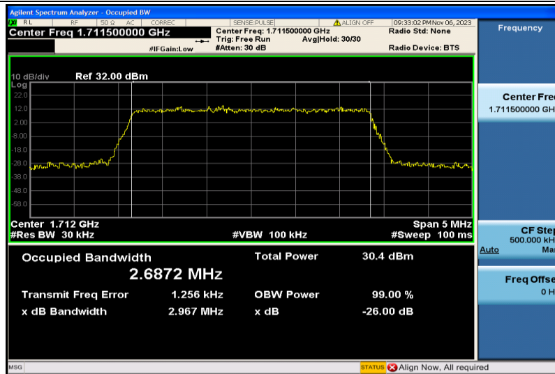
Band4-3MHz-16QAM-19965-15RB#0-2.6872
