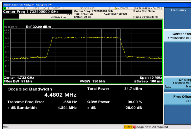
Band4-5MHz-QPSK-17325-25RB#0-4.4802
