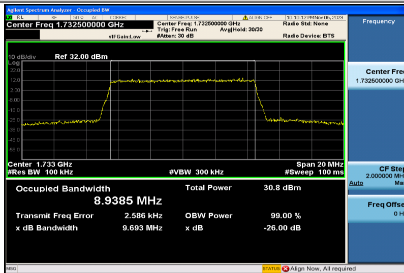
Band4-10MHz-16QAM-20175-50RB#0-8.9385
