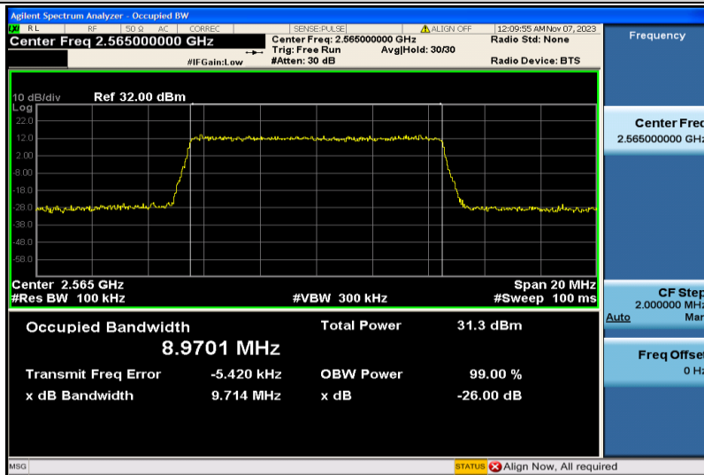
Band7-10MHz-QPSK-21400-50RB#0-8.9701
