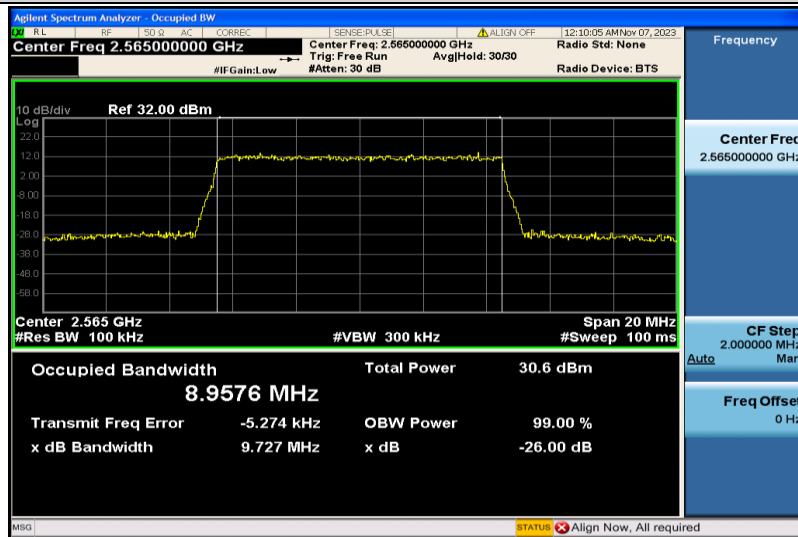
Band7-10MHz-16QAM-21400-50RB#0-8.9576
