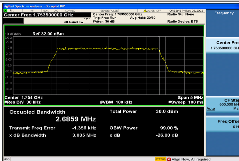
Band4-3MHz-16QAM-20385-15RB#0-2.6859
