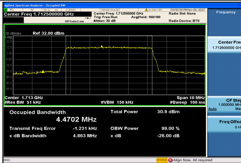
Band4-5MHz-16QAM-19975-25RB#0-4.4702
