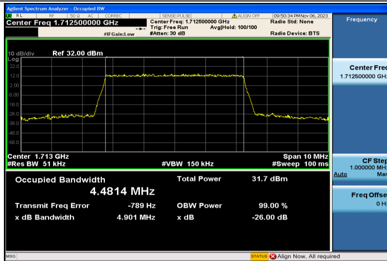
Band4-5MHz-QPSK-19975-25RB#0-4.4814
