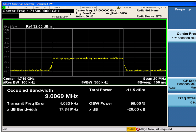
Band4-10MHz-QPSK-20000-50RB#0-9.0069
