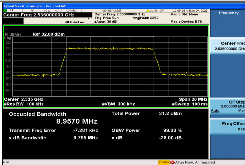
Band7-10MHz-QPSK-21100-50RB#0-8.9570
