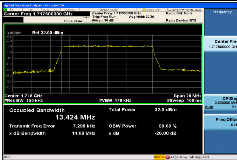
Band4-15MHz-QPSK-20025-75RB#0-13.424
