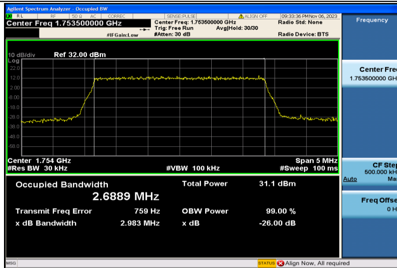
Band4-3MHz-QPSK-20385-15RB#0-2.6889
