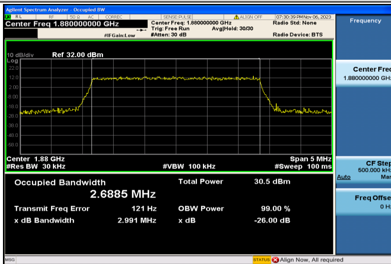
Band2-3MHz-QPSK-18900-15RB#0-2.6885
