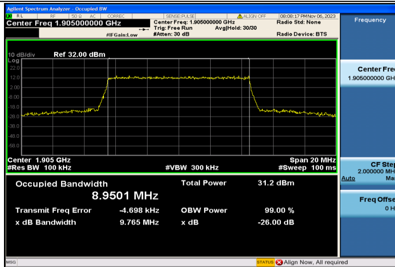
Band2-10MHz-16QAM-19150-50RB#0-8.9501
