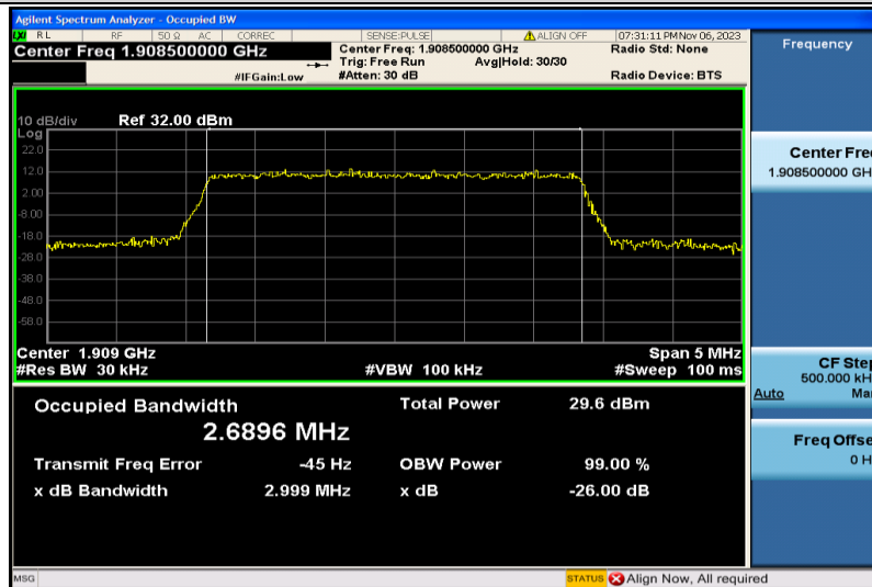
Band2-3MHz-16QAM-19185-15RB#0-2.6896
