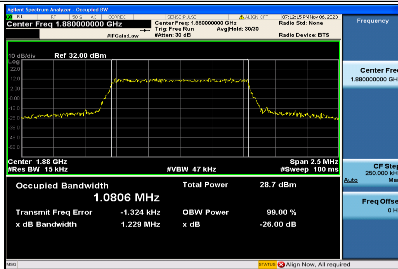
Band2-1.4MHz-16QAM-18900-6RB#0-1.0806
