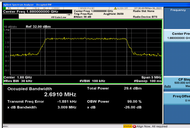
Band2-3MHz-16QAM-18900-15RB#0-2.6910
