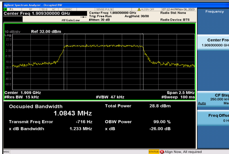
Band2-1.4MHz-16QAM-19193-6RB#0-1.0843
