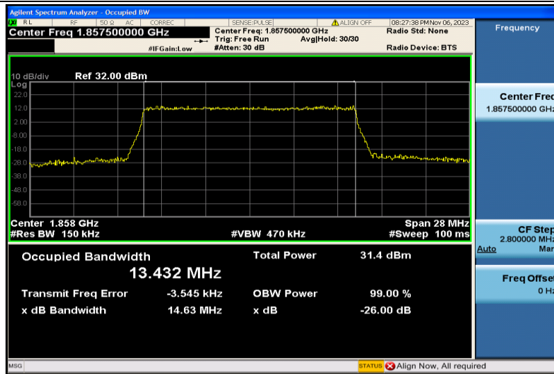
Band2-15MHz-16QAM-18675-75RB#0-13.432
