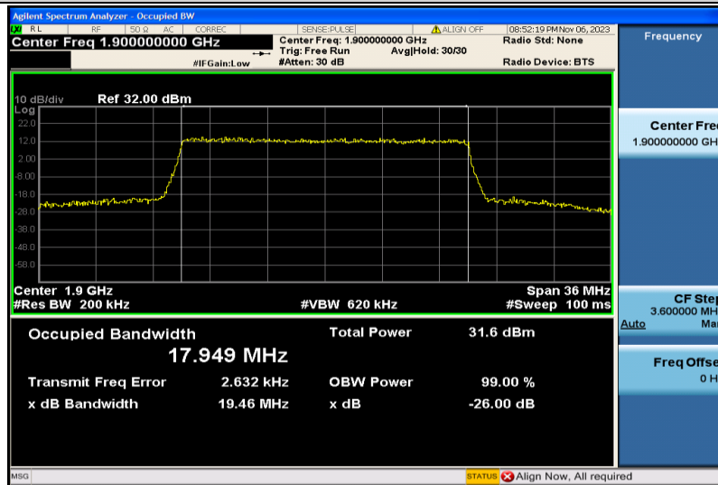
Band2-20MHz-16QAM-19100-100RB#0-17.949
