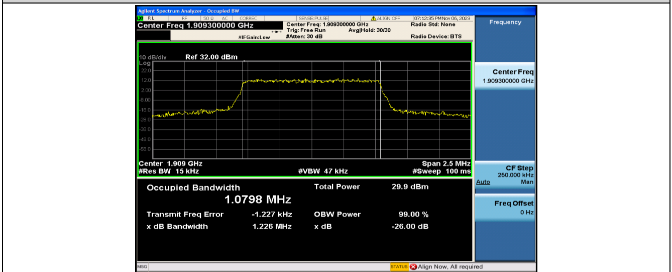
Band2-1.4MHz-QPSK-19193-6RB#0-1.0798
