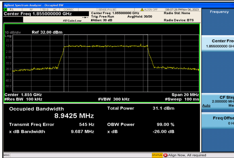
Band2-10MHz-16QAM-18650-50RB#0-8.9425
