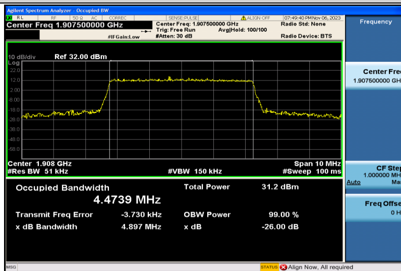
Band2-5MHz-16QAM-19175-25RB#0-4.4739
