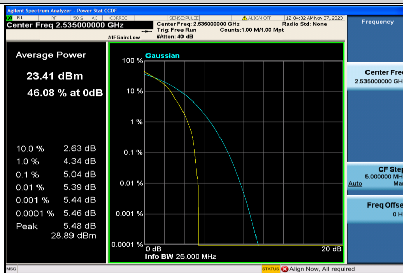
Band7-5MHz-QPSK-21100-1RB#0
