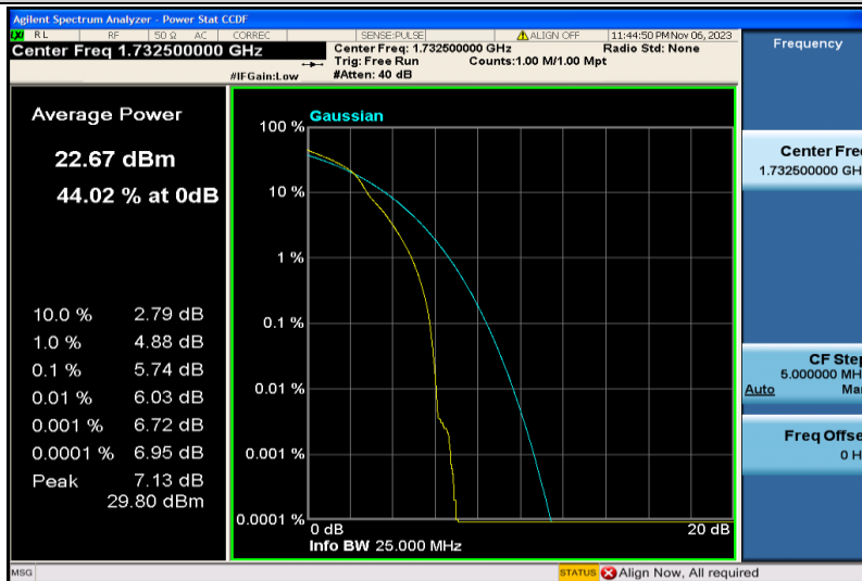
Band4-20MHz-16QAM-20175-1RB#0
