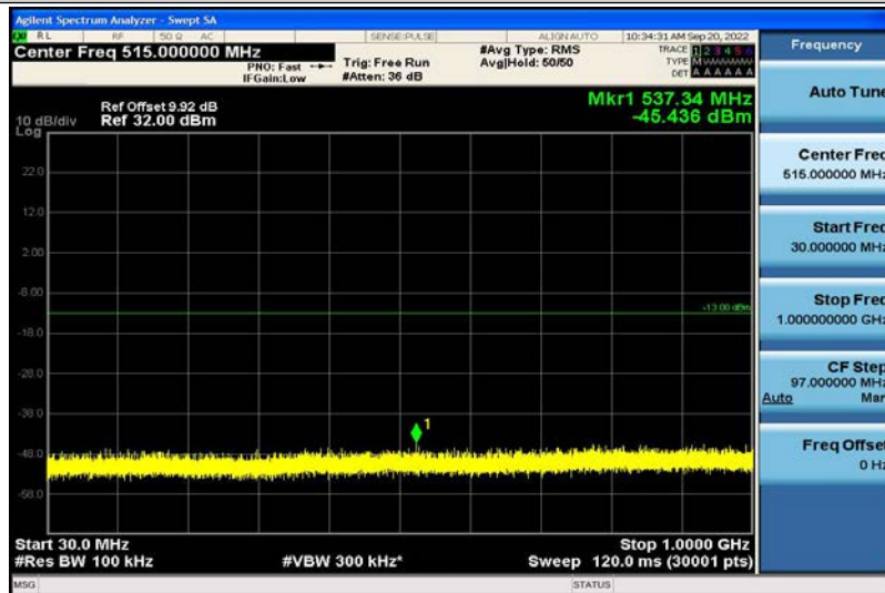
Band2-1.4MHz-16QAM-Run-18900-1RB#0-30~1000MHz
