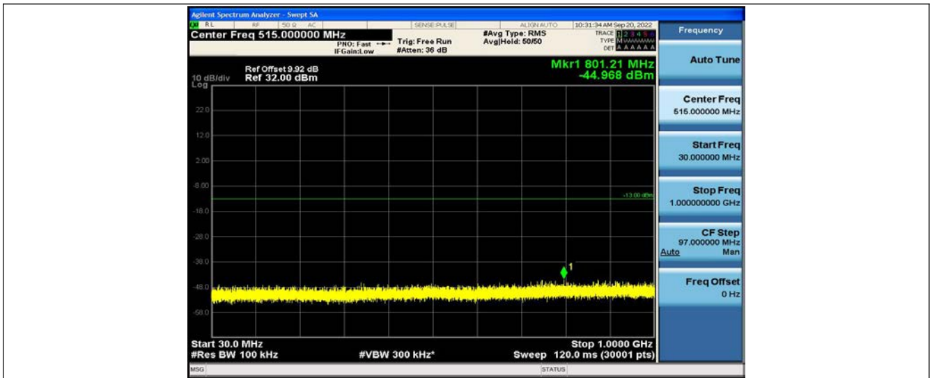
Band2-1.4MHz-QPSK-18607-1RB#0-30~1000MHz
