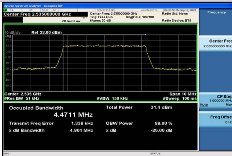
Band7-5MHz-QPSK-21100-25RB#0-4.4711
