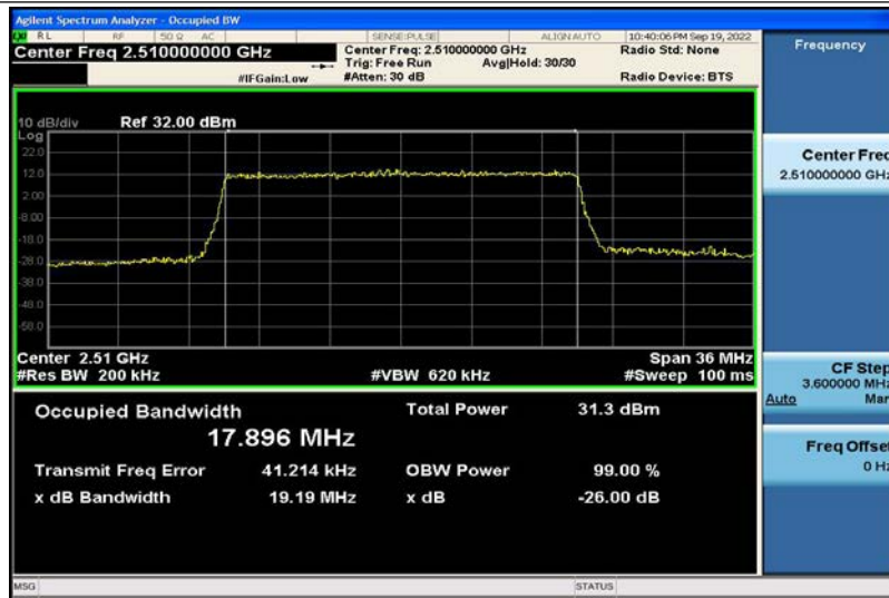
Band7-20MHz-16QAM-20850-100RB#0-17.896
