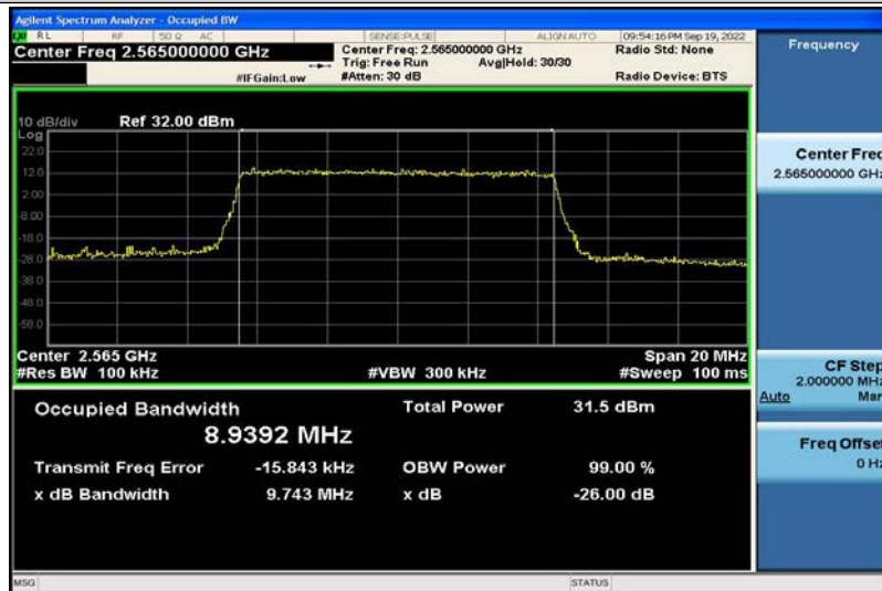
Band7-10MHz-QPSK-21400-50RB#0-8.9392
