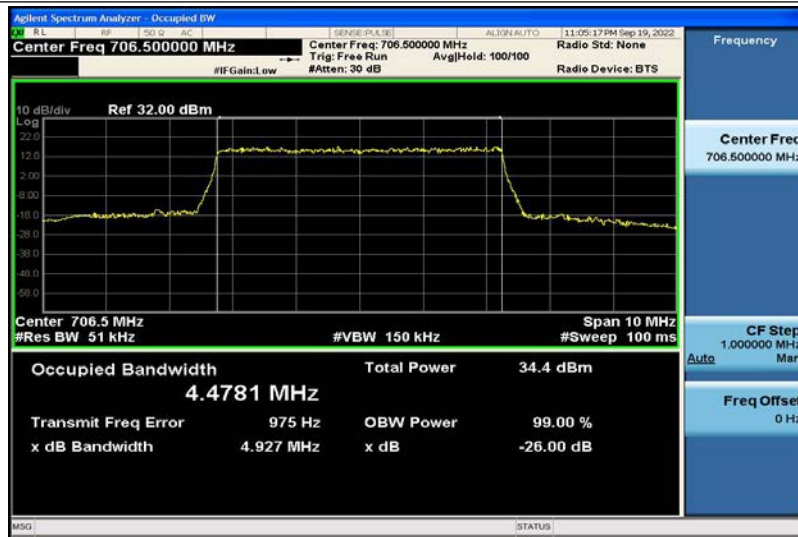
Band17-5MHz-QPSK-23755-25RB#0-4.4781
