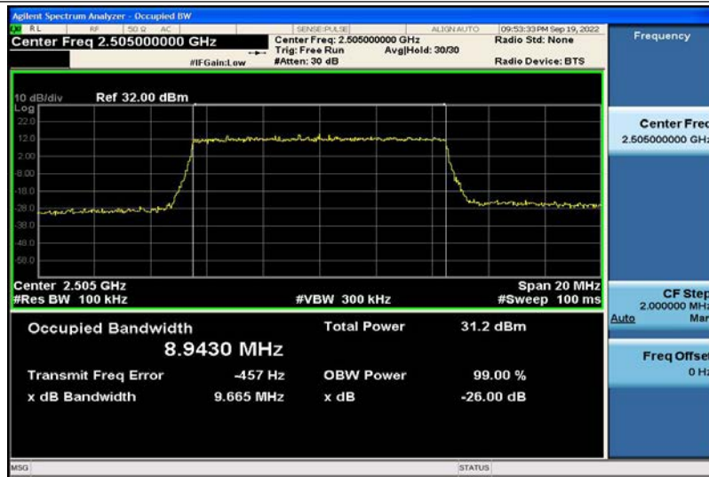
Band7-10MHz-QPSK-20800-50RB#0-8.9430
