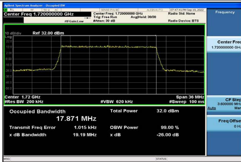
Band4-20MHz-16QAM-20050-100RB#0-17.871
