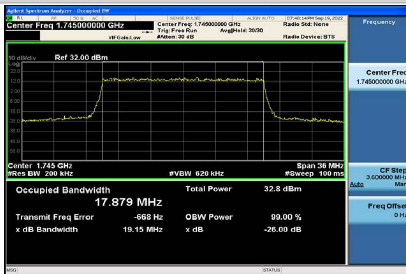
Band4-20MHz-QPSK-20300-100RB#0-17.879
