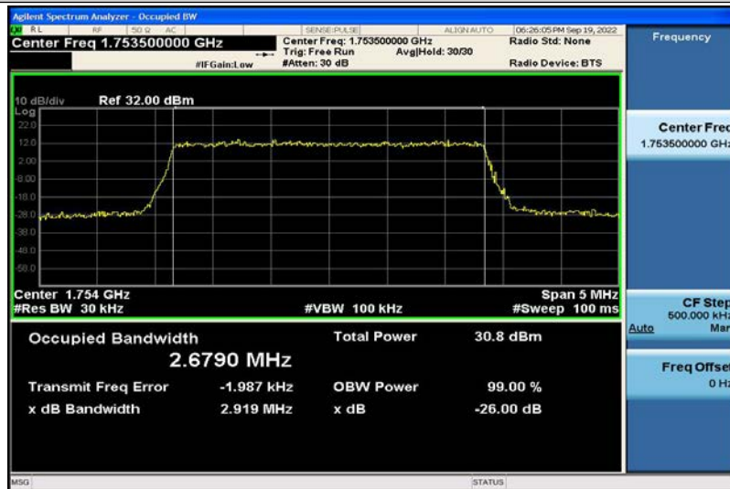
Band4-3MHz-16QAM-20385-15RB#0-2.6790
