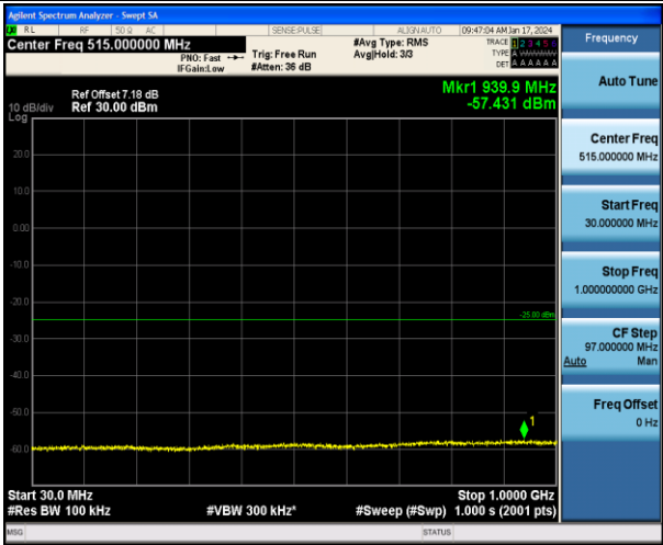
Band7_20MHz_QPSK_20850_1RB#0_30~1000_30~1000
