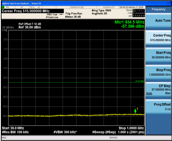
Band7_20MHz_QPSK_21350_1RB#0_30~1000_30~1000
