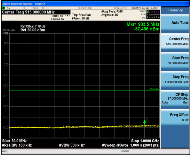
Band7_10MHz_16QAM_20800_1RB#0_30~1000_30~1000
