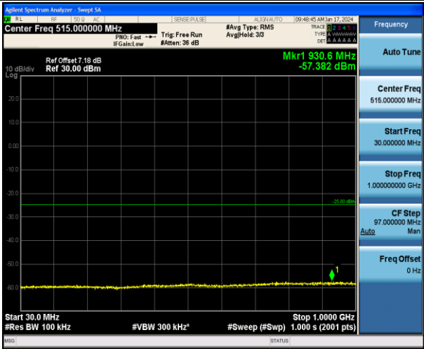
Band7_20MHz_16QAM_21100_1RB#0_30~1000_30~1000
