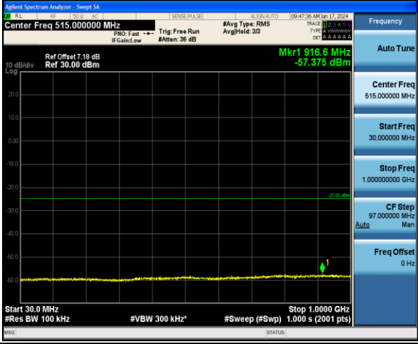
Band7_20MHz_16QAM_20850_1RB#0_30~1000_30~1000
