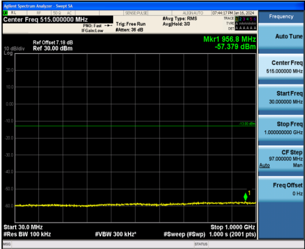
Band2_15MHz_QPSK_19125_1RB#0_30~1000_30~1000
