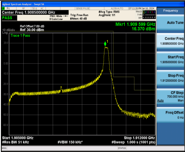
Band2_5MHz_QPSK_19175_1RB#24
