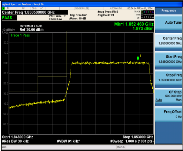
Band2_3MHz_16QAM_18615_15RB#0
