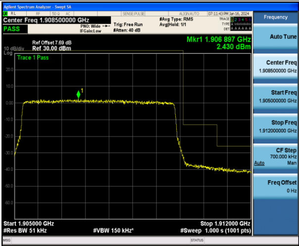
Band2_5MHz_QPSK_19175_25RB#0
