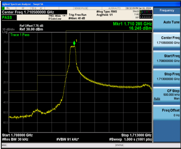
Band4_3MHz_QPSK_19965_1RB#0
