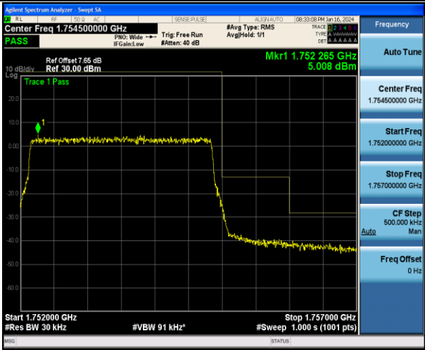
Band4_3MHz_QPSK_20385_15RB#0
