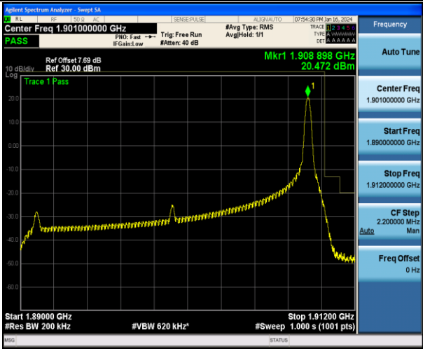
Band2_20MHz_QPSK_19100_1RB#99
