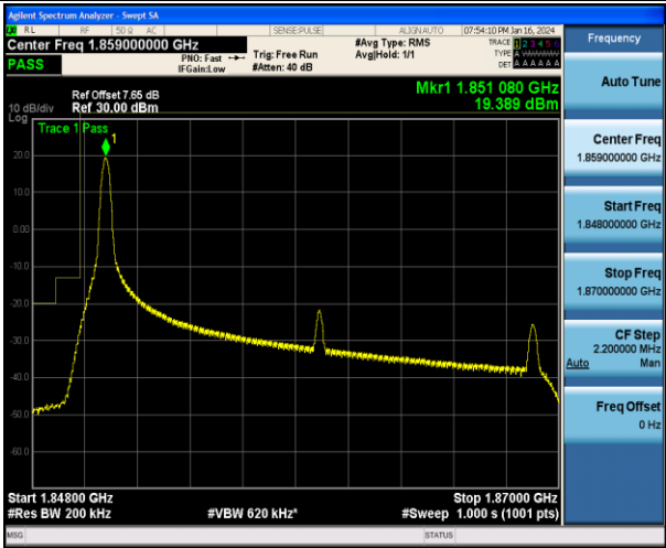
Band2_20MHz_16QAM_18700_1RB#0
