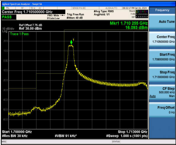
Band4_3MHz_16QAM_19965_1RB#0
