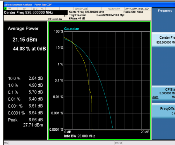
Band5-5MHz-16QAM-20425-1RB#0-PASS
