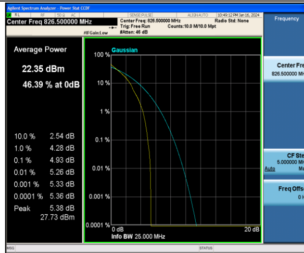
Band5-5MHz-QPSK-20425-1RB#0-PASS
