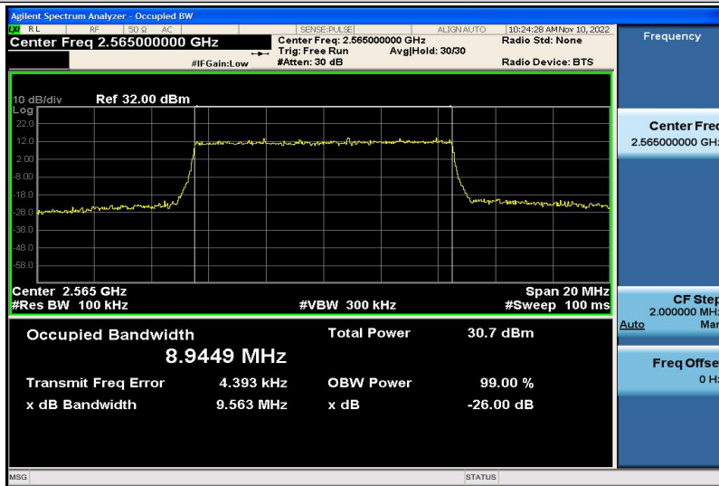
Band7-10MHz-QPSK-21400-50RB#0-8.9449
