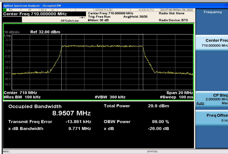
Band17-10MHz-16QAM-23790-50RB#0-8.9507
