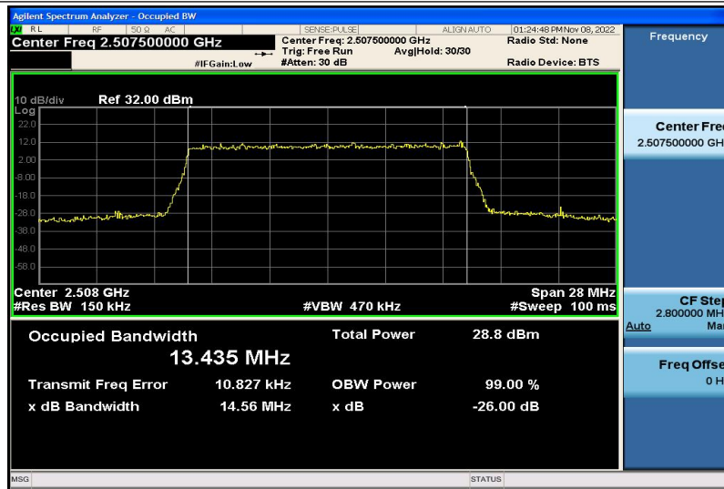
Band7-15MHz-16QAM-20825-75RB#0-13.435
