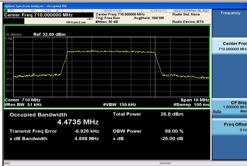
Band17-5MHz-QPSK-23790-25RB#0-4.4735
