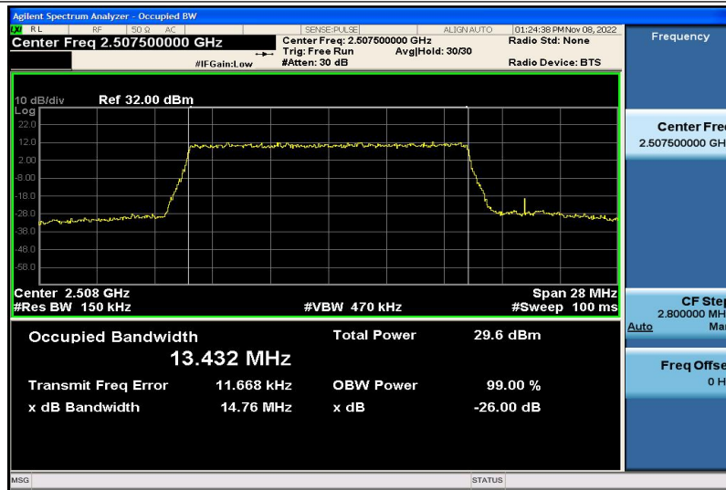
Band7-15MHz-QPSK-20825-75RB#0-13.432
