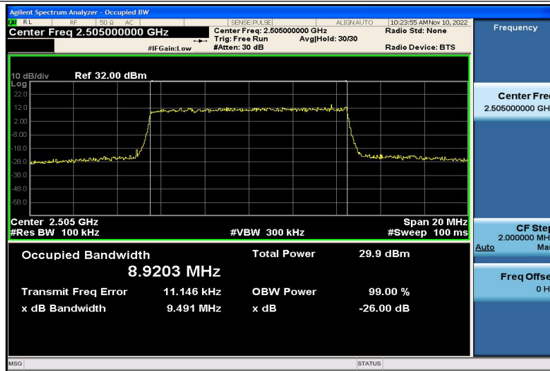
Band7-10MHz-16QAM-20800-50RB#0-8.9203
