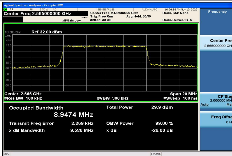
Band7-10MHz-16QAM-21400-50RB#0-8.9474
