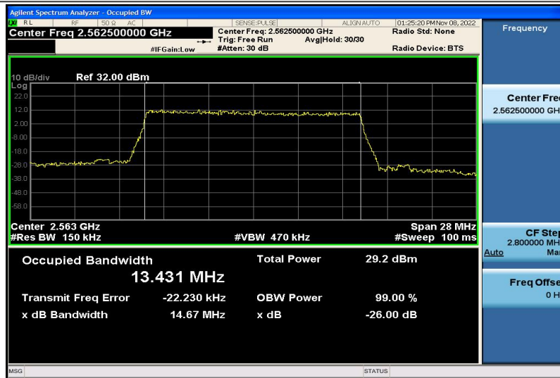
Band7-15MHz-QPSK-21375-75RB#0-13.431
