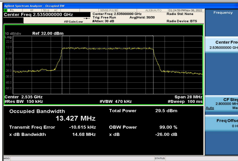
Band7-15MHz-QPSK-21100-75RB#0-13.427
