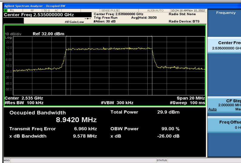
Band7-10MHz-16QAM-21100-50RB#0-8.9420
