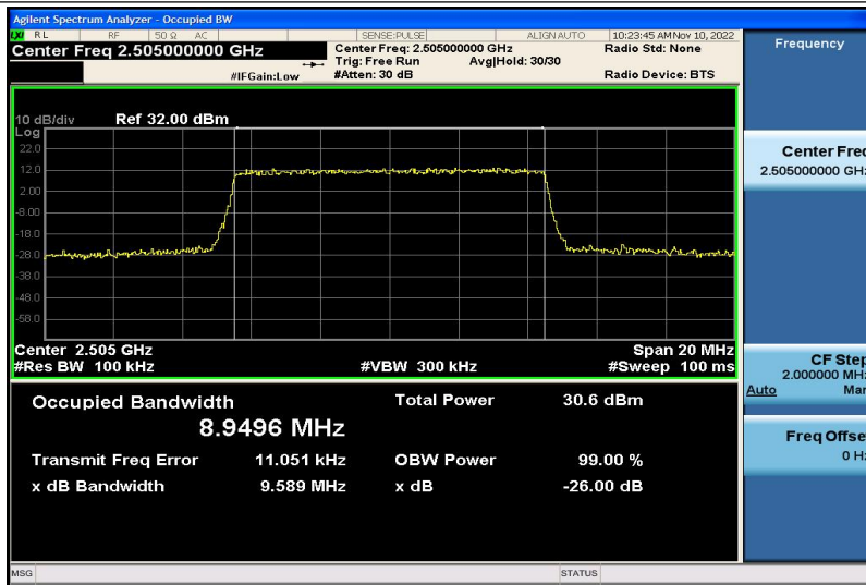
Band7-10MHz-QPSK-20800-50RB#0-8.9496
