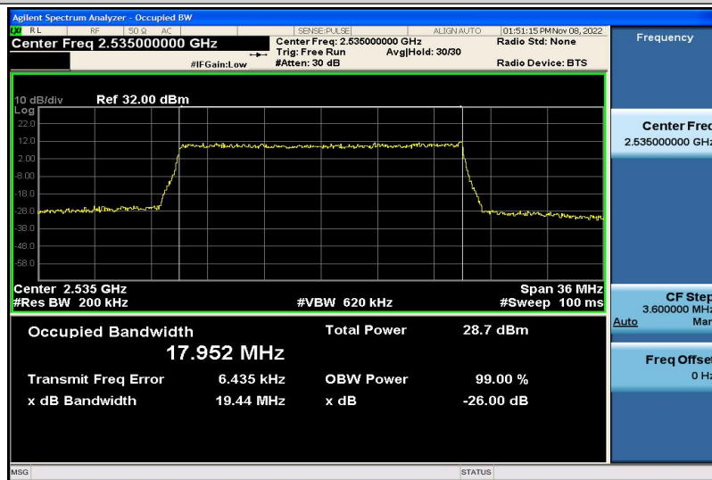
Band7-20MHz-16QAM-21100-100RB#0-17.952
