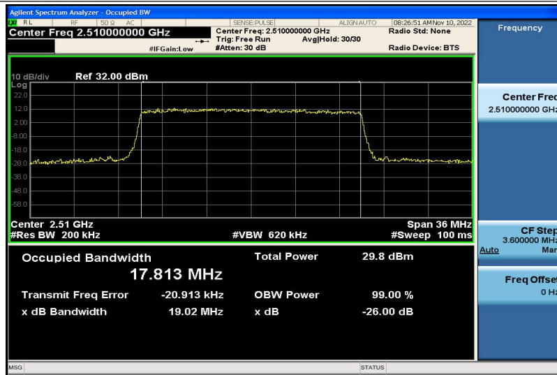
Band7-20MHz-16QAM-20850-100RB#0-17.813
