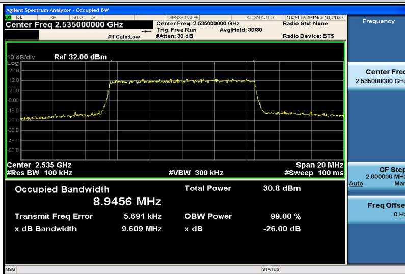
Band7-10MHz-QPSK-21100-50RB#0-8.9456
