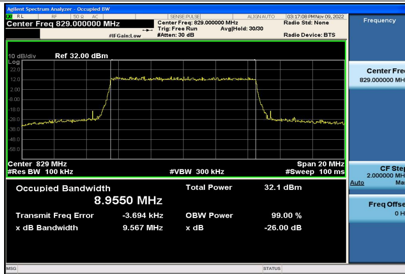
Band5-10MHz-QPSK-20450-50RB#0-8.9550
