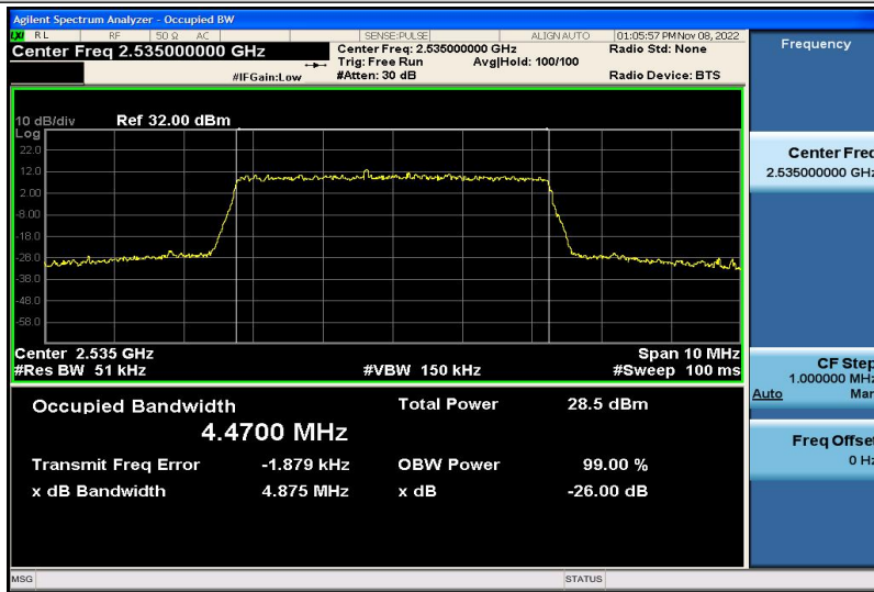
Band7-5MHz-16QAM-21100-25RB#0-4.4700
