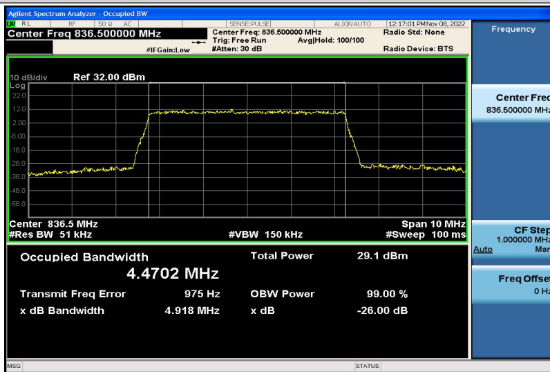
Band5-5MHz-QPSK-20525-25RB#0-4.4702
