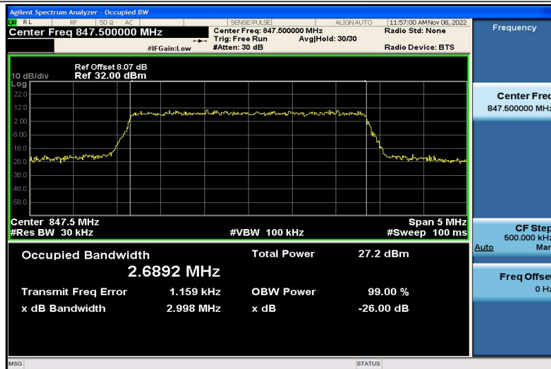
Band5-3MHz-16QAM-20635-15RB#0-2.6892
