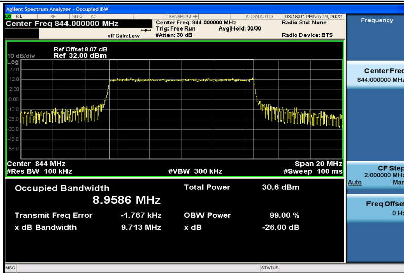
Band5-10MHz-16QAM-20600-50RB#0-8.9586
