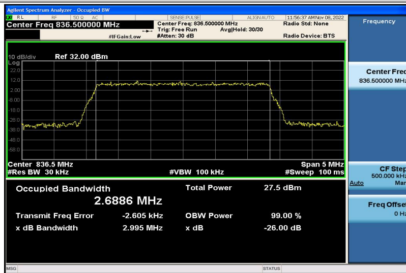
Band5-3MHz-16QAM-20525-15RB#0-2.6886
