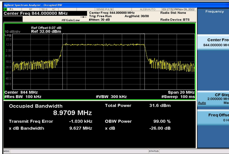
Band5-10MHz-QPSK-20600-50RB#0-8.9709
