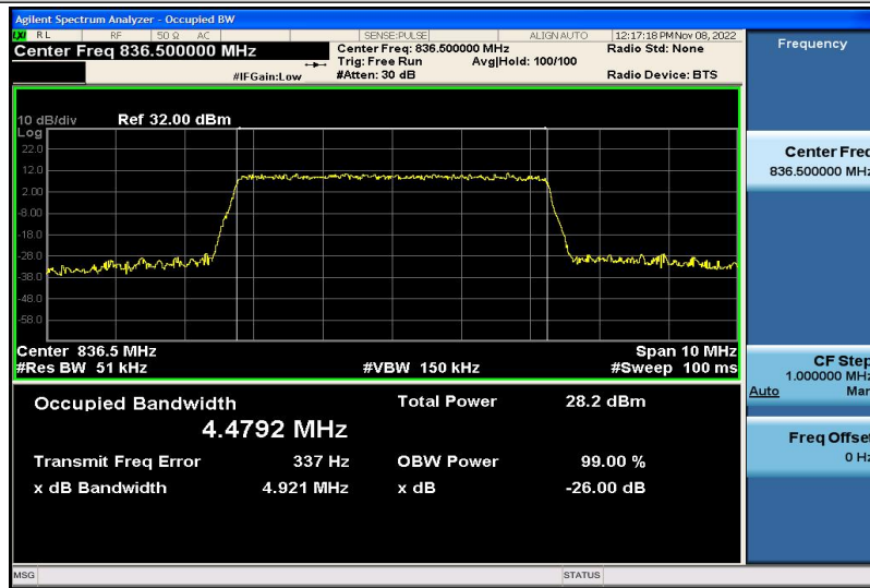
Band5-5MHz-16QAM-20525-25RB#0-4.4792
