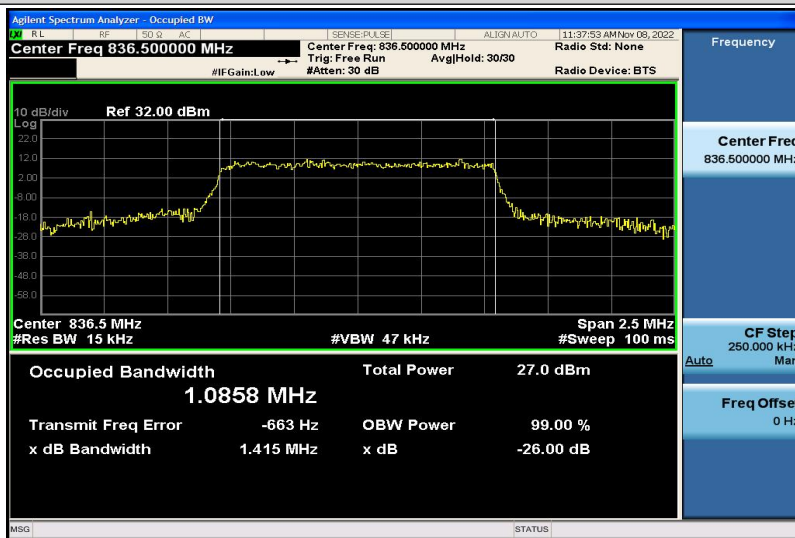
Band5-1.4MHz-16QAM-20525-6RB#0-1.0858
