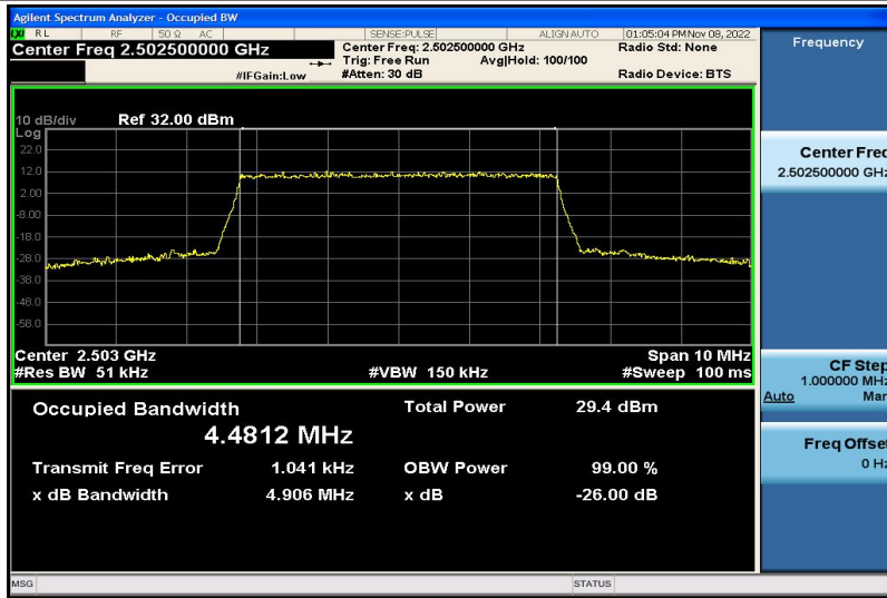
Band7-5MHz-QPSK-20775-25RB#0-4.4812
