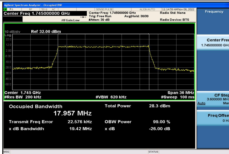
Band4-20MHz-16QAM-20300-100RB#0-17.957
