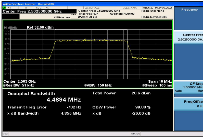
Band7-5MHz-16QAM-20775-25RB#0-4.4694
