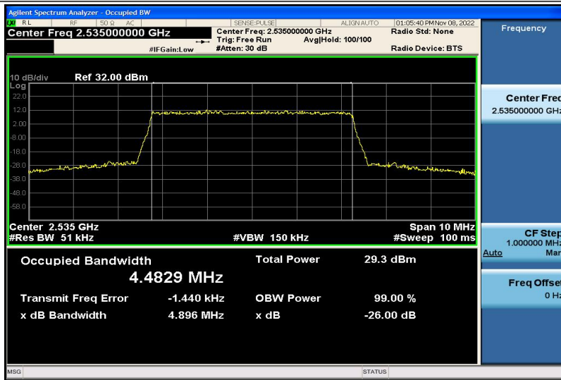
Band7-5MHz-QPSK-21100-25RB#0-4.4829
