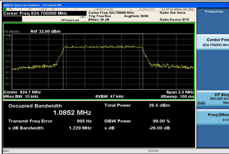
Band5-1.4MHz-16QAM-20407-6RB#0-1.0852
