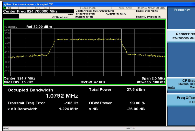
Band5-1.4MHz-QPSK-20407-6RB#0-1.0792
