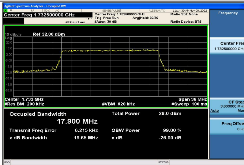
Band4-20MHz-16QAM-20175-100RB#0-17.900
