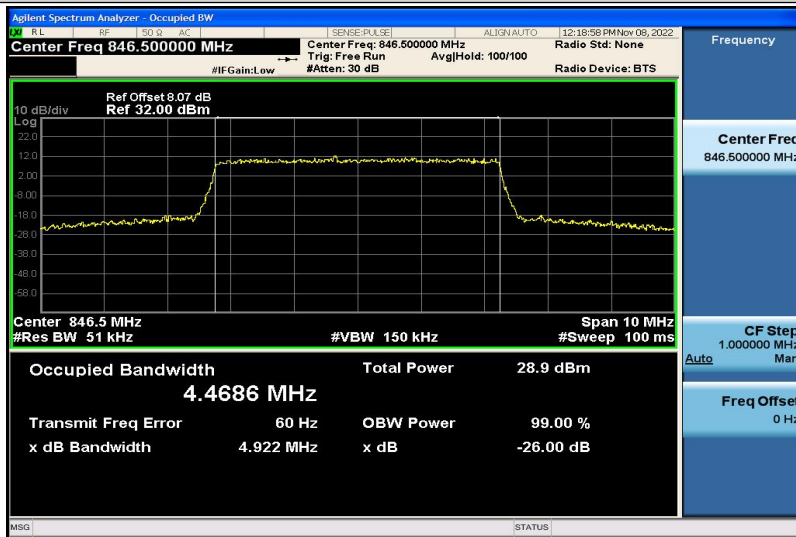
Band5-5MHz-QPSK-20625-25RB#0-4.4686
