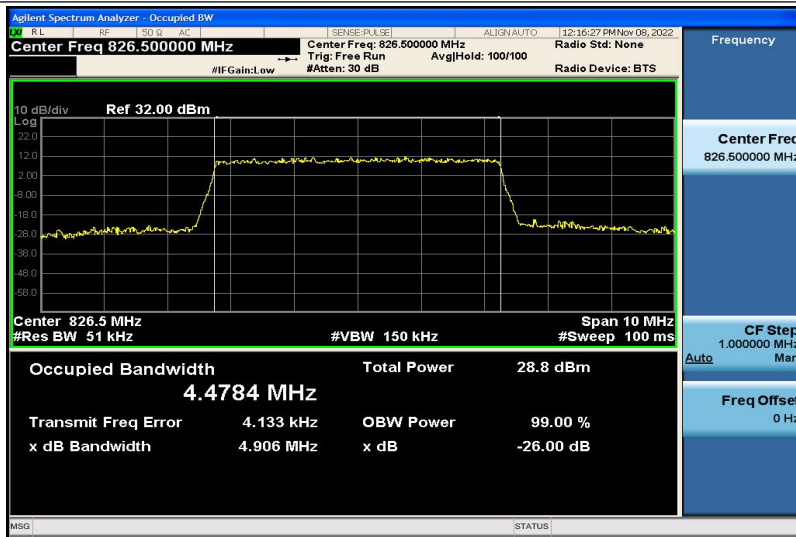
Band5-5MHz-QPSK-20425-25RB#0-4.4784
