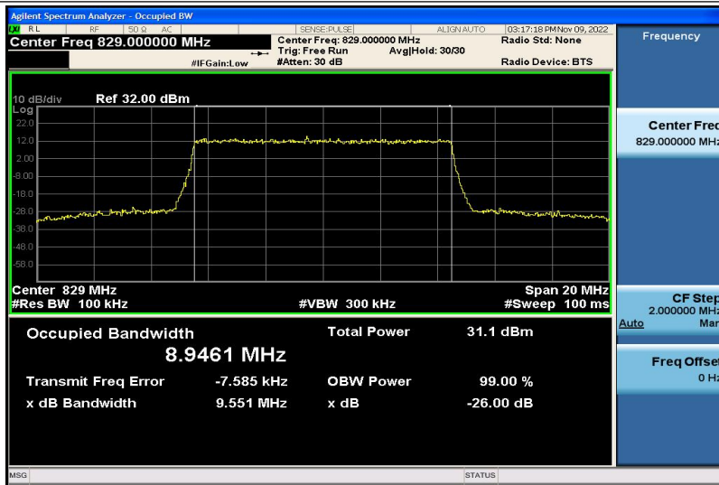
Band5-10MHz-16QAM-20450-50RB#0-8.9461
