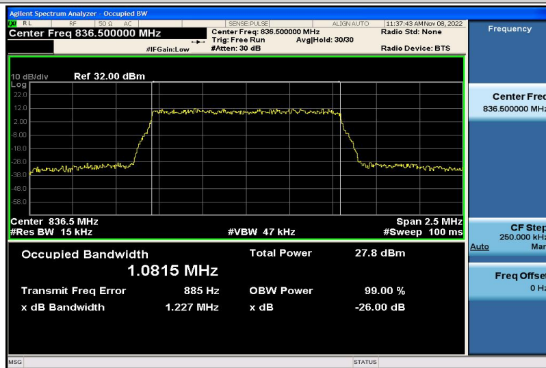
Band5-1.4MHz-QPSK-20525-6RB#0-1.0815
