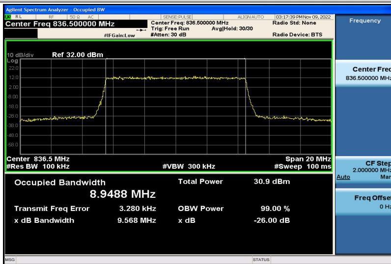
Band5-10MHz-16QAM-20525-50RB#0-8.9488
