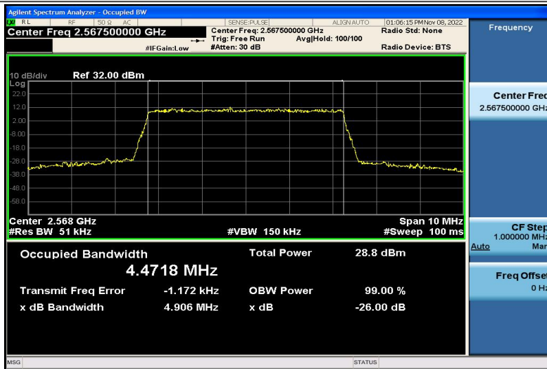
Band7-5MHz-QPSK-21425-25RB#0-4.4718
