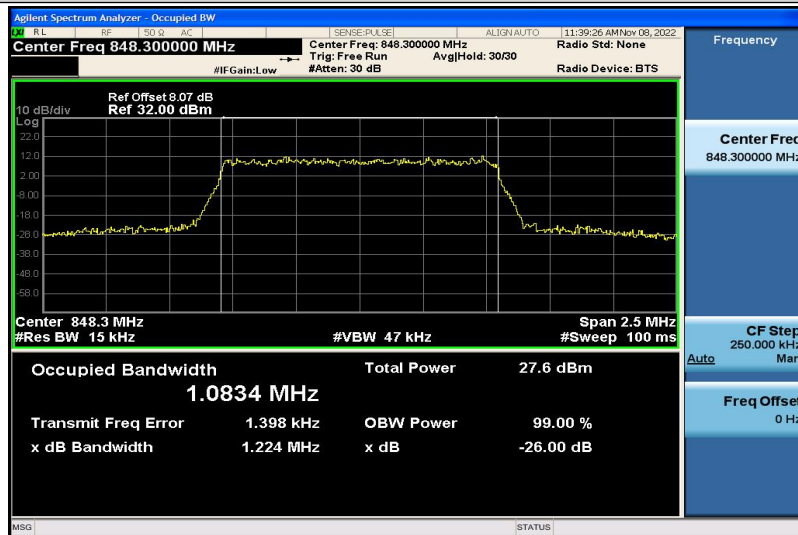
Band5-1.4MHz-QPSK-20643-6RB#0-1.0834
