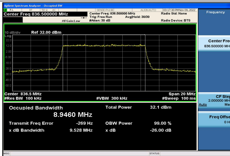
Band5-10MHz-QPSK-20525-50RB#0-8.9460
