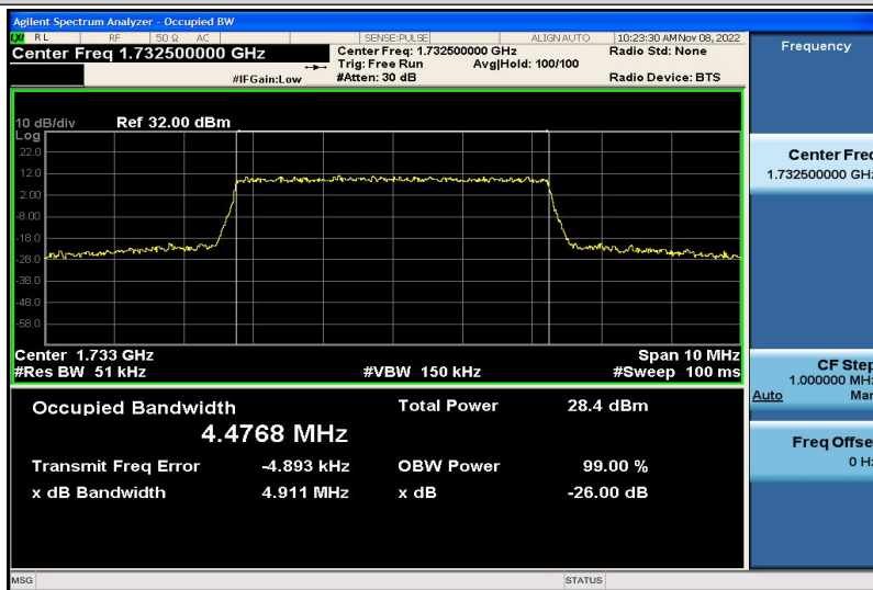
Band4-5MHz-QPSK-17325-25RB#0-4.4768
