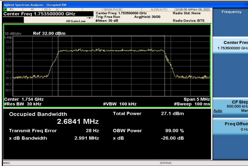
Band4-3MHz-16QAM-20385-15RB#0-2.6841
