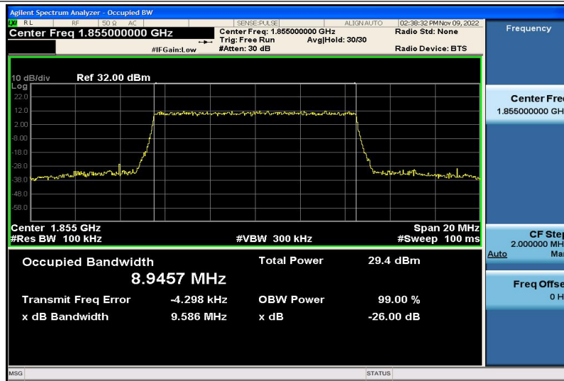
Band2-10MHz-16QAM-18650-50RB#0-8.9457
