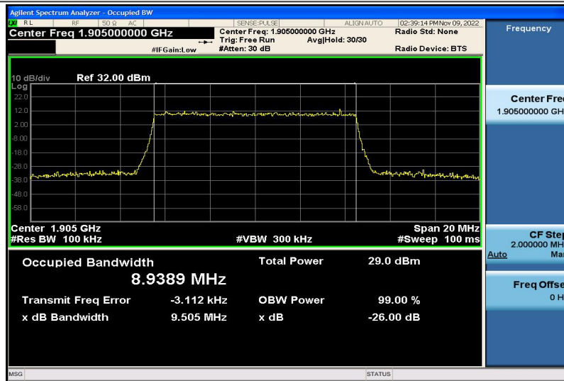
Band2-10MHz-16QAM-19150-50RB#0-8.9389
