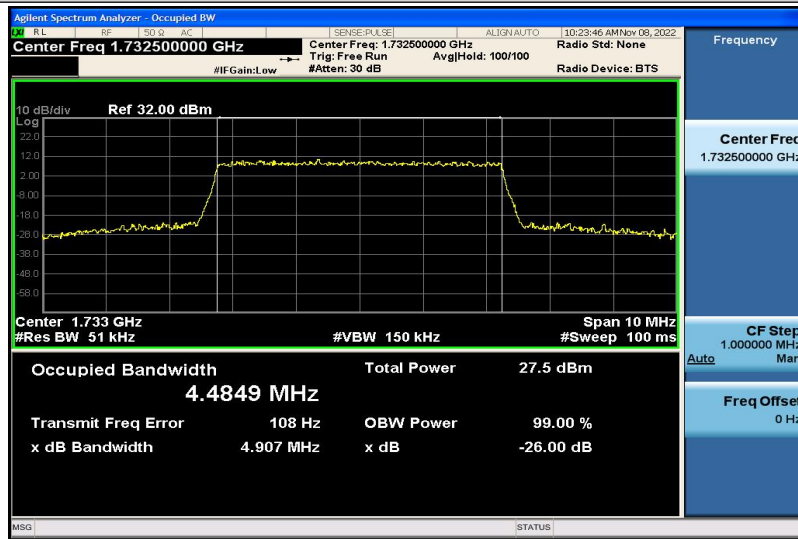
Band4-5MHz-16QAM-20175-25RB#0-4.4849
