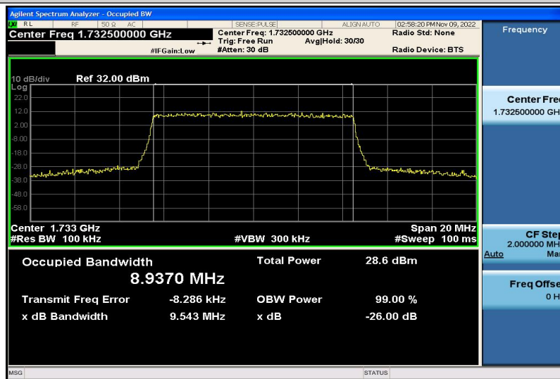
Band4-10MHz-16QAM-20175-50RB#0-8.9370
