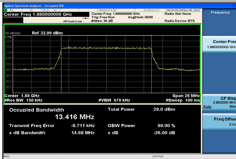
Band2-15MHz-QPSK-18900-75RB#0-13.416
