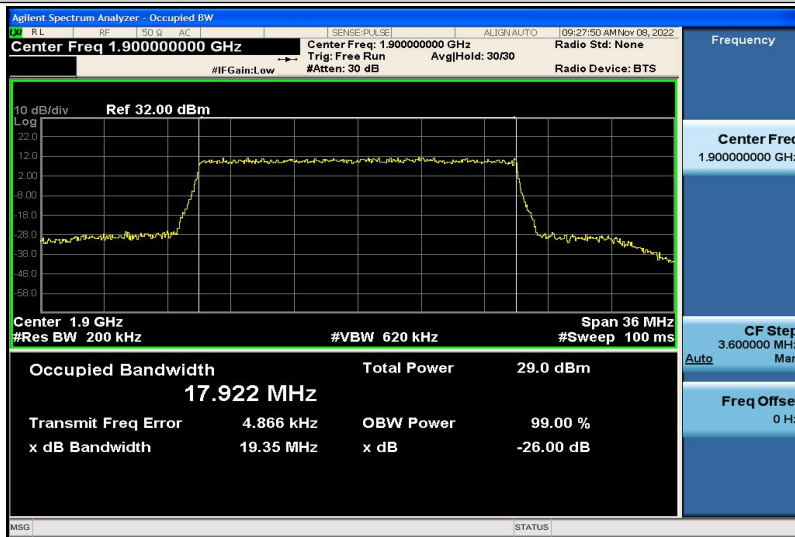
Band2-20MHz-16QAM-19100-100RB#0-17.922
