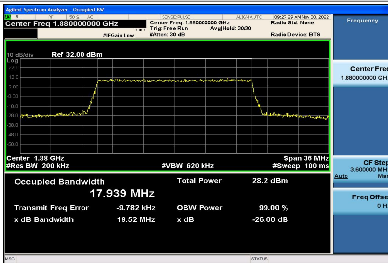
Band2-20MHz-16QAM-18900-100RB#0-17.939
