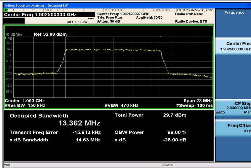
Band2-15MHz-QPSK-19125-75RB#0-13.362
