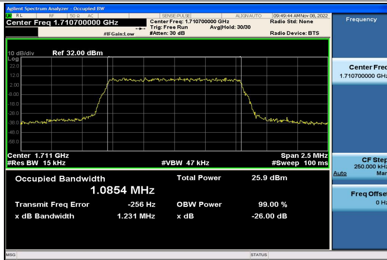
Band4-1.4MHz-16QAM-19957-6RB#0-1.0854
