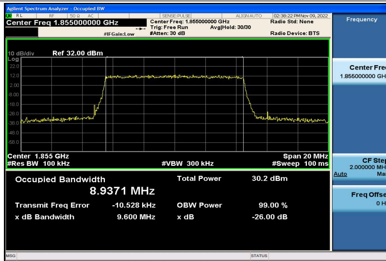
Band2-10MHz-QPSK-18650-50RB#0-8.9371
