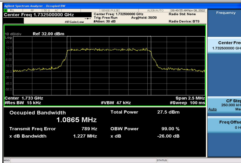
Band4-1.4MHz-QPSK-20175-6RB#0-1.0865
