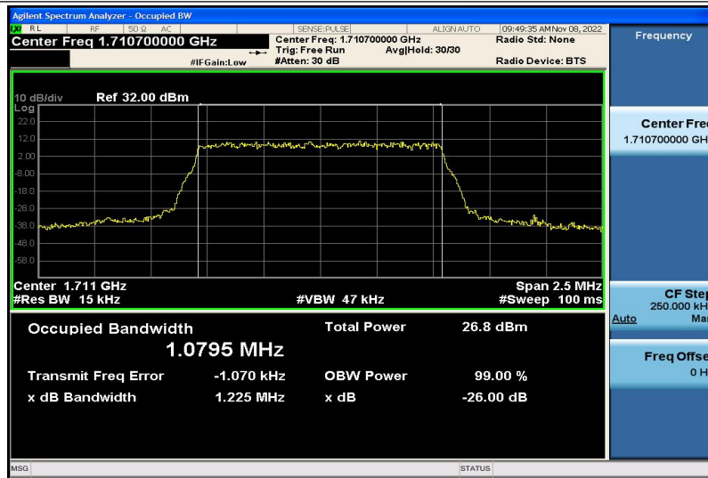
Band4-1.4MHz-QPSK-19957-6RB#0-1.0795
