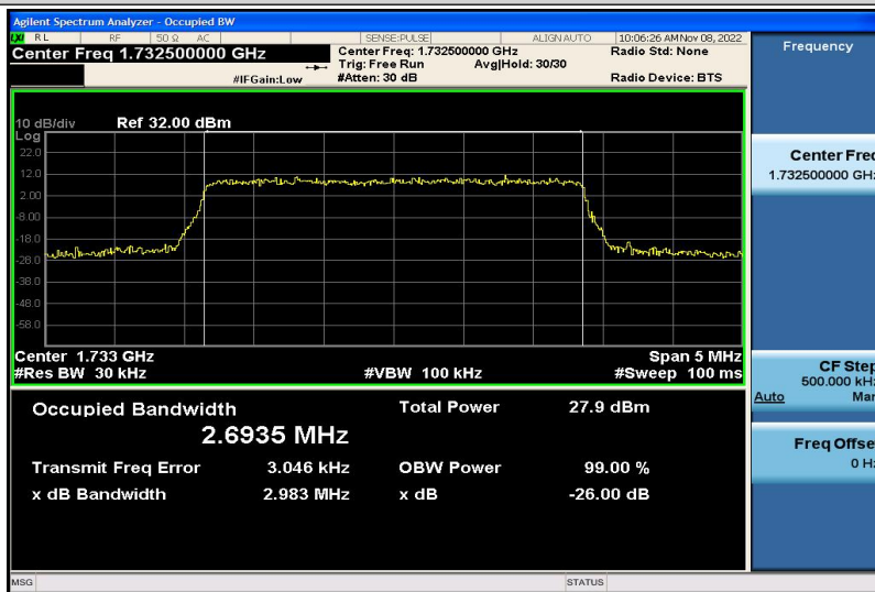
Band4-3MHz-QPSK-20175-15RB#0-2.6935
