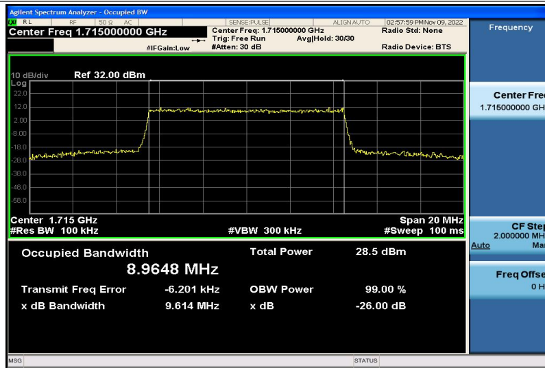
Band4-10MHz-16QAM-20000-50RB#0-8.9648
