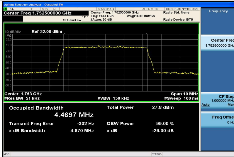
Band4-5MHz-16QAM-20375-25RB#0-4.4697
