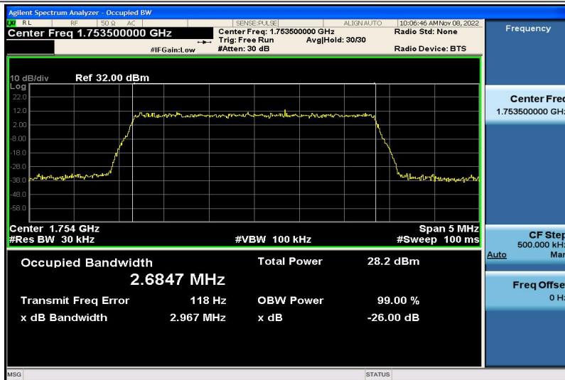
Band4-3MHz-QPSK-20385-15RB#0-2.6847
