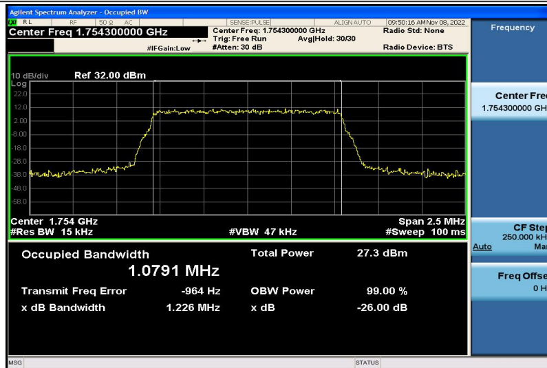
Band4-1.4MHz-QPSK-20393-6RB#0-1.0791
