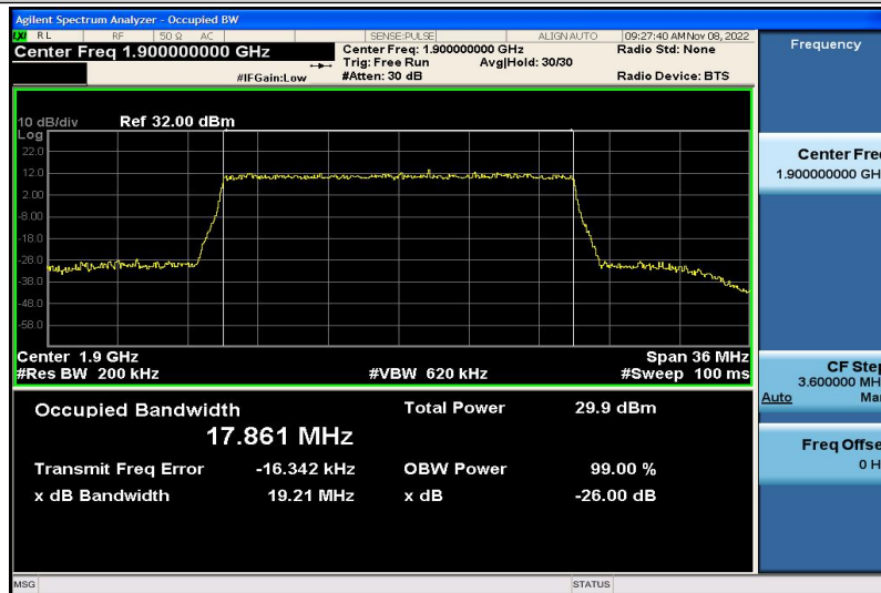
Band2-20MHz-QPSK-19100-100RB#0-17.861
