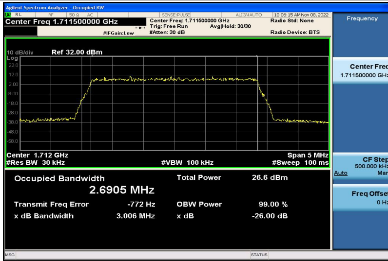
Band4-3MHz-16QAM-19965-15RB#0-2.6905
