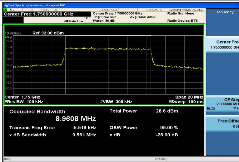
Band4-10MHz-16QAM-20350-50RB#0-8.9608
