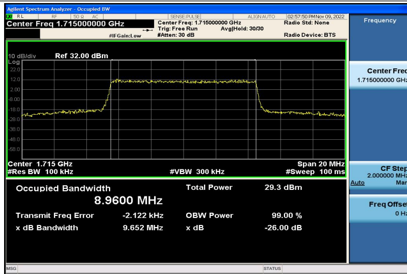
Band4-10MHz-QPSK-20000-50RB#0-8.9600
