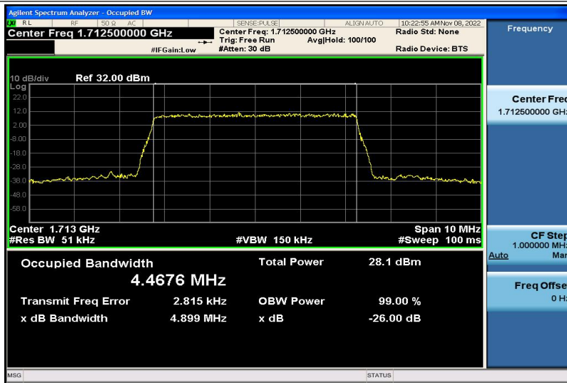
Band4-5MHz-QPSK-19975-25RB#0-4.4676
