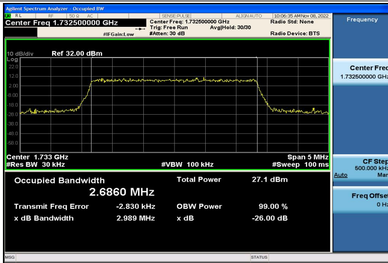
Band4-3MHz-16QAM-20175-15RB#0-2.6860
