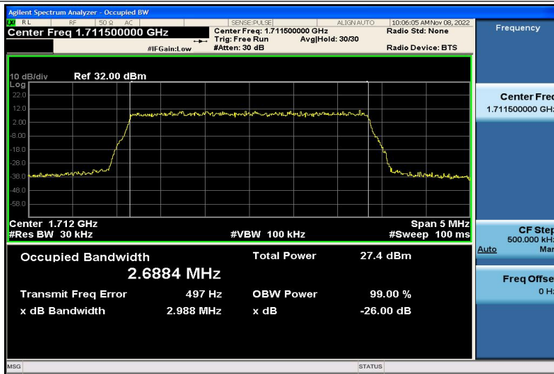
Band4-3MHz-QPSK-19965-15RB#0-2.6884
