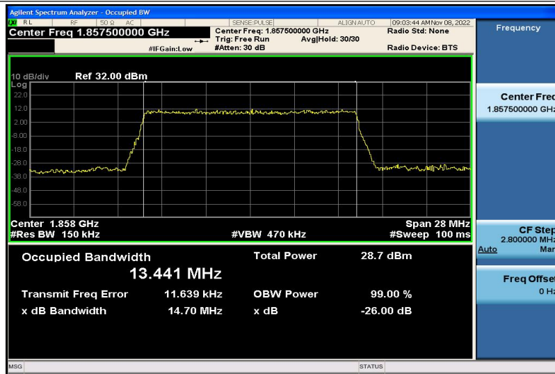
Band2-15MHz-QPSK-18675-75RB#0-13.441
