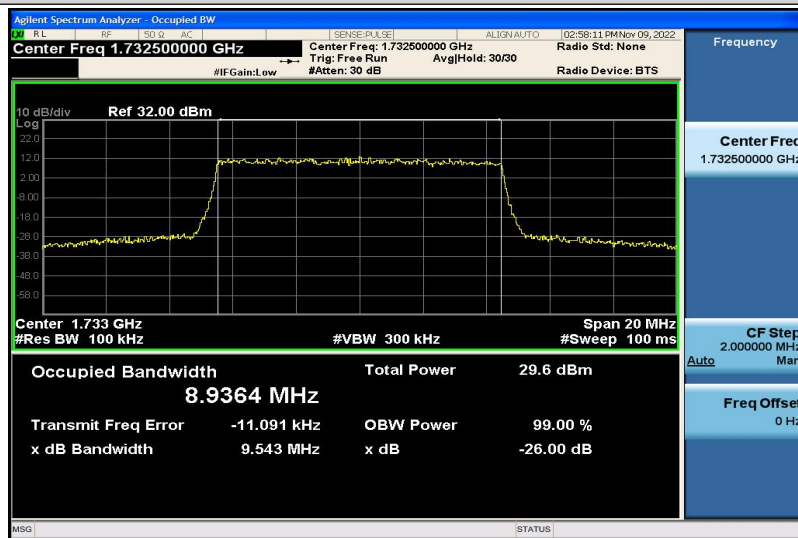
Band4-10MHz-QPSK-20175-50RB#0-8.9364
