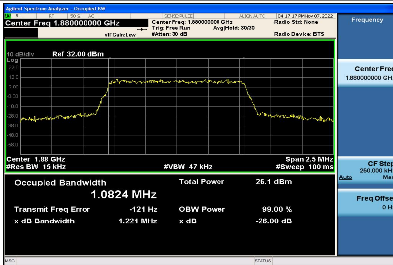
Band2-1.4MHz-16QAM-18900-6RB#0-1.0824
