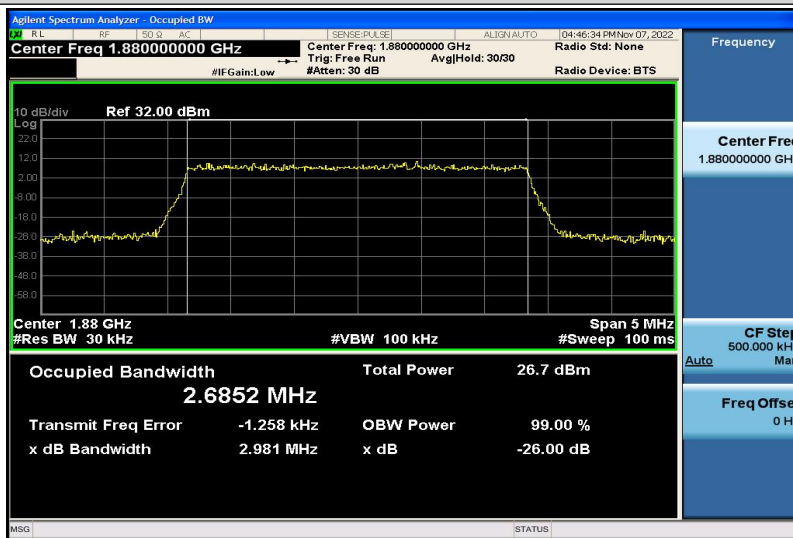
Band2-3MHz-16QAM-18900-15RB#0-2.6852
