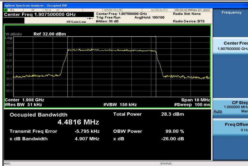
Band2-5MHz-QPSK-19175-25RB#0-4.4816
