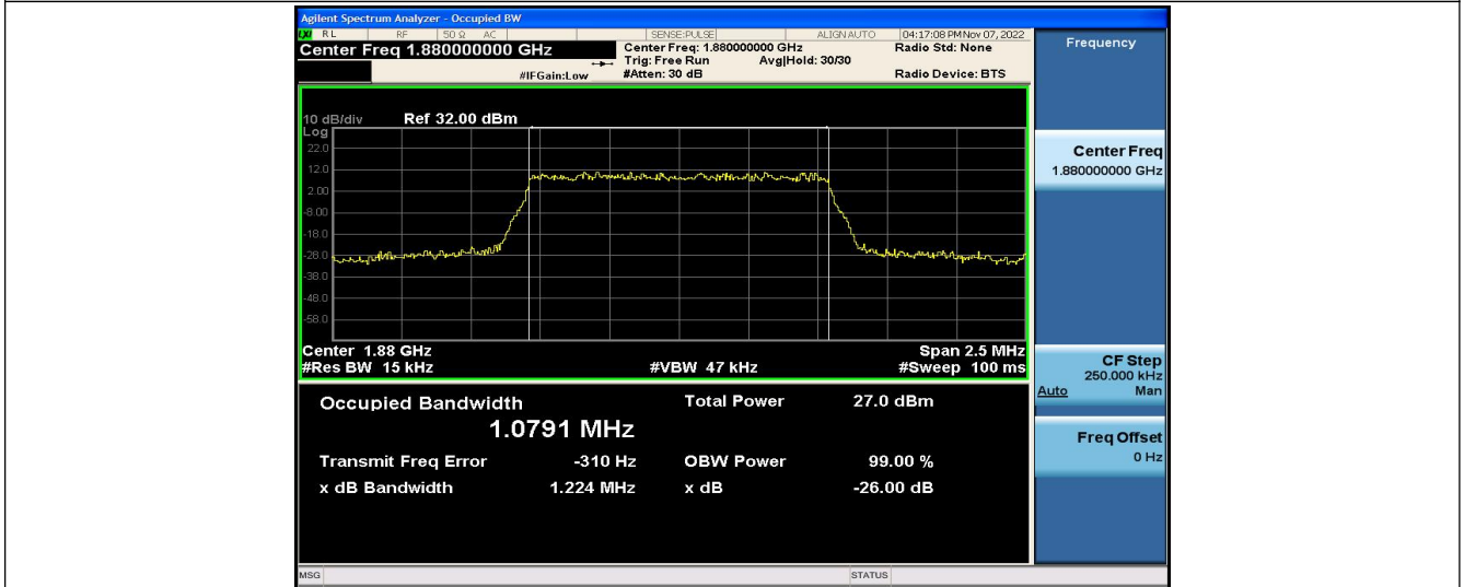
Band2-1.4MHz-QPSK-18900-6RB#0-1.0791
