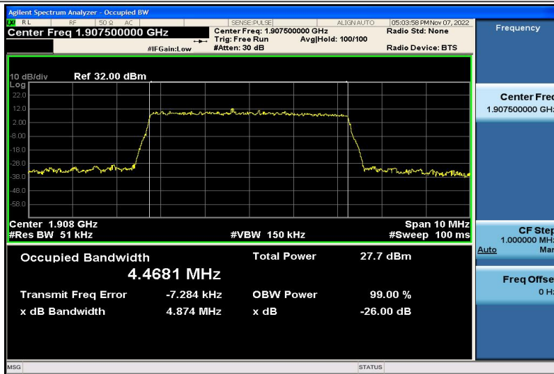
Band2-5MHz-16QAM-19175-25RB#0-4.4681
