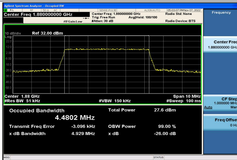
Band2-5MHz-QPSK-18900-25RB#0-4.4802
