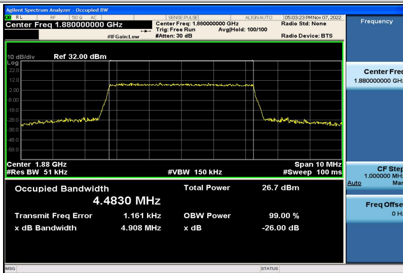
Band2-5MHz-16QAM-18900-25RB#0-4.4830
