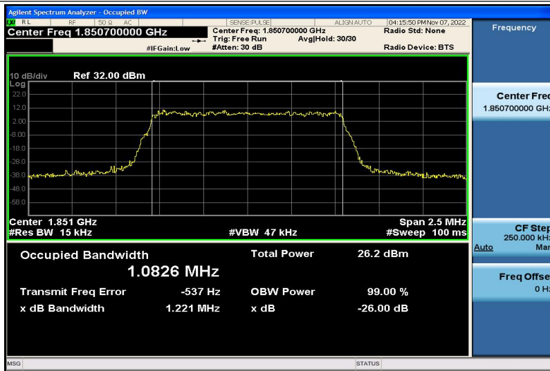
Band2-1.4MHz-16QAM-18607-6RB#0-1.0826
