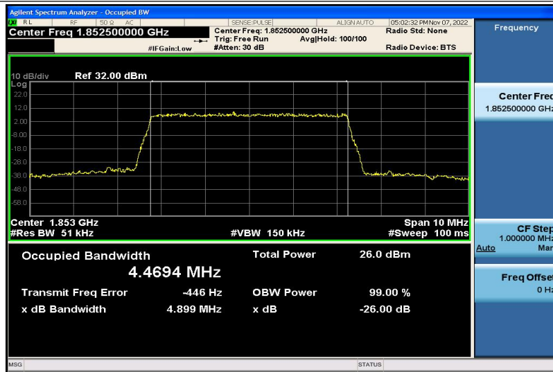
Band2-5MHz-QPSK-18625-25RB#0-4.4694
