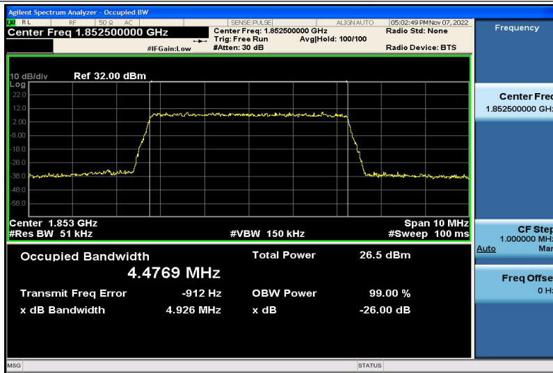
Band2-5MHz-16QAM-18625-25RB#0-4.4769
