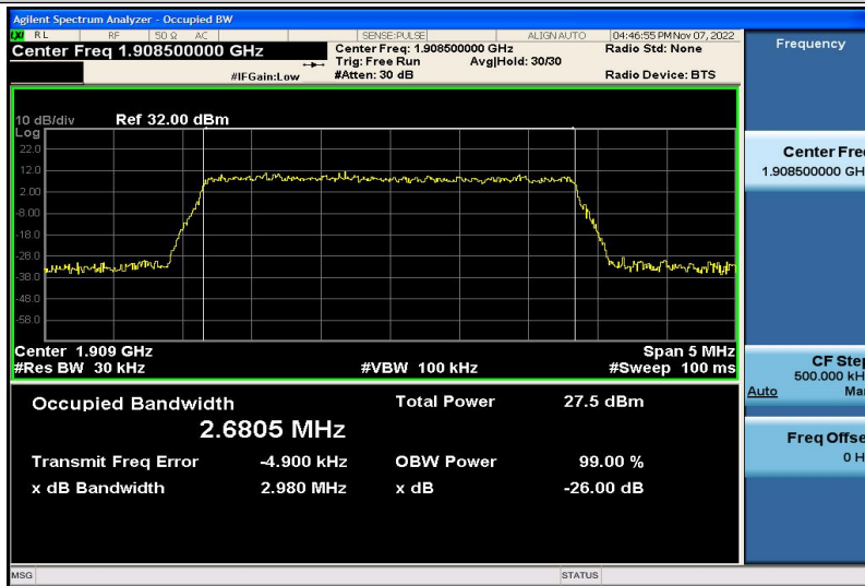
Band2-3MHz-16QAM-19185-15RB#0-2.6805
