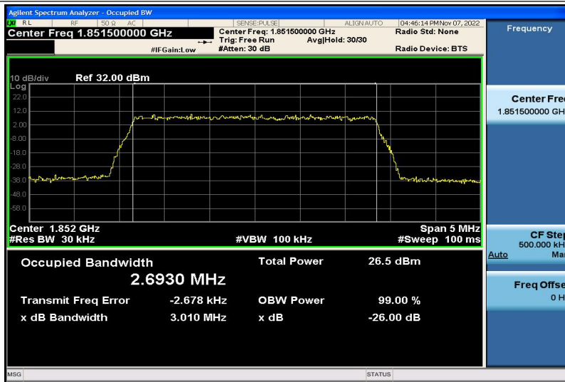
Band2-3MHz-16QAM-18615-15RB#0-2.6930
