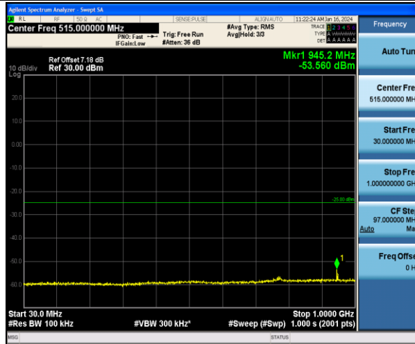
Band7_20MHz_16QAM_20850_1RB#0_30~1000_30~1000
