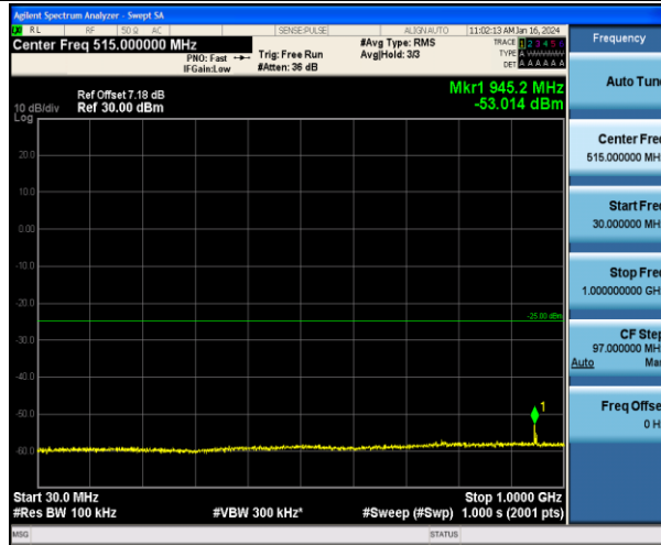
Band7_15MHz_QPSK_21375_1RB#0_30~1000_30~1000
