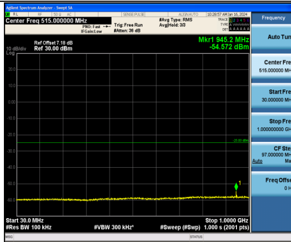
Band7_10MHz_QPSK_21100_1RB#0_30~1000_30~1000
