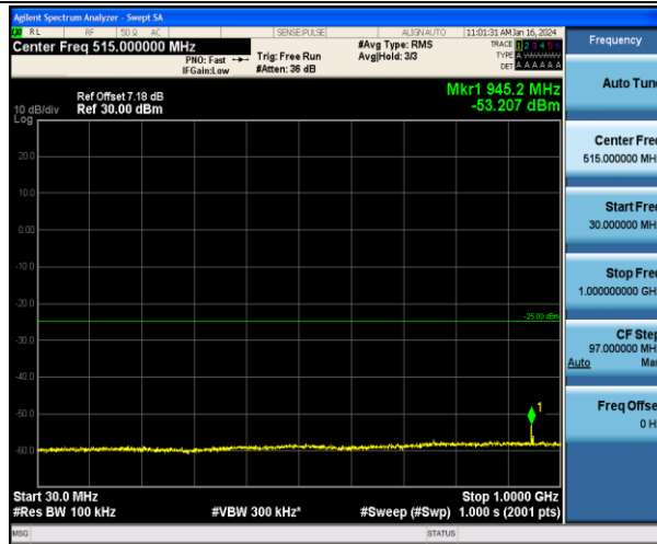
Band7_15MHz_16QAM_21100_1RB#0_30~1000_30~1000
