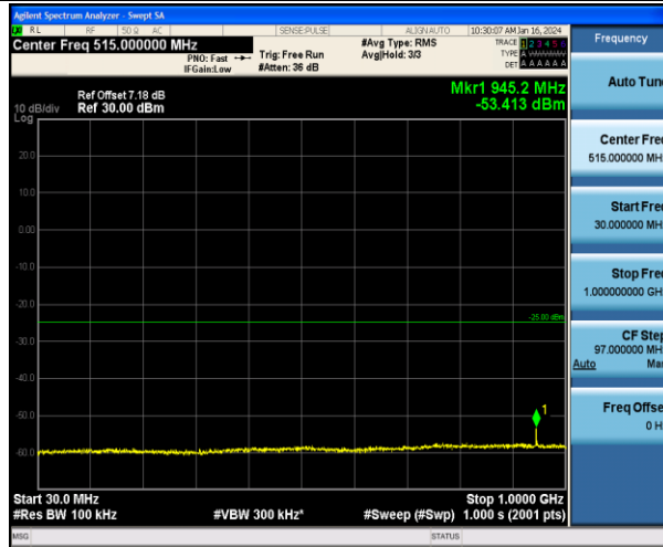
Band7_10MHz_QPSK_21400_1RB#0_30~1000_30~1000
