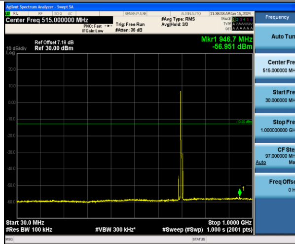
Band17_5MHz_16QAM_23755_1RB#0_30~1000_30~1000
