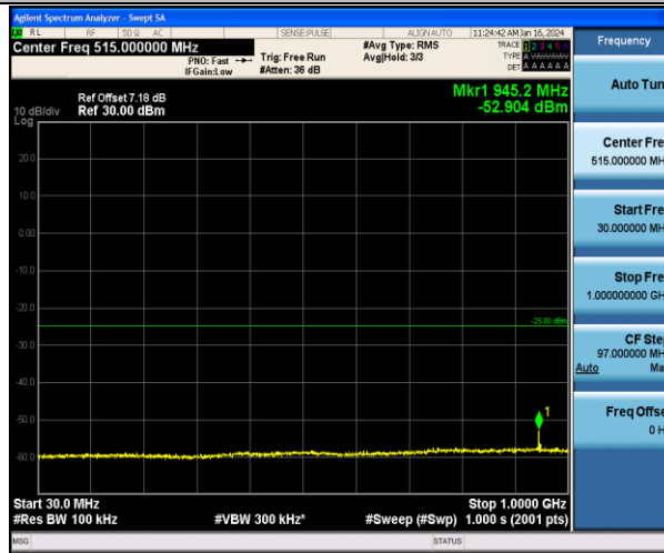
Band7_20MHz_16QAM_21350_1RB#0_30~1000_30~1000
