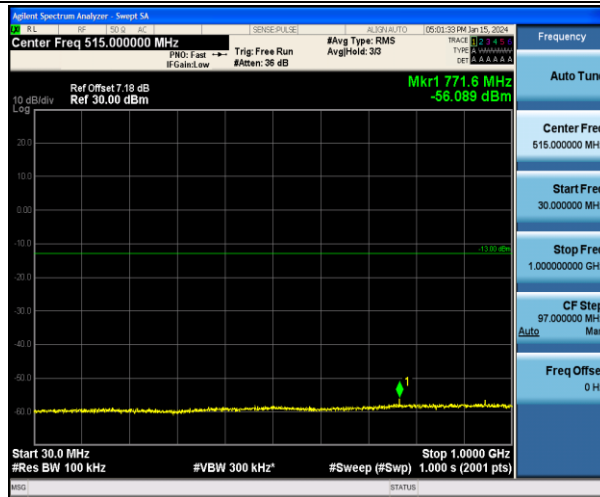
Band4_5MHz_QPSK_19975_1RB#0_30~1000_30~1000
