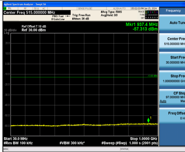
Band4_5MHz_16QAM_19975_1RB#0_30~1000_30~1000
