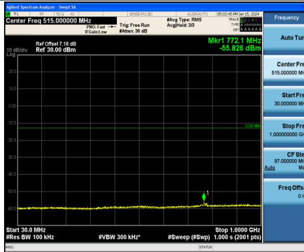
Band4_5MHz_QPSK_20375_1RB#0_30~1000_30~1000
