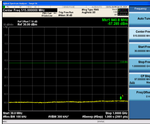
Band2_20MHz_16QAM_18700_1RB#0_30~1000_30~1000
