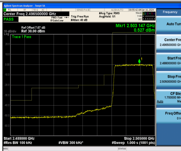
Band7_5MHz_QPSK_20775_25RB#0
