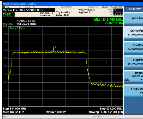
Band5_5MHz_QPSK_20625_25RB#0
