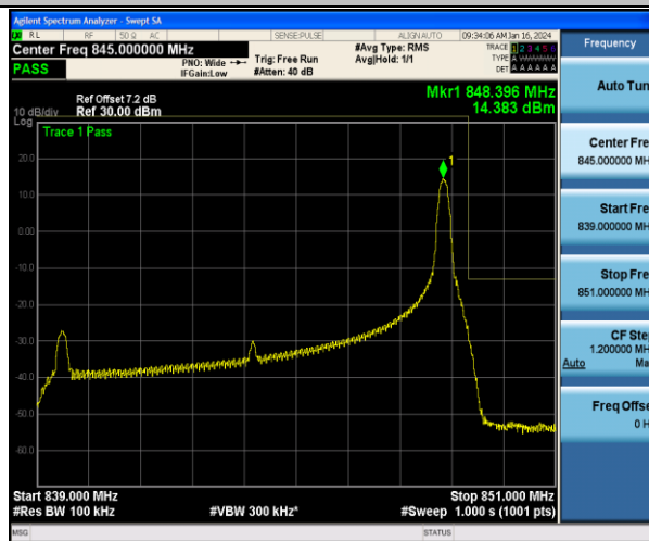
Band5_10MHz_QPSK_20600_1RB#49
