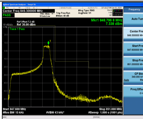
Band5_1.4MHz_16QAM_20643_1RB#5
