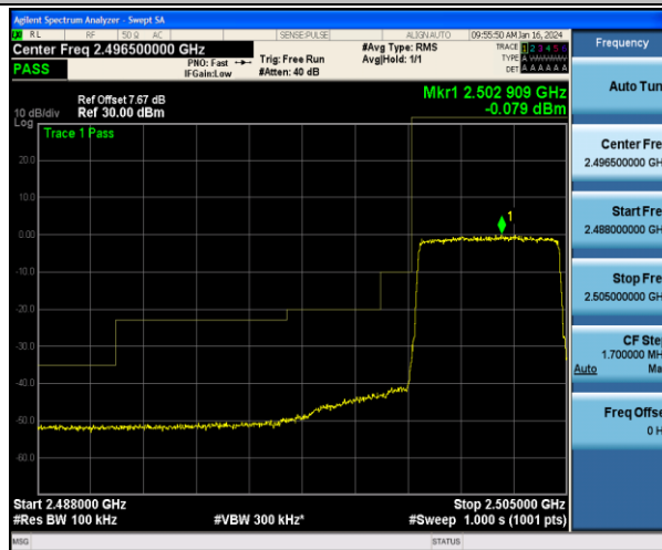
Band7_5MHz_16QAM_20775_25RB#0
