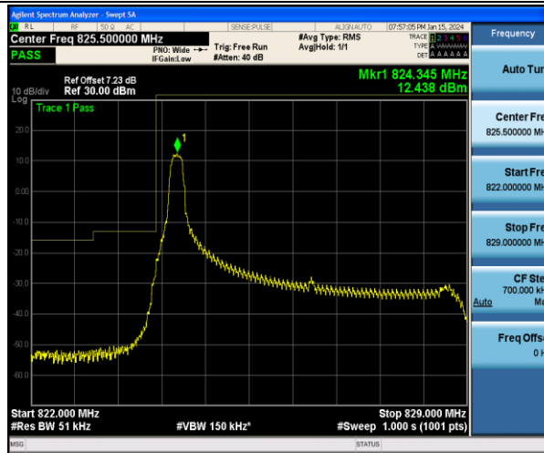
Band5_5MHz_QPSK_20425_1RB#0
