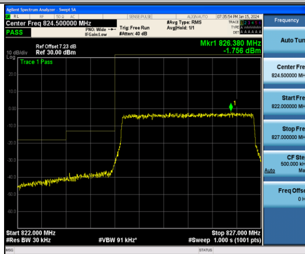
Band5_3MHz_16QAM_20415_15RB#0
