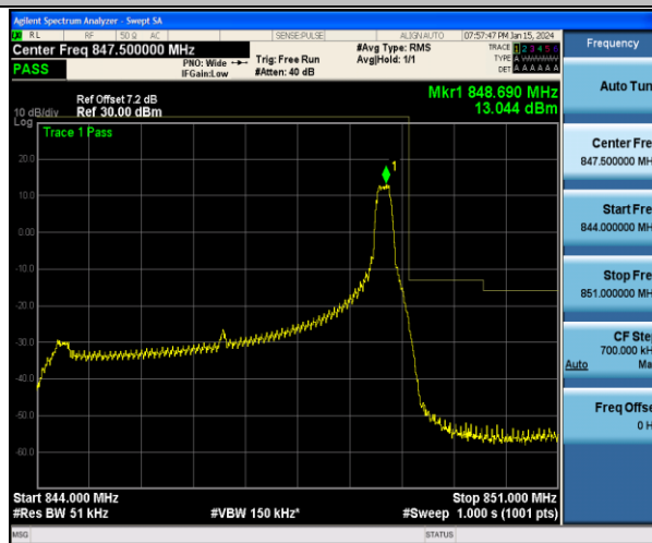
Band5_5MHz_QPSK_20625_1RB#24
