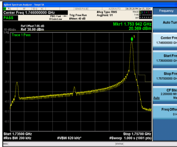
Band4_20MHz_QPSK_20300_1RB#99
