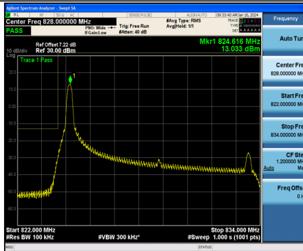
Band5_10MHz_QPSK_20450_1RB#0
