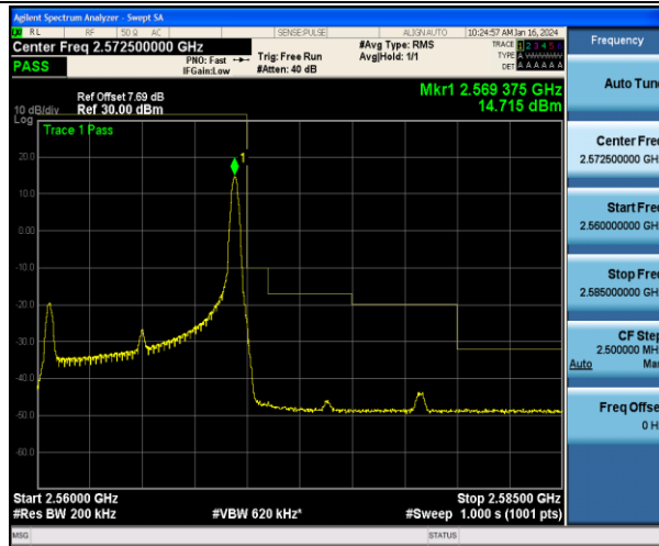
Band7_10MHz_QPSK_21400_1RB#49
