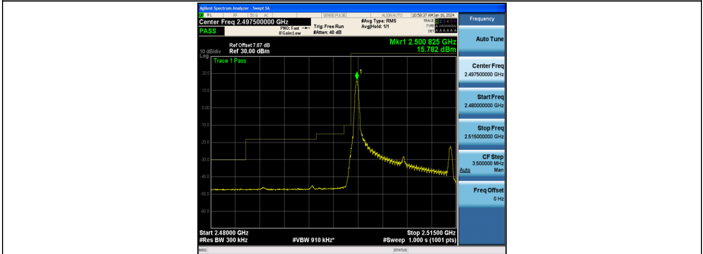
Band7_15MHz_16QAM_20825_1RB#0
