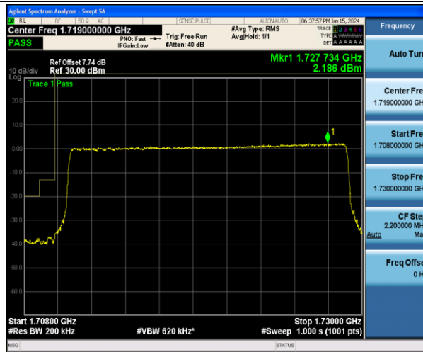
Band4_20MHz_QPSK_20050_100RB#0
