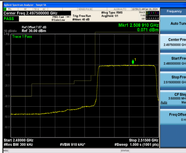
Band7_15MHz_QPSK_20825_75RB#0
