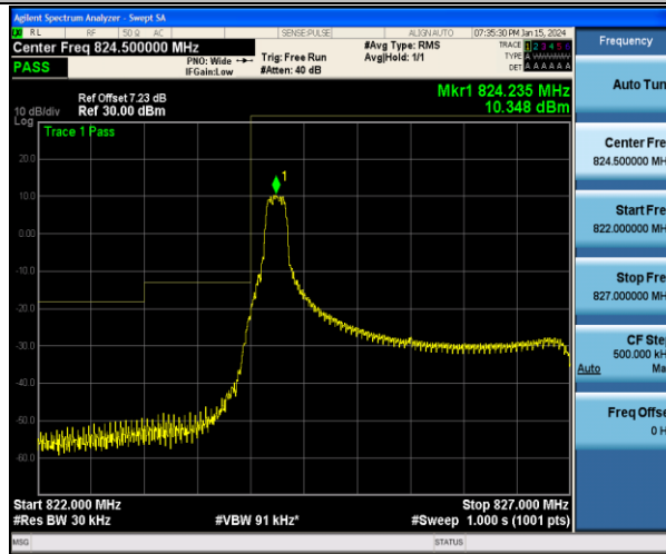
Band5_3MHz_QPSK_20415_1RB#0
