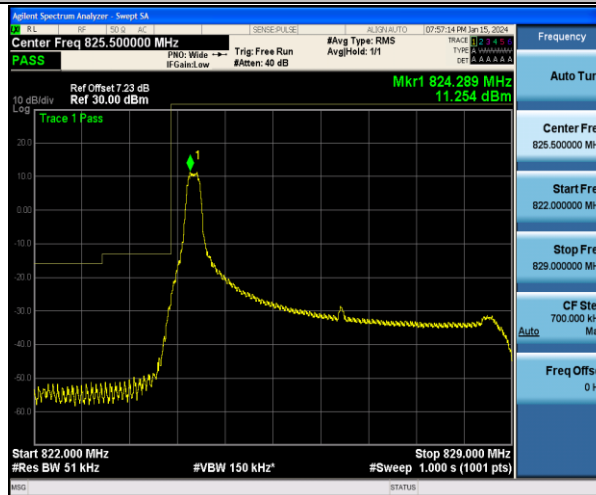
Band5_5MHz_16QAM_20425_1RB#0
