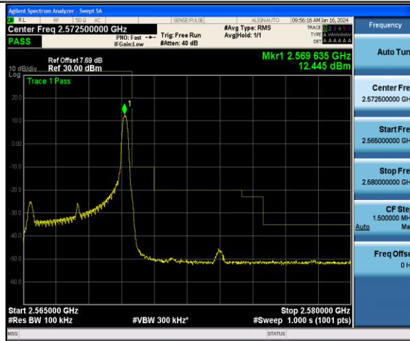
Band7_5MHz_16QAM_21425_1RB#24
