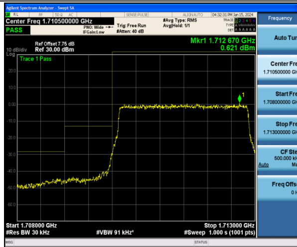
Band4_3MHz_QPSK_19965_15RB#0
