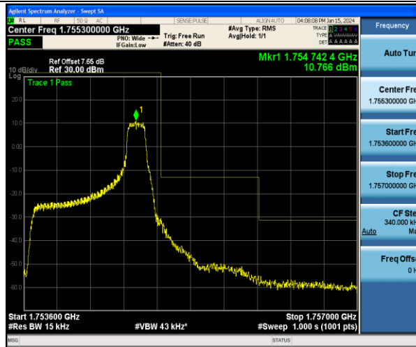
Band4_1.4MHz_QPSK_20393_1RB#5
