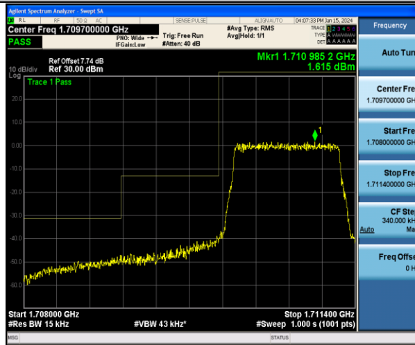
Band4_1.4MHz_QPSK_19957_6RB#0
