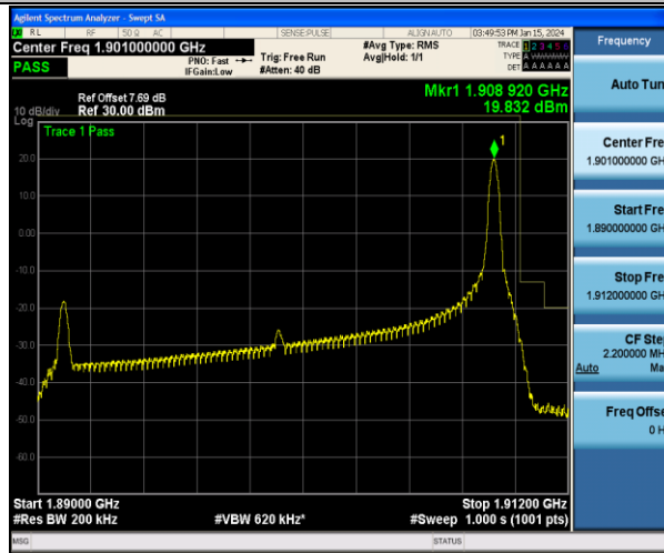
Band2_20MHz_QPSK_19100_1RB#99
