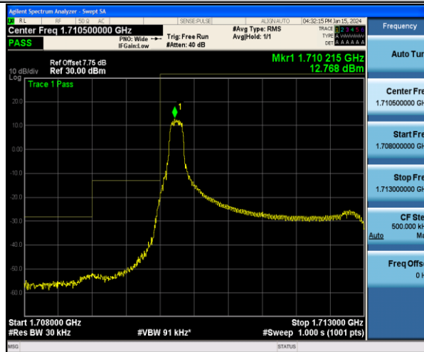
Band4_3MHz_QPSK_19965_1RB#0
