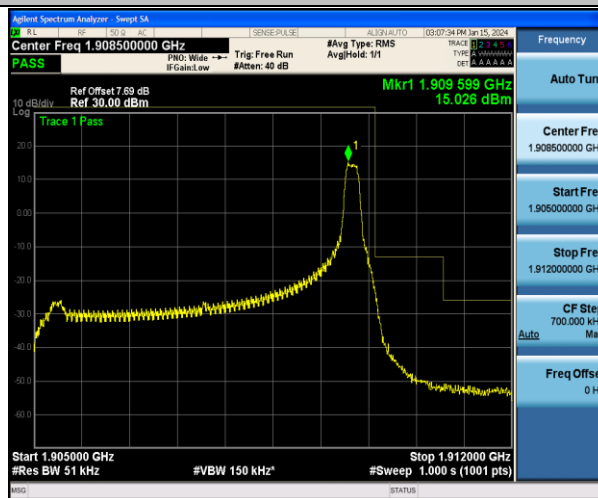
Band2_5MHz_QPSK_19175_1RB#24
