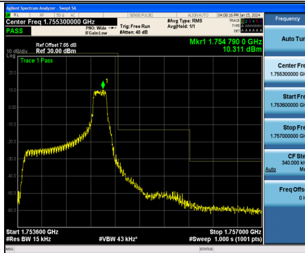
Band4_1.4MHz_16QAM_20393_1RB#5
