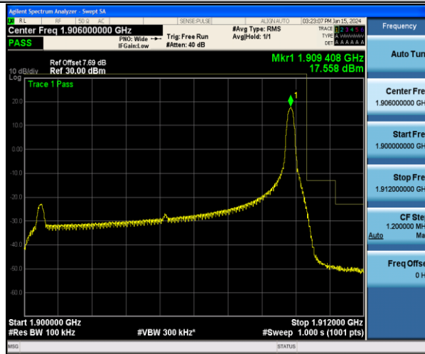
Band2_10MHz_QPSK_19150_1RB#49
