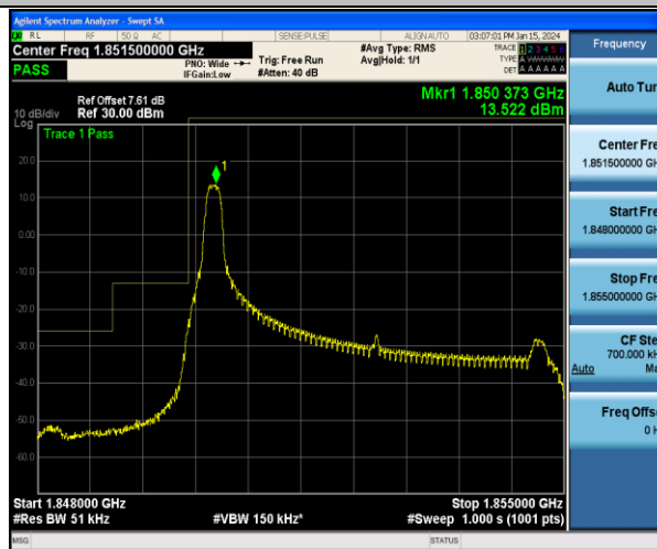
Band2_5MHz_16QAM_18625_1RB#0
