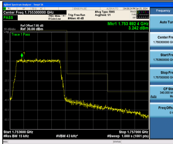
Band4_1.4MHz_QPSK_20393_6RB#0
