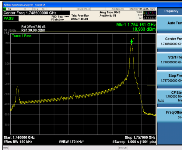
Band4_15MHz_16QAM_20325_1RB#74
