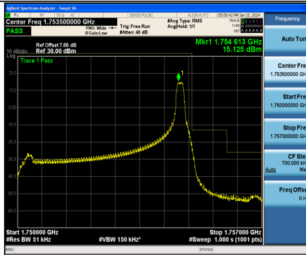
Band4_5MHz_QPSK_20375_1RB#24
