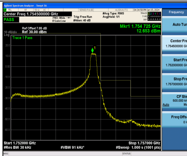
Band4_3MHz_QPSK_20385_1RB#14
