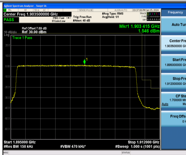
Band2_15MHz_QPSK_19125_75RB#0
