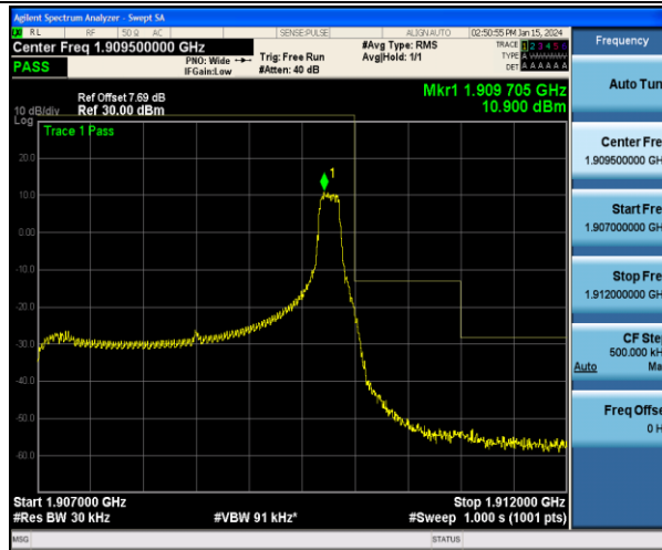
Band2_3MHz_16QAM_19185_1RB#14
