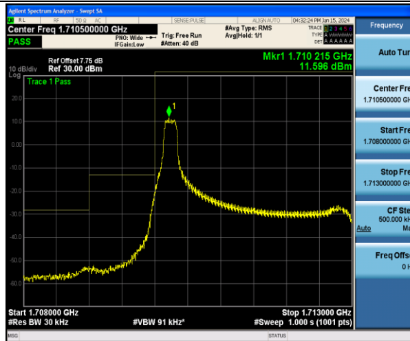
Band4_3MHz_16QAM_19965_1RB#0
