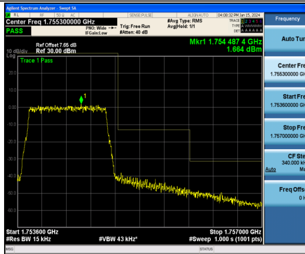
Band4_1.4MHz_16QAM_20393_6RB#0
