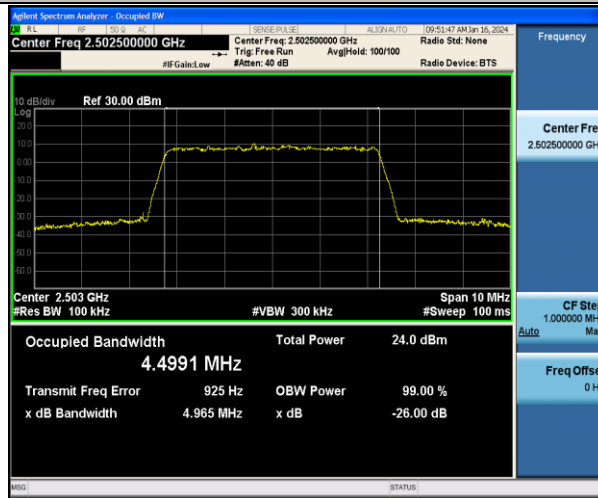
Band7-5MHz-16QAM-20775-25RB#0-PASS
