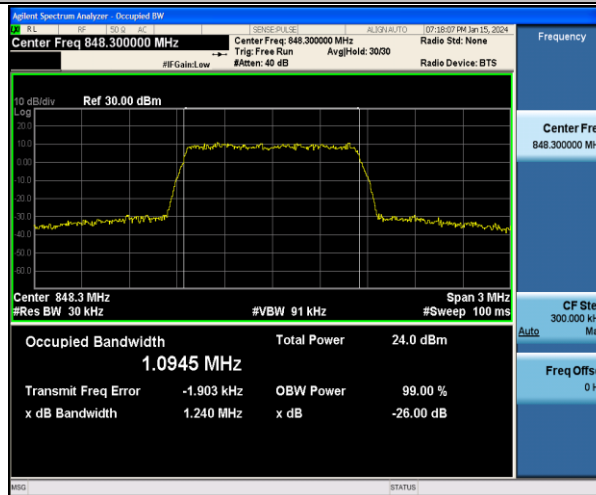
Band5-1.4MHz-QPSK-20643-6RB#0-PASS
