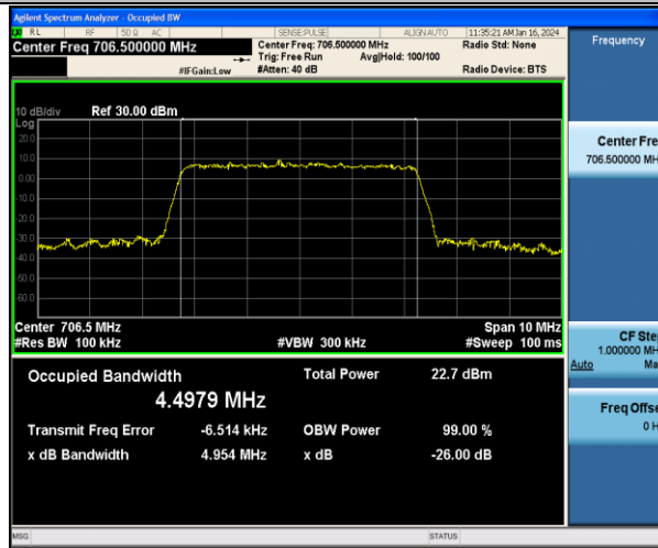
Band17-5MHz-16QAM-23755-25RB#0-PASS
