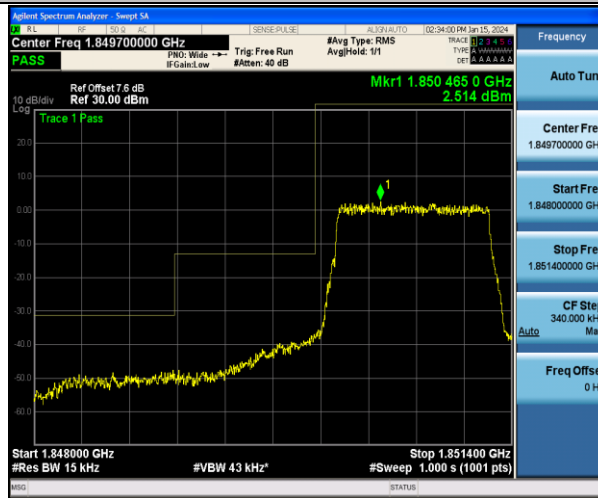
Band2_1.4MHz_QPSK_18607_6RB#0
