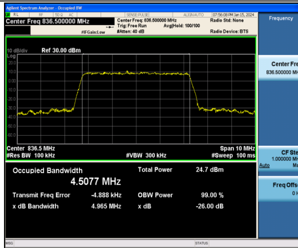
Band5-5MHz-16QAM-20525-25RB#0-PASS
