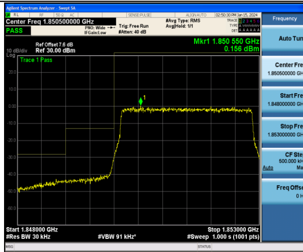
Band2_3MHz_16QAM_18615_15RB#0
