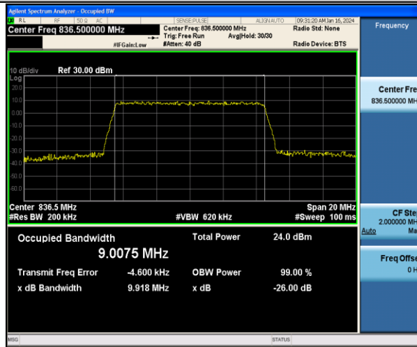
Band5-10MHz-QPSK-20525-50RB#0-PASS
