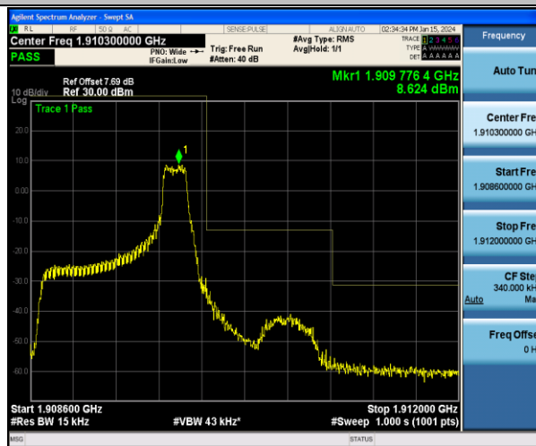
Band2_1.4MHz_16QAM_19193_1RB#5
