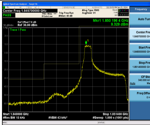
Band2_1.4MHz_16QAM_18607_1RB#0
