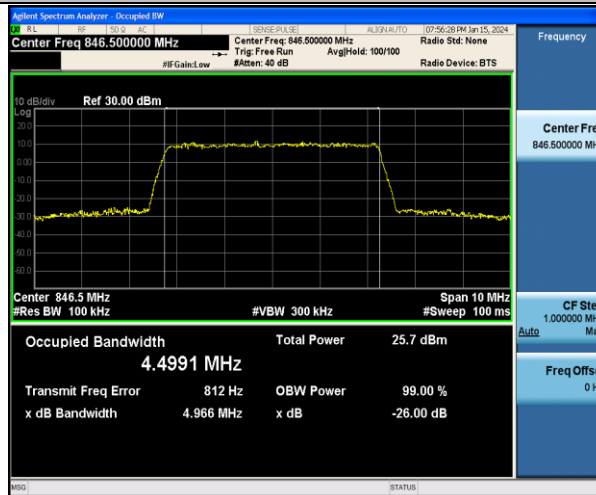
Band5-5MHz-QPSK-20625-25RB#0-PASS
