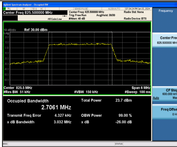
Band5-3MHz-16QAM-20415-15RB#0-PASS
