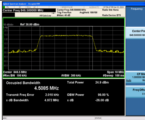
Band5-5MHz-16QAM-20625-25RB#0-PASS
