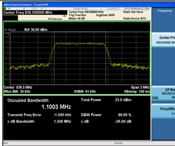
Band5-1.4MHz-16QAM-20525-6RB#0-PASS
