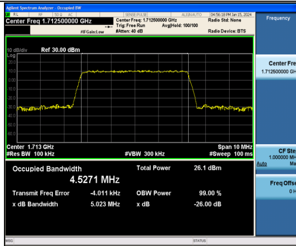
Band4-5MHz-16QAM-19975-25RB#0-PASS
