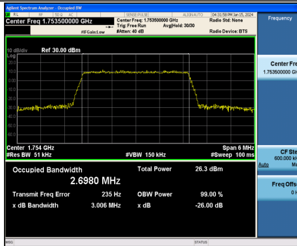
Band4-3MHz-16QAM-20385-15RB#0-PASS
