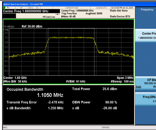
Band2-1.4MHz-16QAM-18900-6RB#0-PASS
