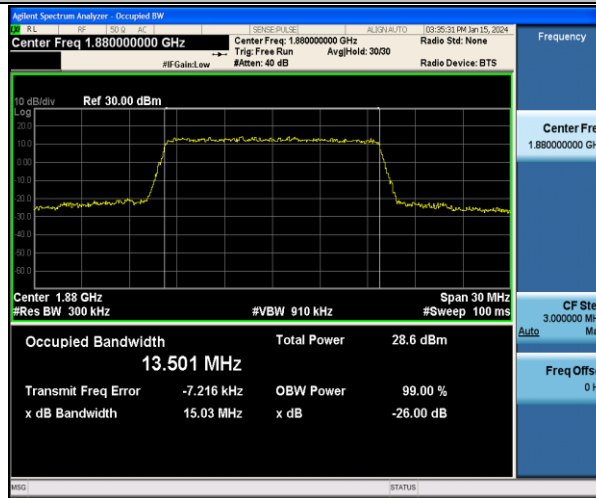
Band2-15MHz-QPSK-18900-75RB#0-PASS
