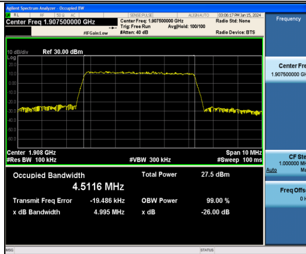
Band2-5MHz-QPSK-19175-25RB#0-PASS
