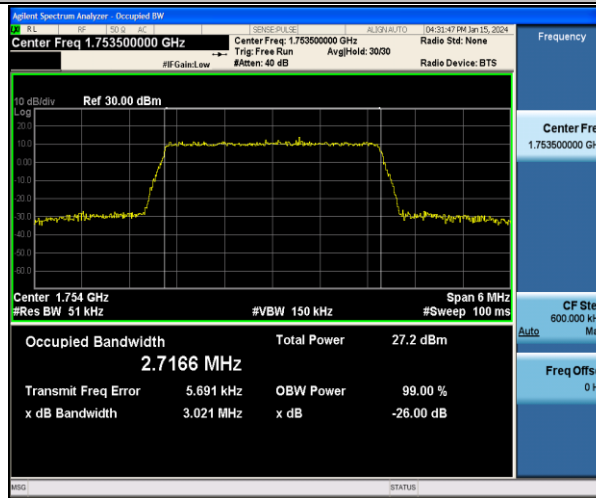
Band4-3MHz-QPSK-20385-15RB#0-PASS
