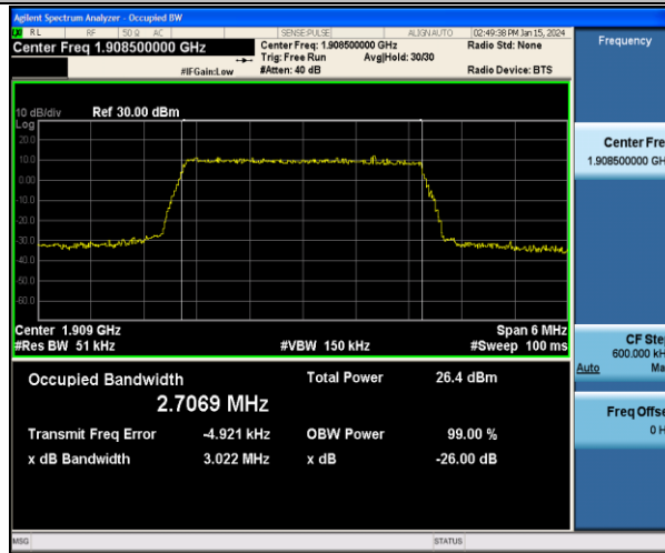
Band2-3MHz-QPSK-19185-15RB#0-PASS
