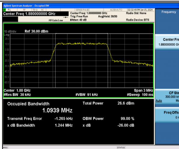
Band2-1.4MHz-QPSK-18900-6RB#0-PASS
