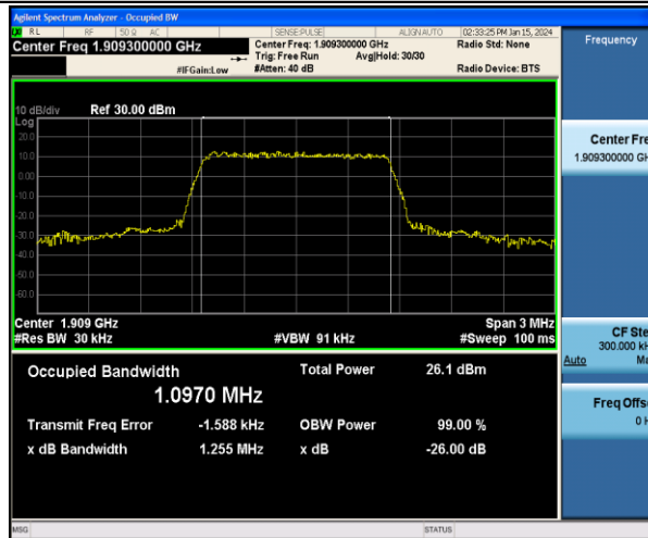
Band2-1.4MHz-16QAM-19193-6RB#0-PASS
