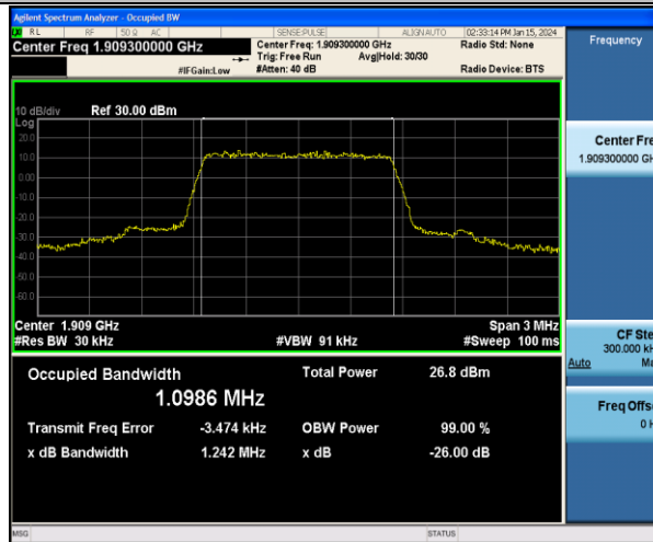
Band2-1.4MHz-QPSK-19193-6RB#0-PASS
