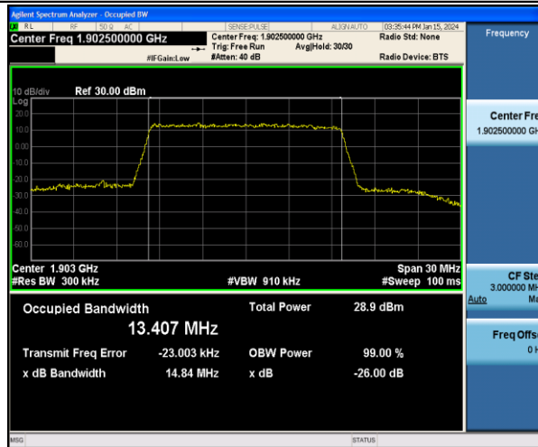
Band2-15MHz-QPSK-19125-75RB#0-PASS
