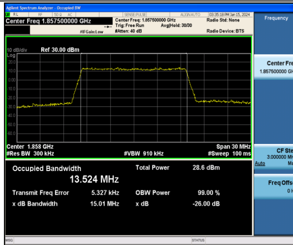
Band2-15MHz-QPSK-18675-75RB#0-PASS
