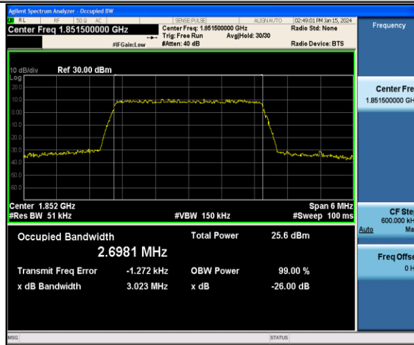
Band2-3MHz-16QAM-18615-15RB#0-PASS
