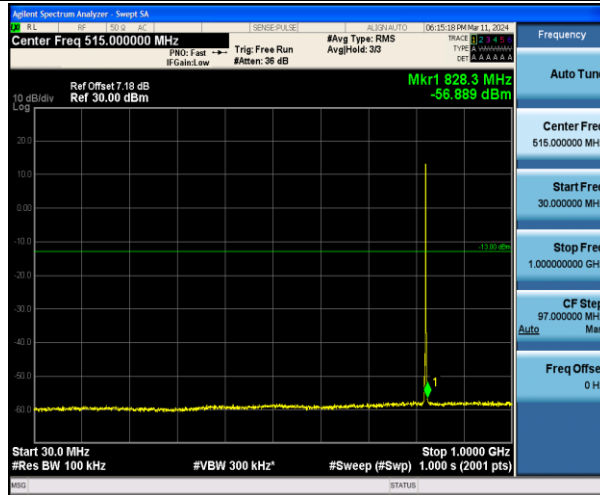
Band5_1.4MHz_16QAM_20407_1RB#0_30~1000_30~1000
