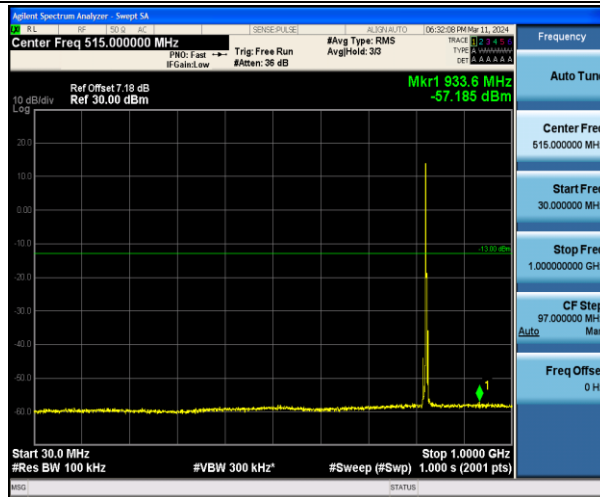
Band5_3MHz_QPSK_20415_1RB#0_30~1000_30~1000
