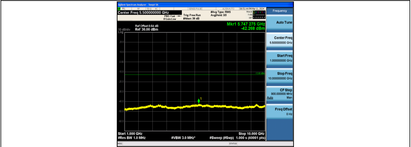
Band5_5MHz_QPSK_20525_1RB#0_1000~10000_1000~10000
