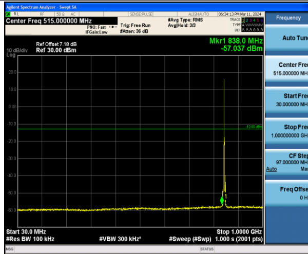
Band5_3MHz_QPSK_20635_1RB#0_30~1000_30~1000
