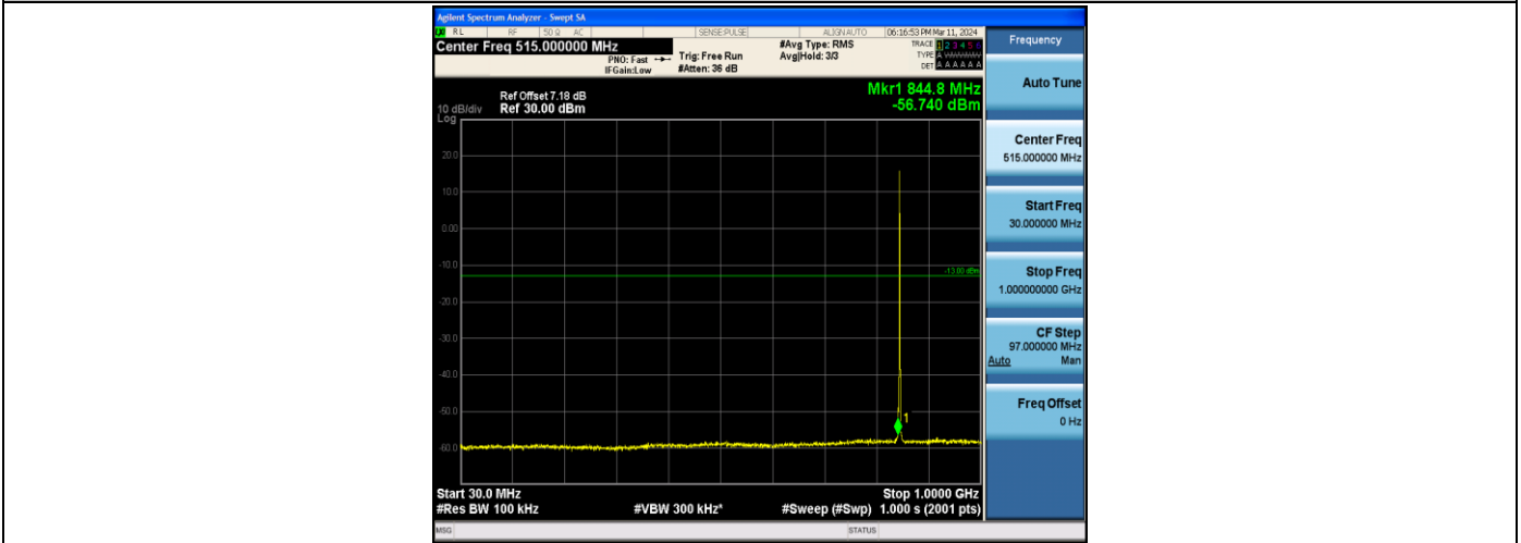
Band5_1.4MHz_QPSK_20643_1RB#0_30~1000_30~1000
