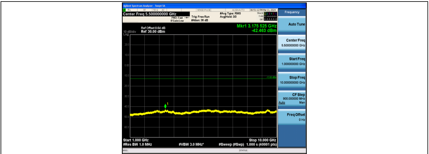
Band5_5MHz_16QAM_20425_1RB#0_1000~10000_1000~10000
