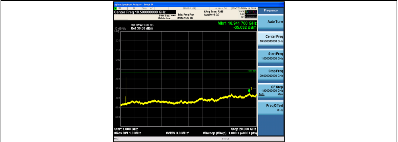
Band4_15MHz_16QAM_20325_1RB#0_1000~20000_1000~20000
