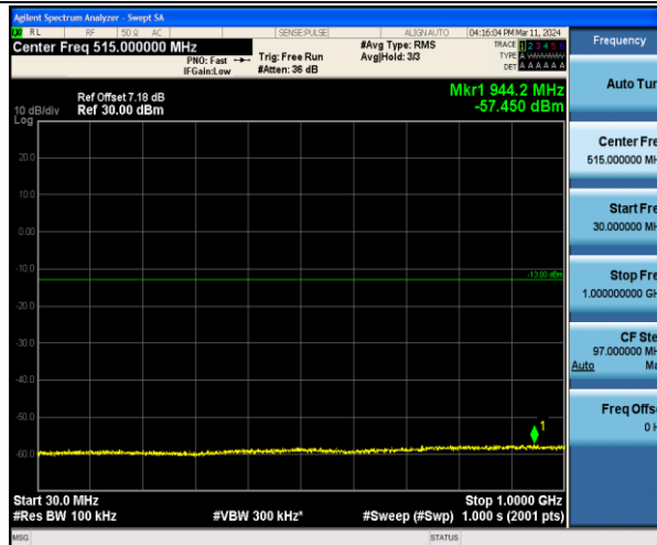
Band2_20MHz_QPSK_18700_1RB#0_30~1000_30~1000
