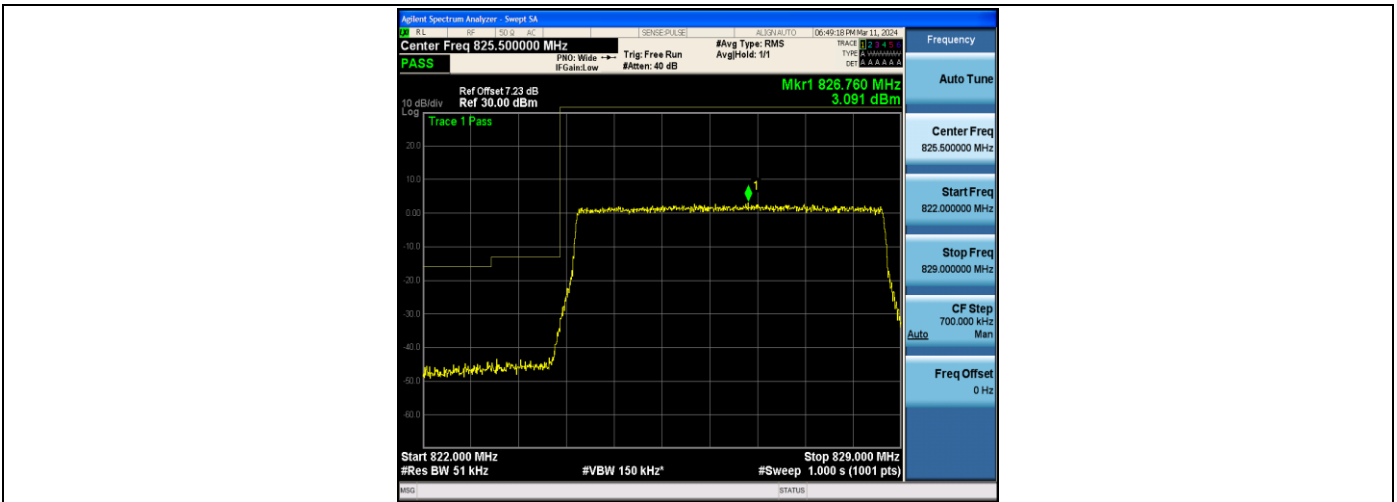
Band5_5MHz_16QAM_20425_25RB#0
