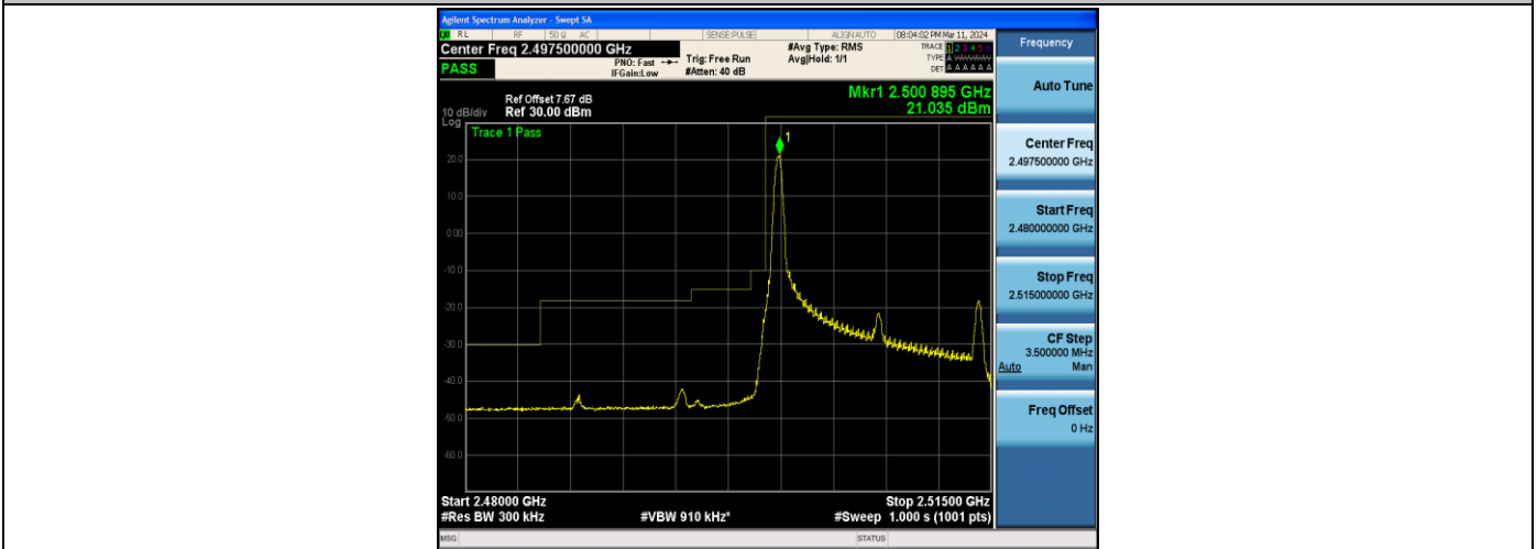
Band7_15MHz_16QAM_20825_1RB#0
