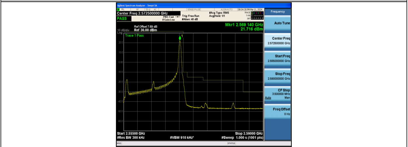
Band7_15MHz_16QAM_21375_1RB#74
