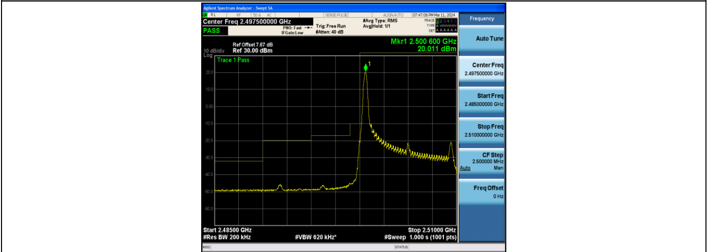
Band7_10MHz_16QAM_20800_1RB#0
