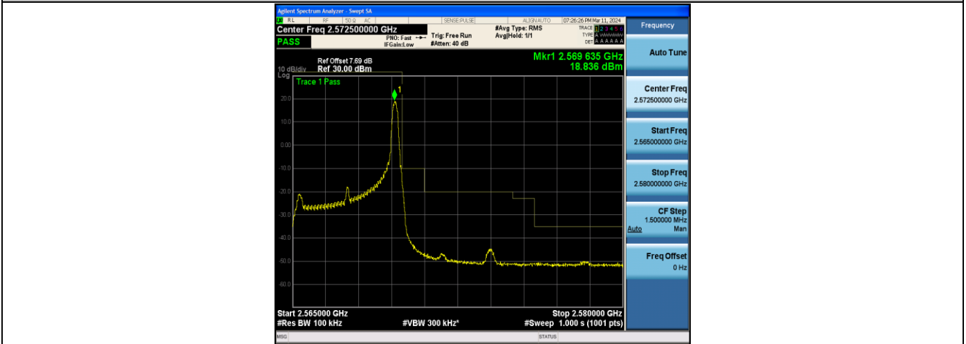
Band7_5MHz_16QAM_21425_1RB#24
