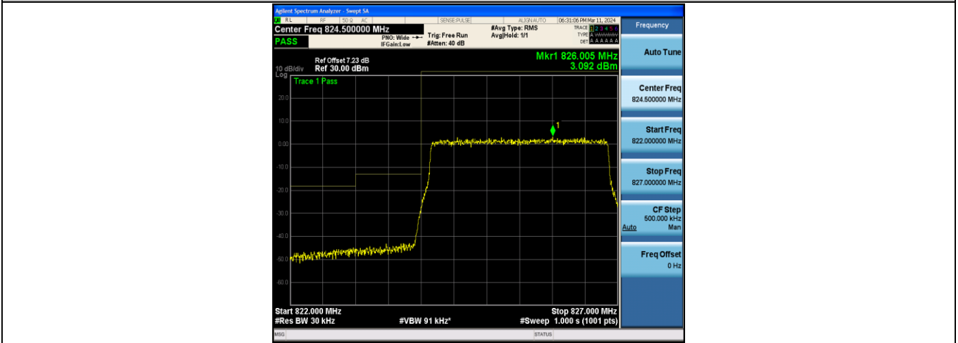
Band5_3MHz_16QAM_20415_15RB#0
