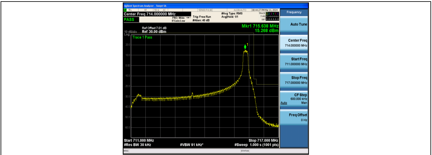
Band17_5MHz_16QAM_23825_1RB#24
