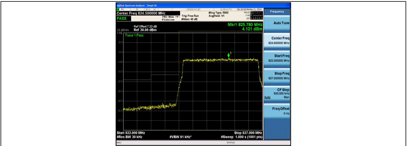
Band5_3MHz_QPSK_20415_15RB#0
