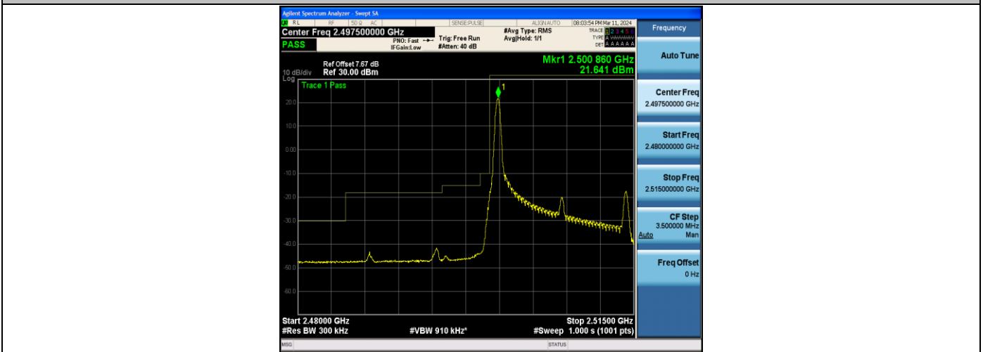
Band7_15MHz_QPSK_20825_1RB#0
