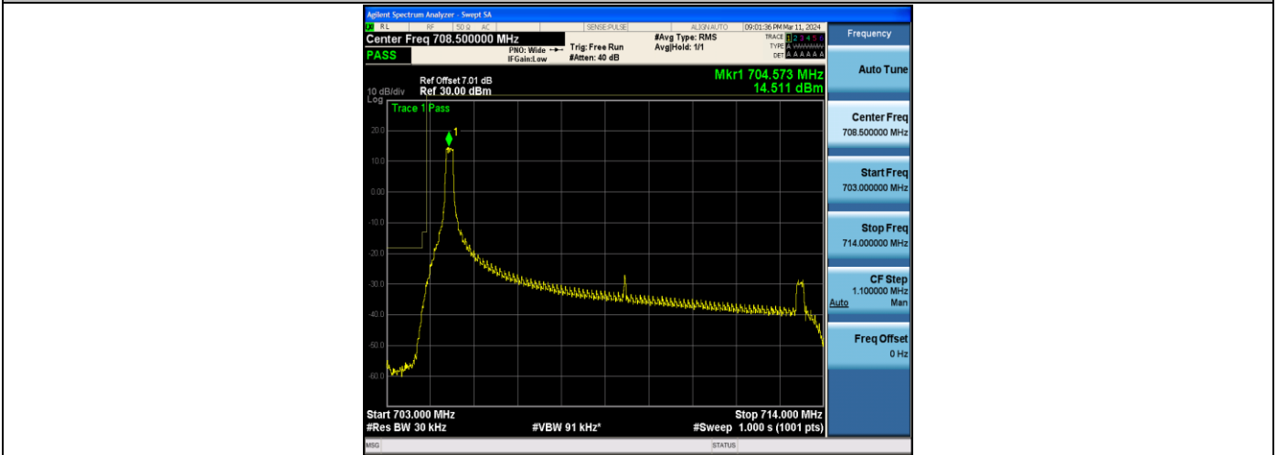
Band17_10MHz_16QAM_23780_1RB#0
