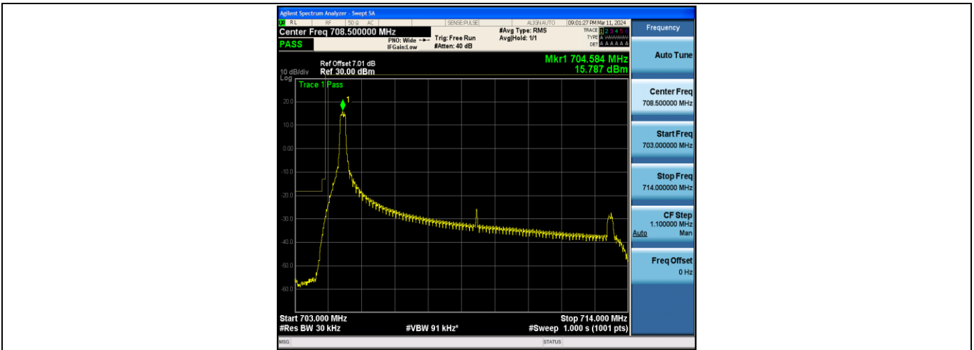
Band17_10MHz_QPSK_23780_1RB#0
