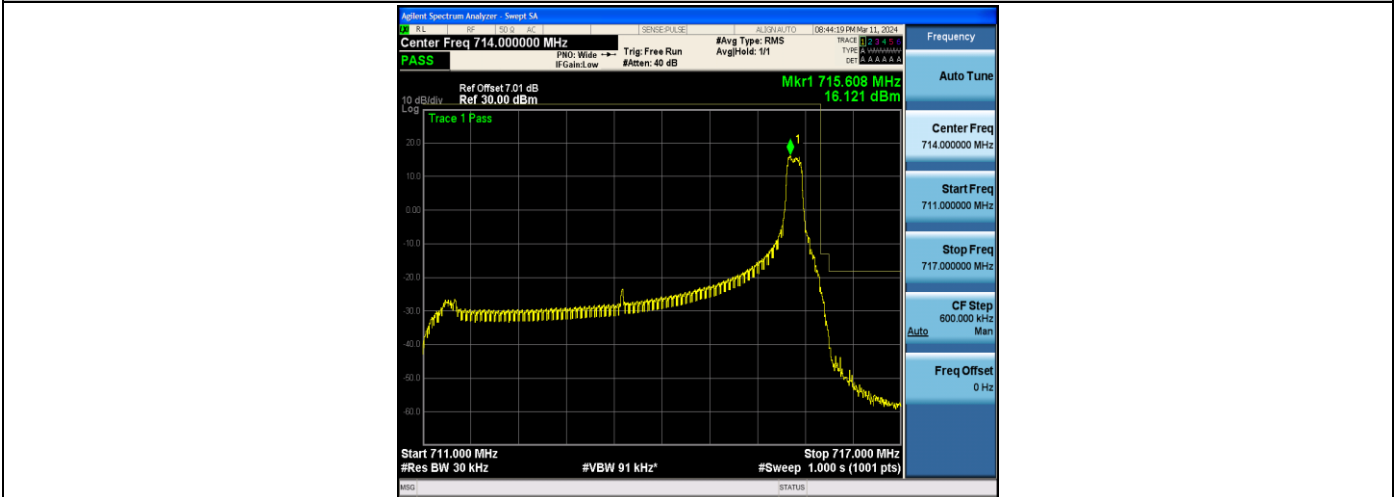
Band17_5MHz_QPSK_23825_1RB#24
