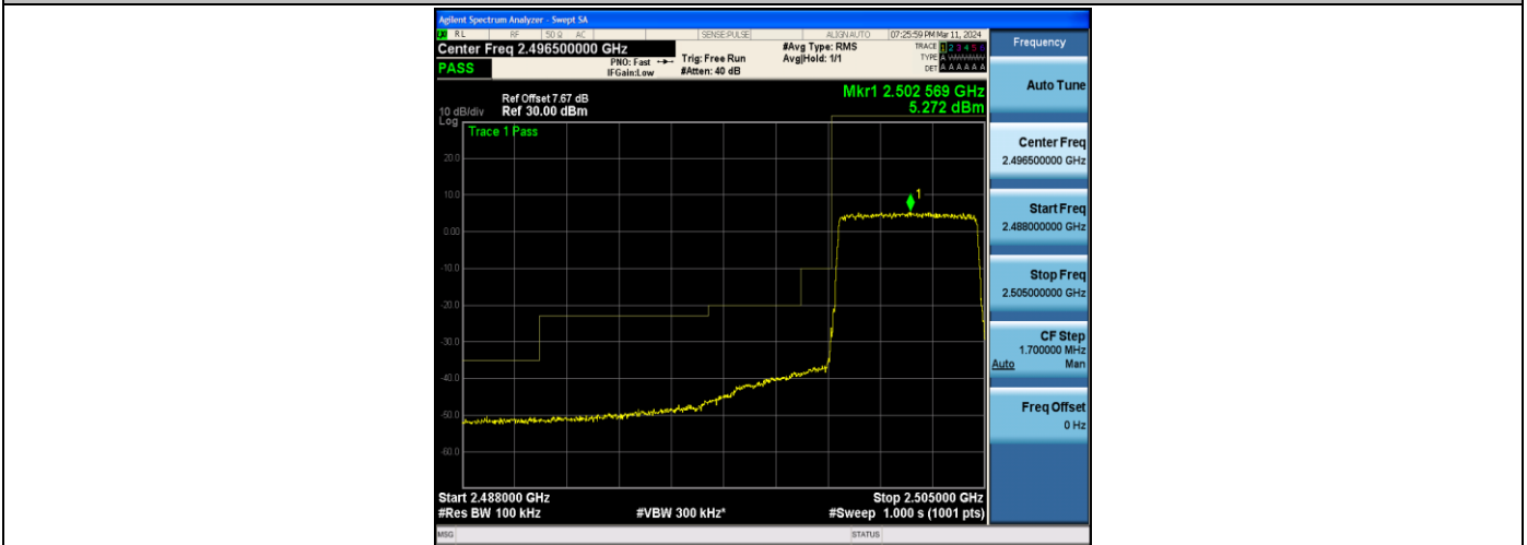
Band7_5MHz_16QAM_20775_25RB#0
