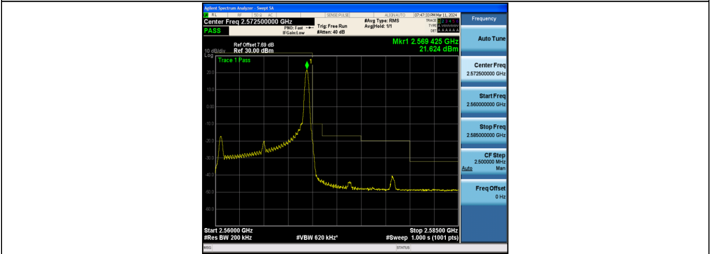
Band7_10MHz_16QAM_21400_1RB#49
