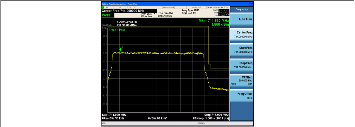
Band17_5MHz_QPSK_23825_25RB#0
