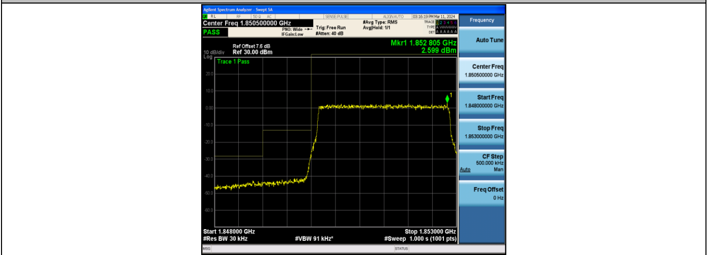
Band2_3MHz_16QAM_18615_15RB#0
