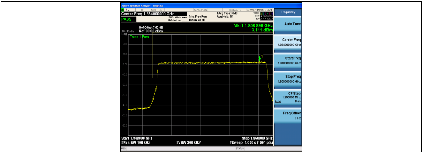
Band2_10MHz_QPSK_18650_50RB#0
