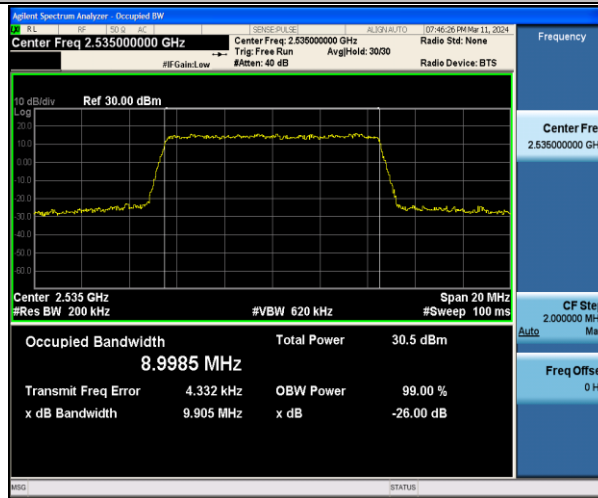
Band7-10MHz-QPSK-21100-50RB#0-PASS
