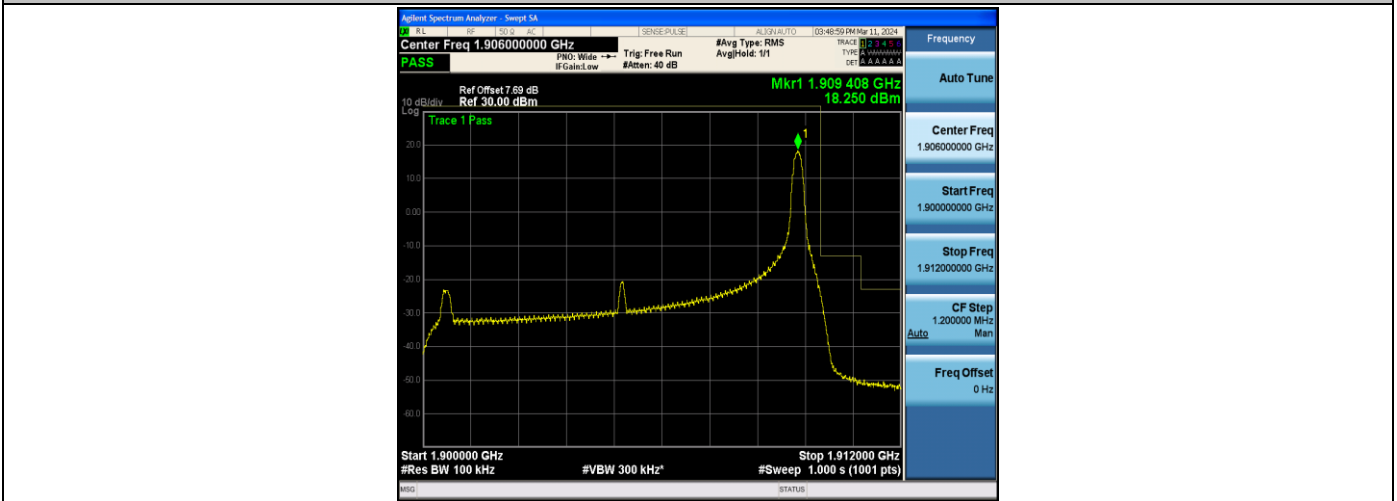
Band2_10MHz_16QAM_19150_1RB#49
