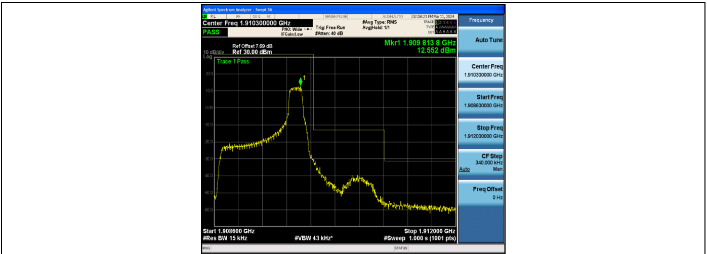
Band2_1.4MHz_QPSK_19193_1RB#5
