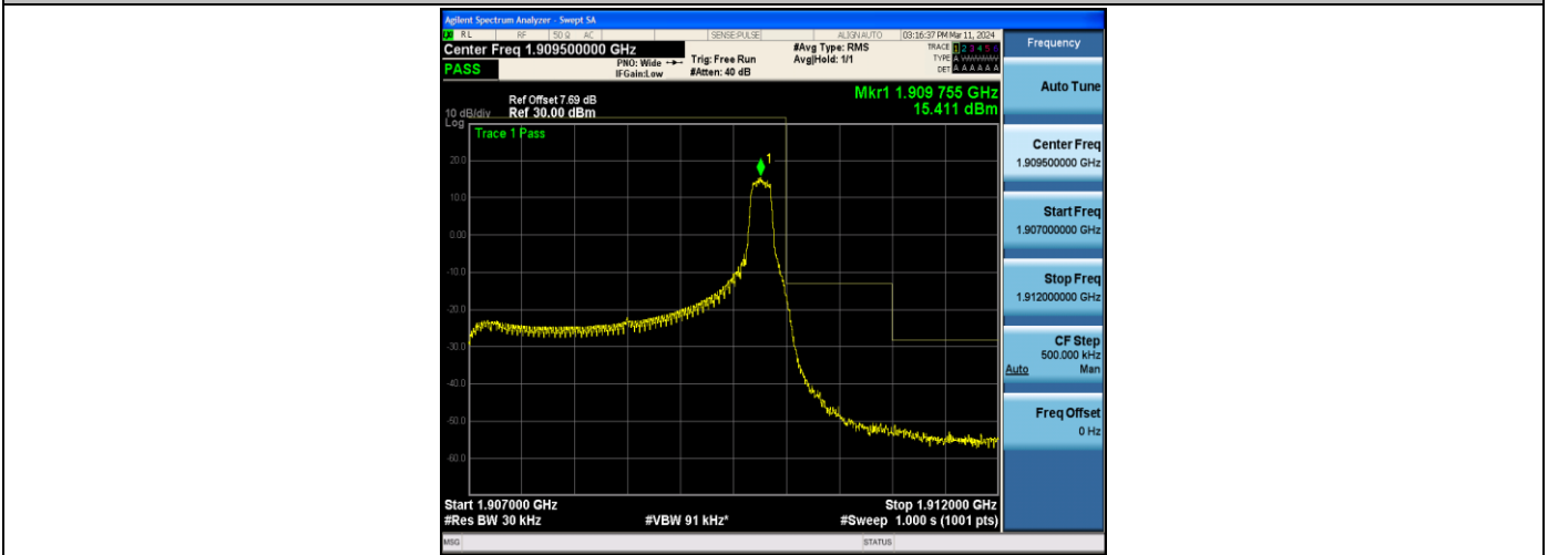
Band2_3MHz_QPSK_19185_1RB#14
