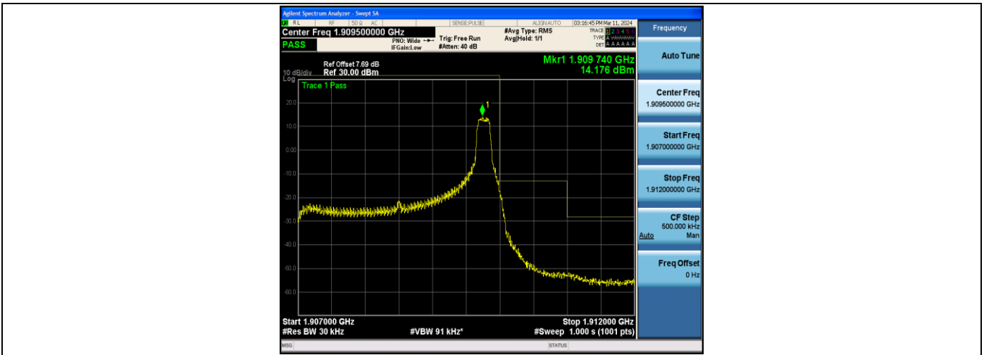
Band2_3MHz_16QAM_19185_1RB#14
