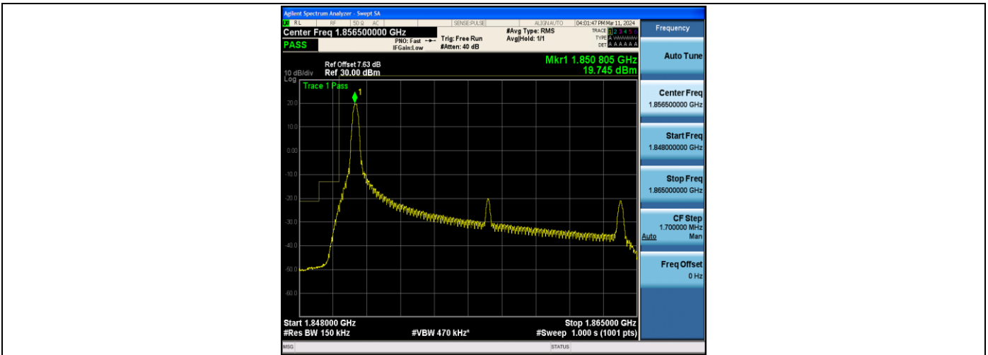
Band2_15MHz_16QAM_18675_1RB#0
