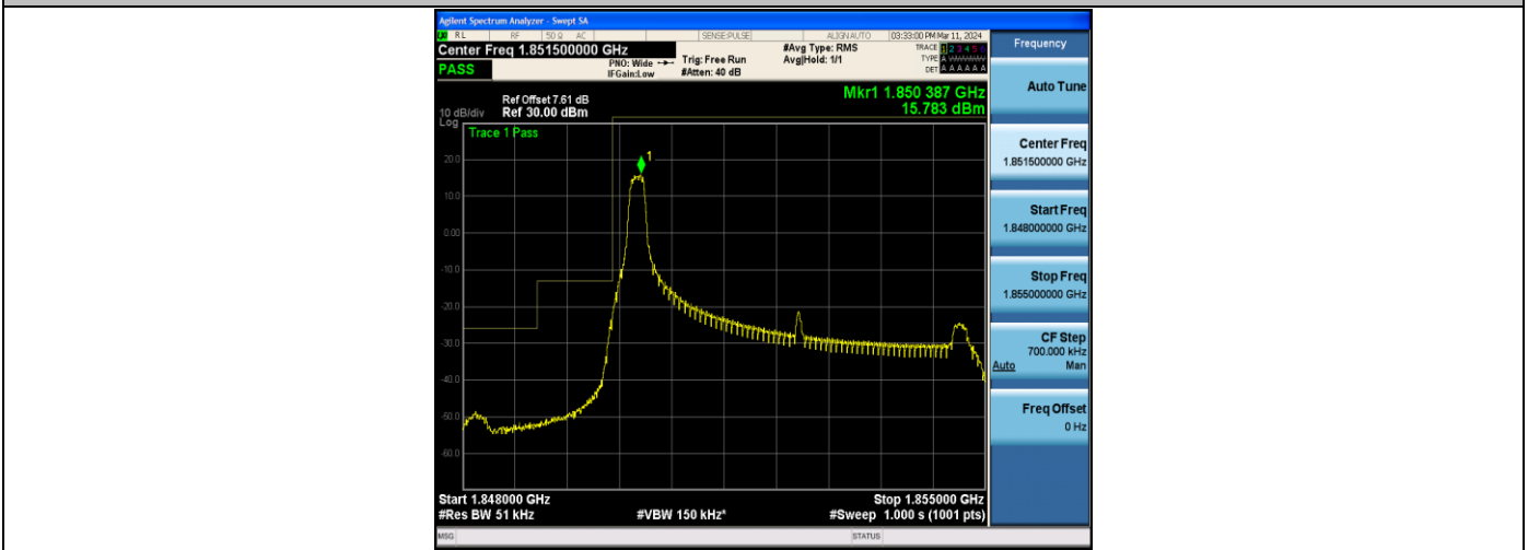
Band2_5MHz_16QAM_18625_1RB#0
