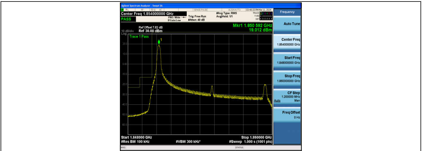
Band2_10MHz_16QAM_18650_1RB#0
