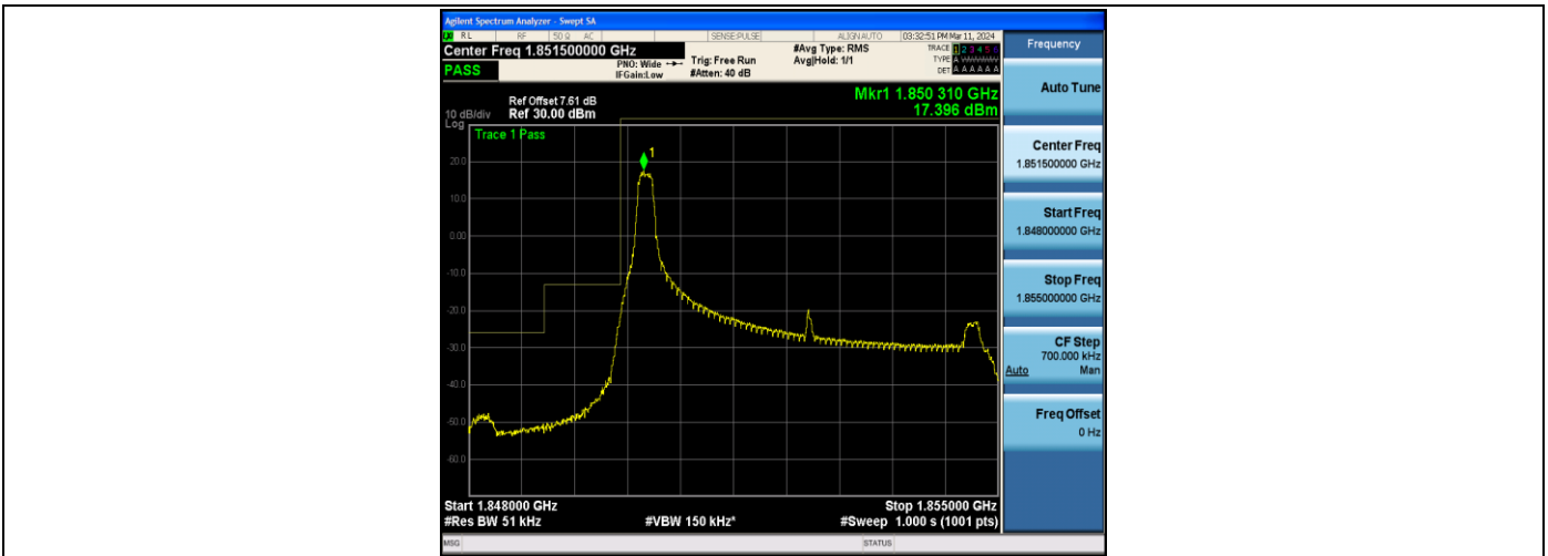
Band2_5MHz_QPSK_18625_1RB#0
