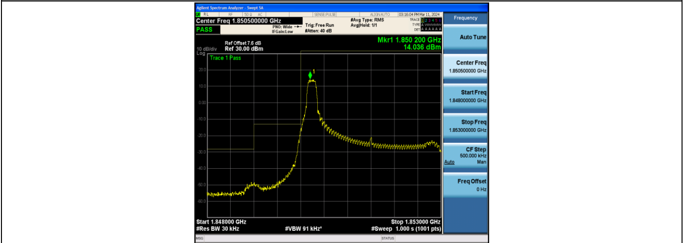
Band2_3MHz_16QAM_18615_1RB#0
