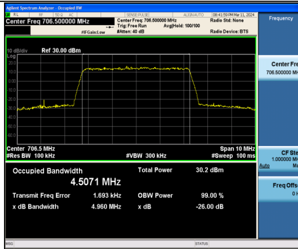
Band17-5MHz-16QAM-23755-25RB#0-PASS
