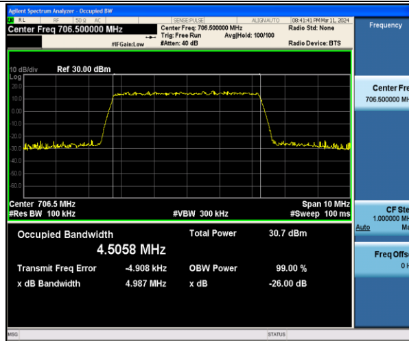
Band17-5MHz-QPSK-23755-25RB#0-PASS
