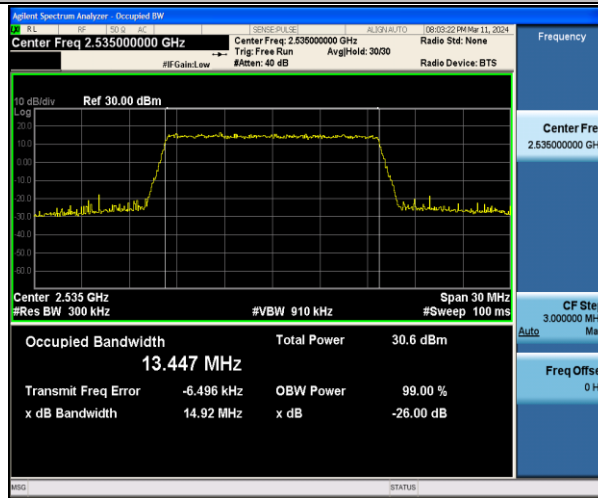
Band7-15MHz-QPSK-21100-75RB#0-PASS
