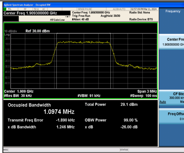
Band2-1.4MHz-QPSK-19193-6RB#0-PASS
