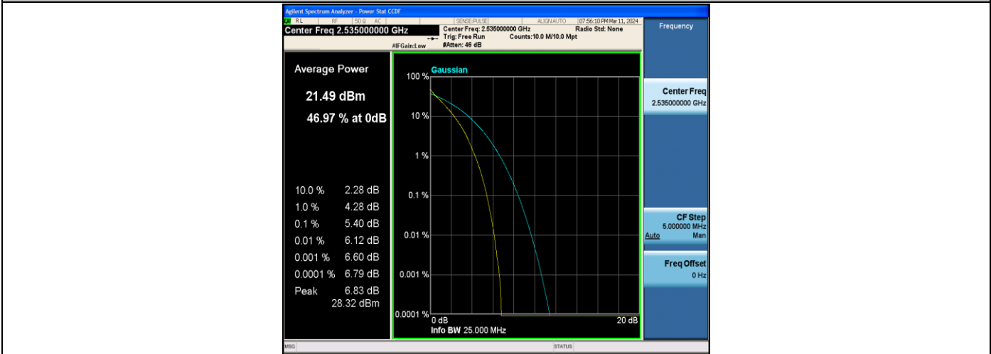
Band7-10MHz-QPSK-21100-50RB#0-PASS
