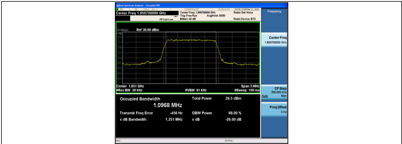
Band2-1.4MHz-QPSK-18607-6RB#0-PASS
