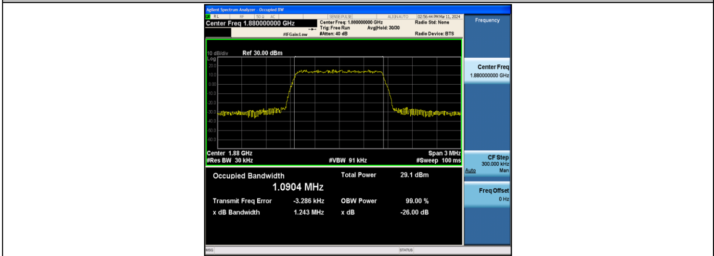
Band2-1.4MHz-QPSK-18900-6RB#0-PASS
