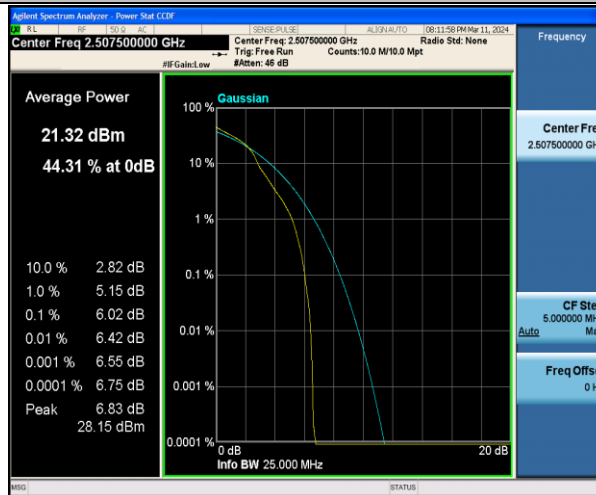
Band7-15MHz-16QAM-20825-1RB#0-PASS
