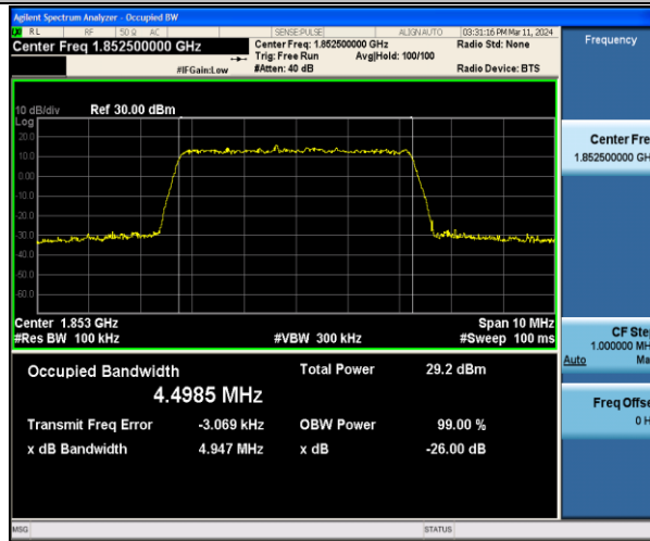
Band2-5MHz-16QAM-18625-25RB#0-PASS
