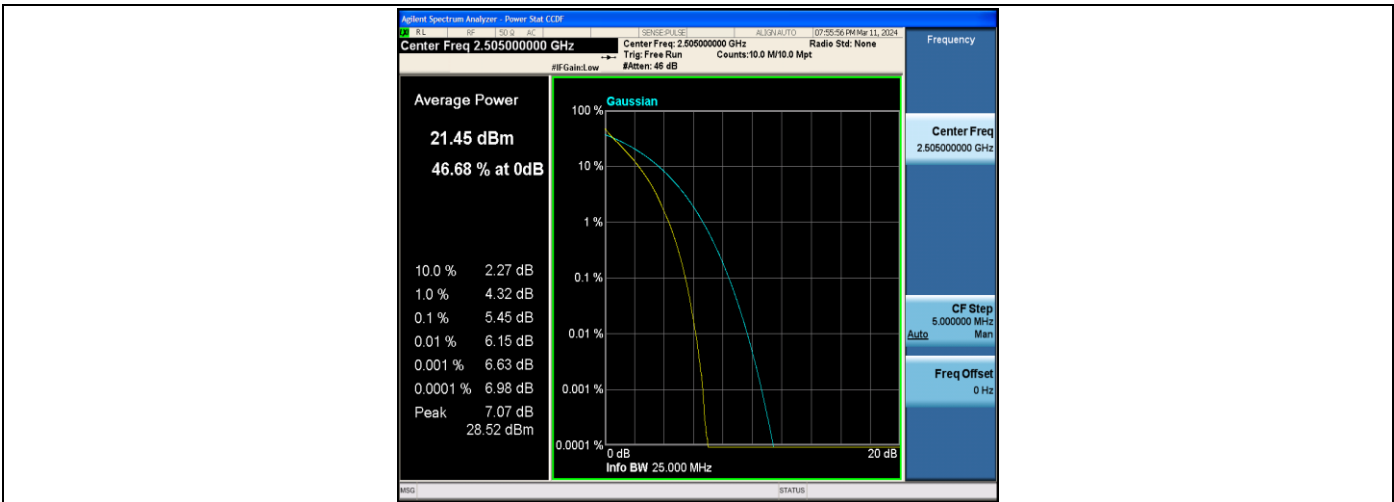
Band7-10MHz-QPSK-20800-50RB#0-PASS
