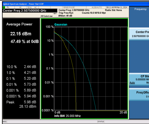
Band7-15MHz-QPSK-20825-1RB#0-PASS
