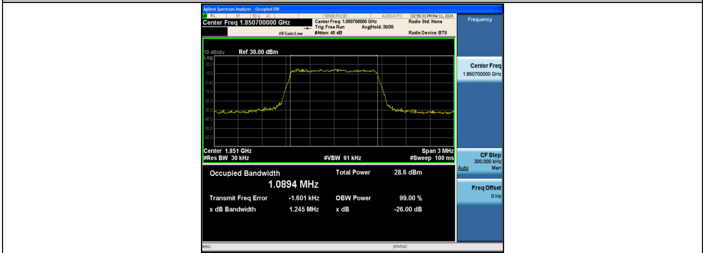
Band2-1.4MHz-16QAM-18607-6RB#0-PASS
