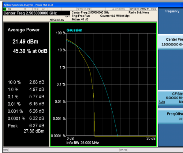
Band7-10MHz-16QAM-20800-1RB#0-PASS
