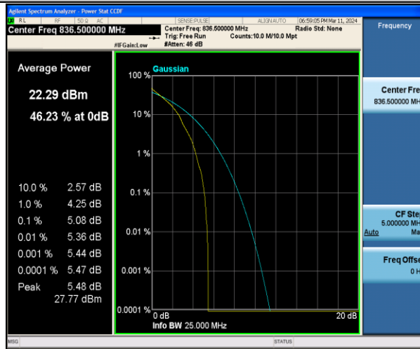
Band5-5MHz-QPSK-20525-1RB#0-PASS
