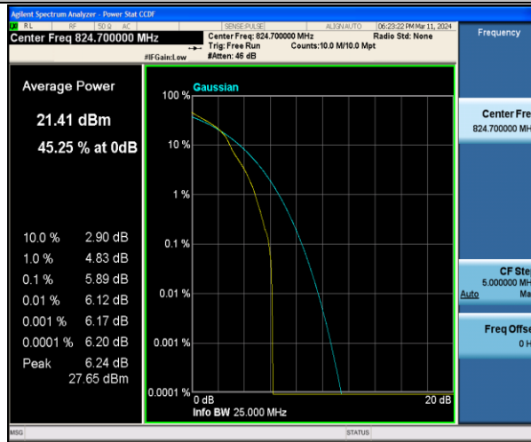
Band5-1.4MHz-16QAM-20407-1RB#0-PASS
