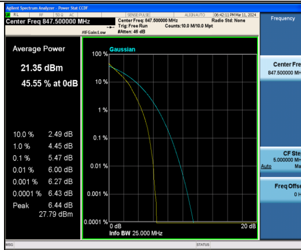
Band5-3MHz-QPSK-20635-15RB#0-PASS
