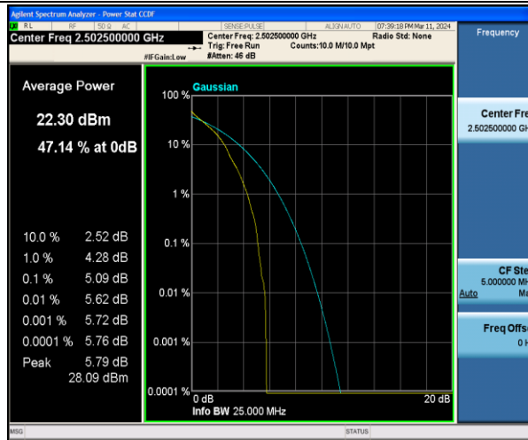
Band7-5MHz-QPSK-20775-1RB#0-PASS
