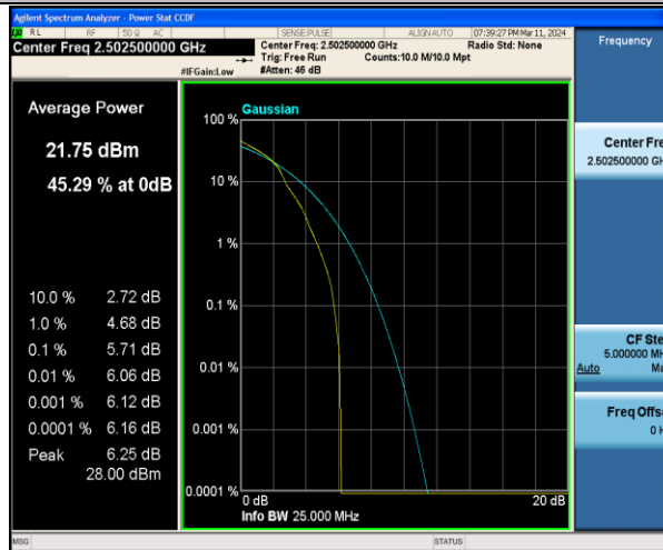
Band7-5MHz-16QAM-20775-1RB#0-PASS
