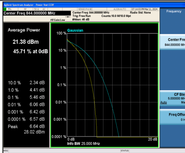
Band5-10MHz-QPSK-20600-50RB#0-PASS
