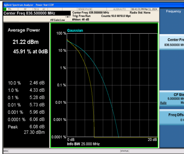
Band5-3MHz-QPSK-20525-15RB#0-PASS
