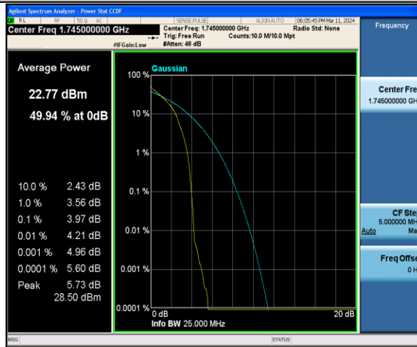
Band4-20MHz-QPSK-20300-1RB#0-PASS
