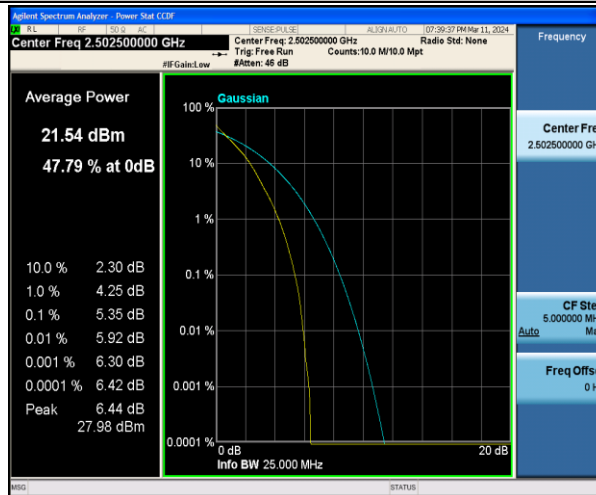
Band7-5MHz-QPSK-20775-25RB#0-PASS
