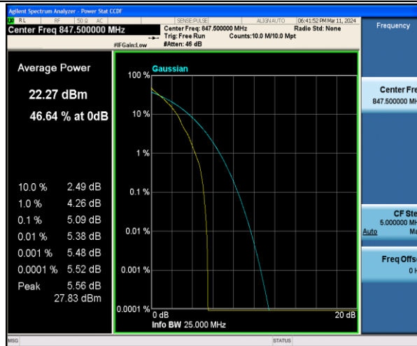
Band5-3MHz-QPSK-20635-1RB#0-PASS
