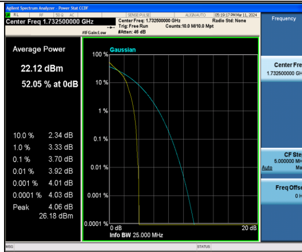
Band4-5MHz-QPSK-20175-1RB#0-PASS
