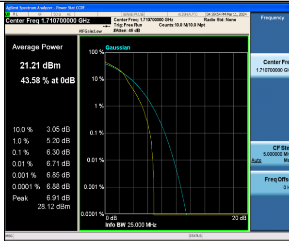
Band4-1.4MHz-16QAM-19957-1RB#0-PASS
