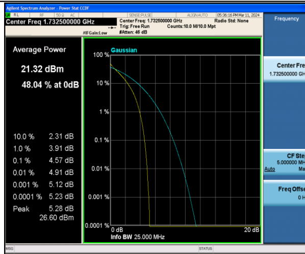
Band4-10MHz-QPSK-20175-50RB#0-PASS
