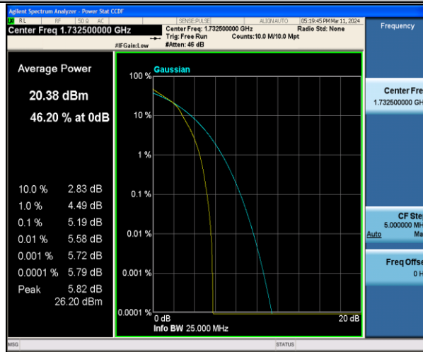
Band4-5MHz-16QAM-20175-25RB#0-PASS
