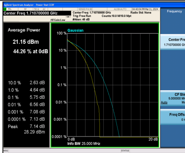
Band4-1.4MHz-QPSK-19957-6RB#0-PASS
