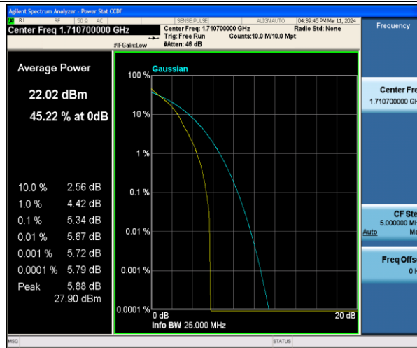
Band4-1.4MHz-QPSK-19957-1RB#0-PASS
