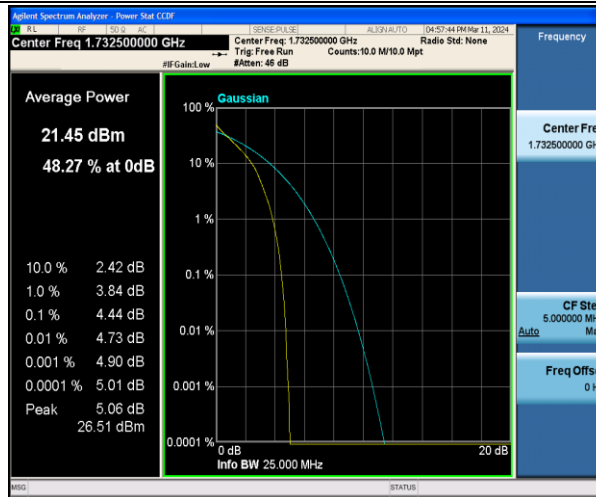
Band4-3MHz-QPSK-20175-15RB#0-PASS
