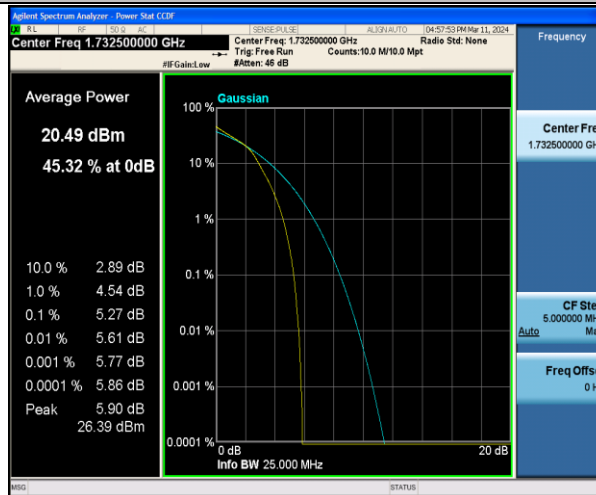
Band4-3MHz-16QAM-20175-15RB#0-PASS
