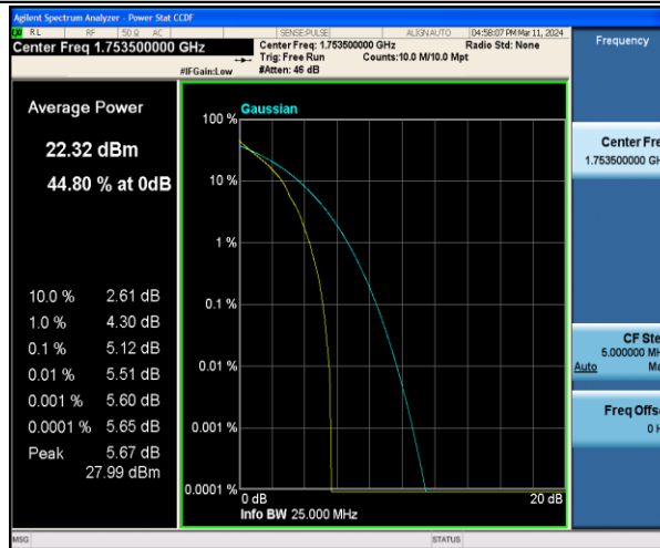
Band4-3MHz-QPSK-20385-1RB#0-PASS
