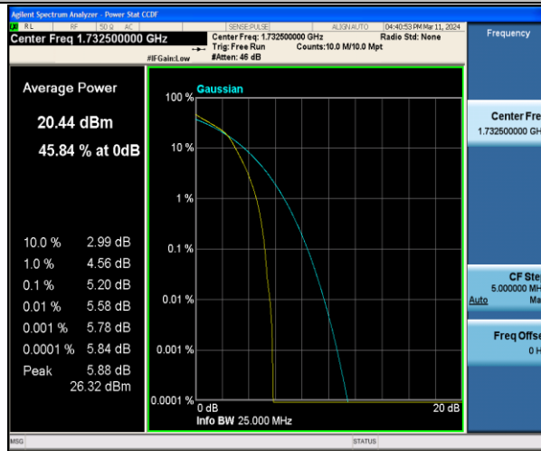
Band4-1.4MHz-16QAM-20175-6RB#0-PASS
