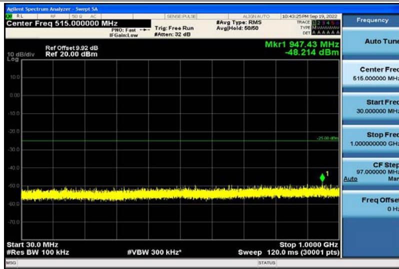
Band7-20MHz-16QAM-20850-1RB#0-30~1000MHz
