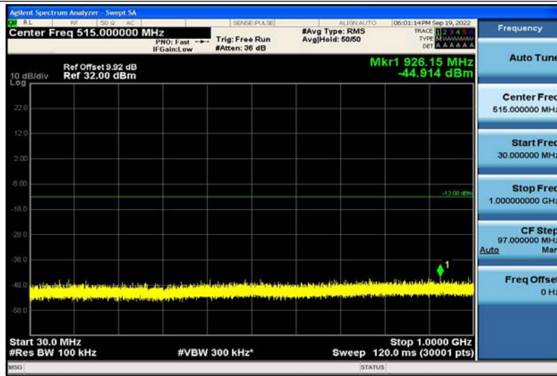
Band4-1.4MHz-QPSK-19957-1RB#0-30~1000MHz
