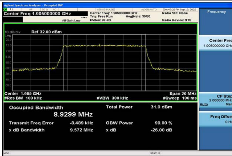
Band2-10MHz-16QAM-19150-50RB#0-8.9299
