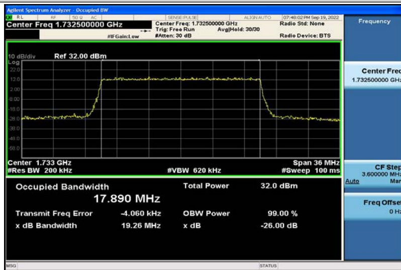
Band4-20MHz-16QAM-20175-100RB#0-17.890
