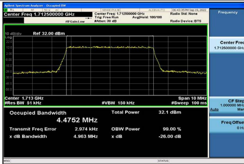
Band4-5MHz-16QAM-19975-25RB#0-4.4752
