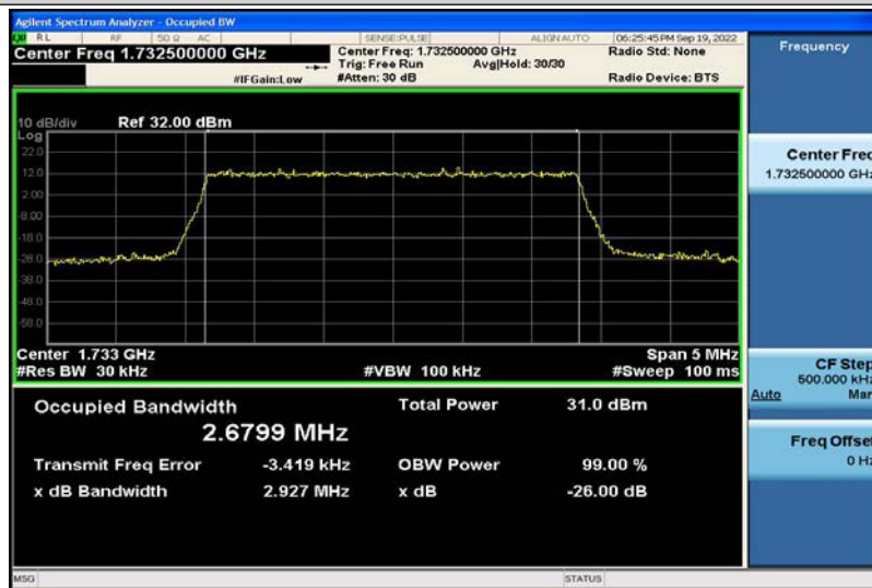
Band4-3MHz-16QAM-20175-15RB#0-2.6799
