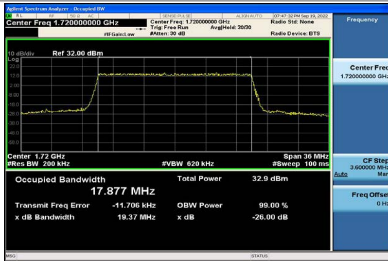
Band4-20MHz-QPSK-20050-100RB#0-17.877
