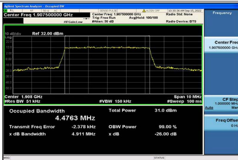
Band2-5MHz-QPSK-19175-25RB#0-4.4763
