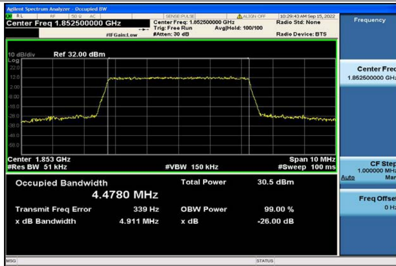
Band2-5MHz-16QAM-18625-25RB#0-4.4780
