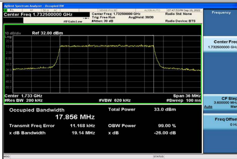
Band4-20MHz-QPSK-20175-100RB#0-17.856
