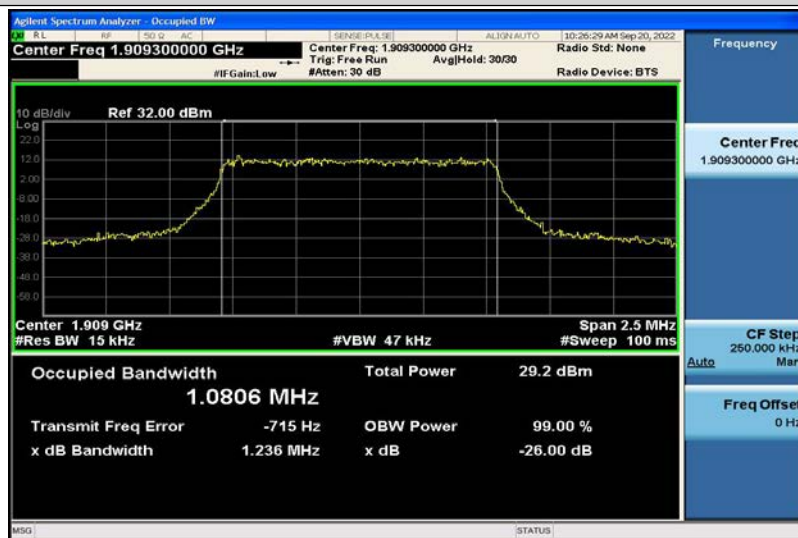
Band2-1.4MHz-16QAM-19193-6RB#0-1.0806
