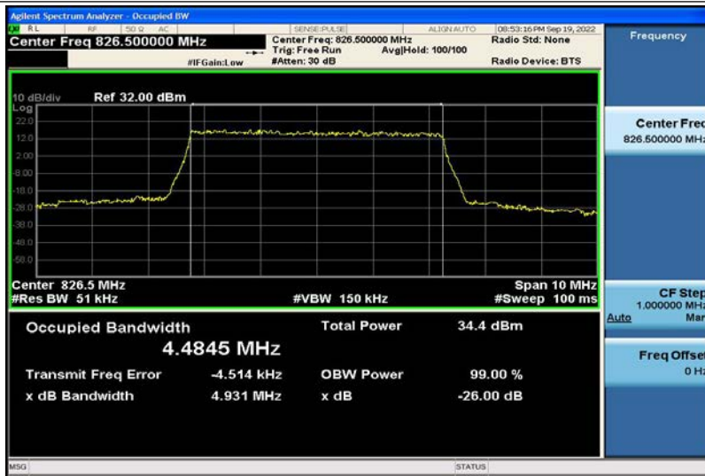
Band5-5MHz-QPSK-20425-25RB#0-4.4845
