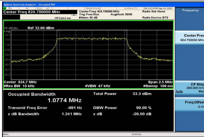
Band5-1.4MHz-QPSK-20407-6RB#0-1.0774
