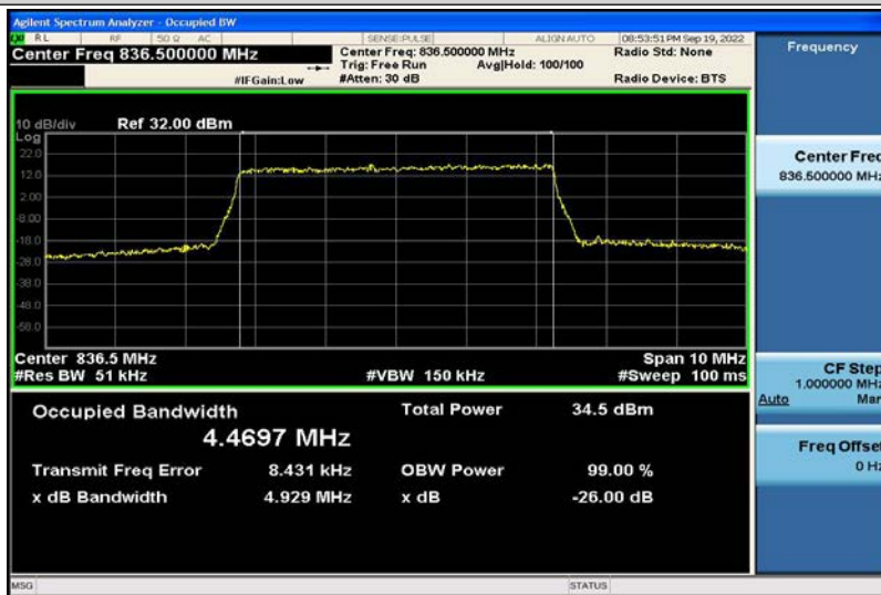
Band5-5MHz-QPSK-20525-25RB#0-4.4697
