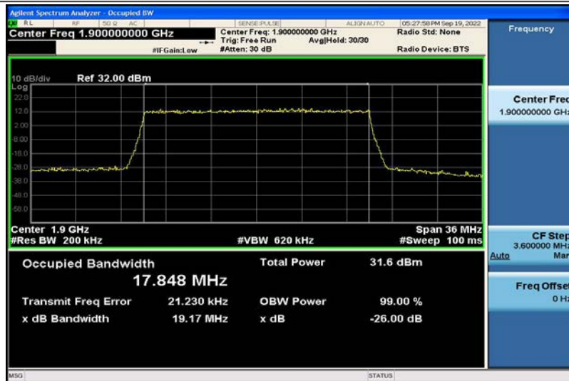
Band2-20MHz-16QAM-19100-100RB#0-17.848
