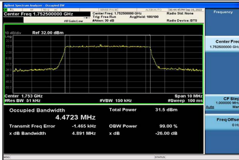
Band4-5MHz-16QAM-20375-25RB#0-4.4723
