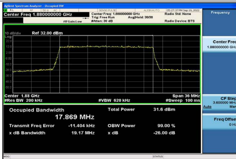
Band2-20MHz-16QAM-18900-100RB#0-17.869
