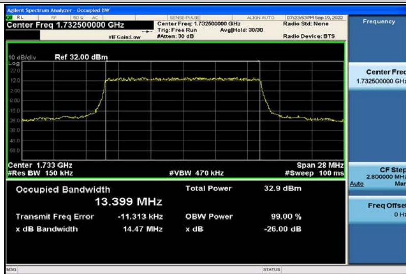
Band4-15MHz-QPSK-20175-75RB#0-13.399
