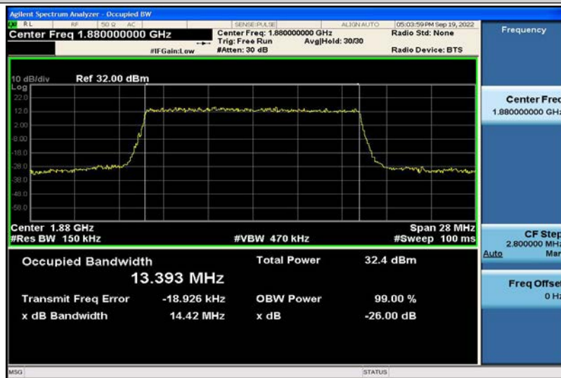
Band2-15MHz-QPSK-18900-75RB#0-13.393
