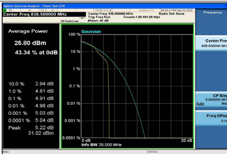
Band5-1.4MHz-16QAM-20525-1RB#0
