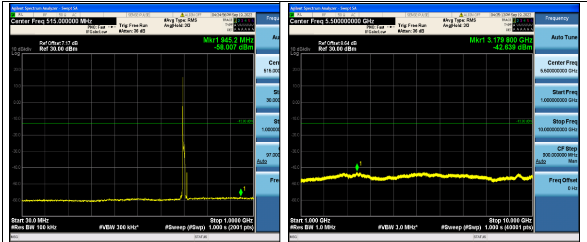
Band12_10MHz_16QAM_23095_1RB#0_30~1000_30~1000
