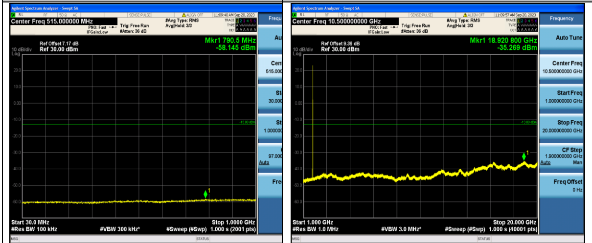
Band66_5MHz_16QAM_132647_1RB#0_30~1000_30~1000
