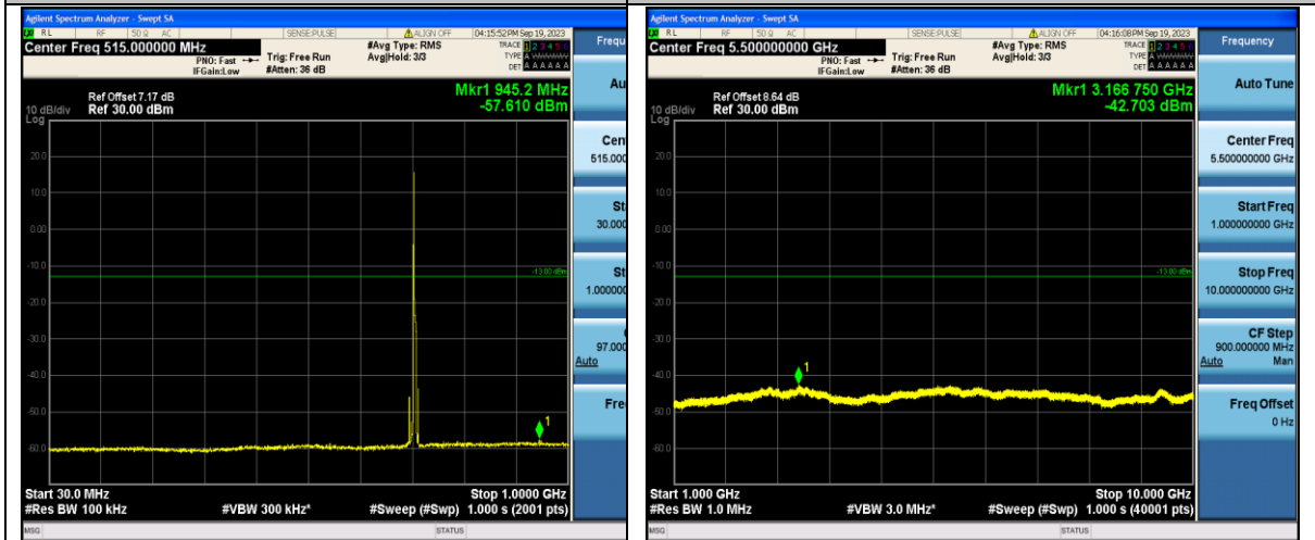
Band12_5MHz_16QAM_23155_1RB#0_30~1000_30~1000
