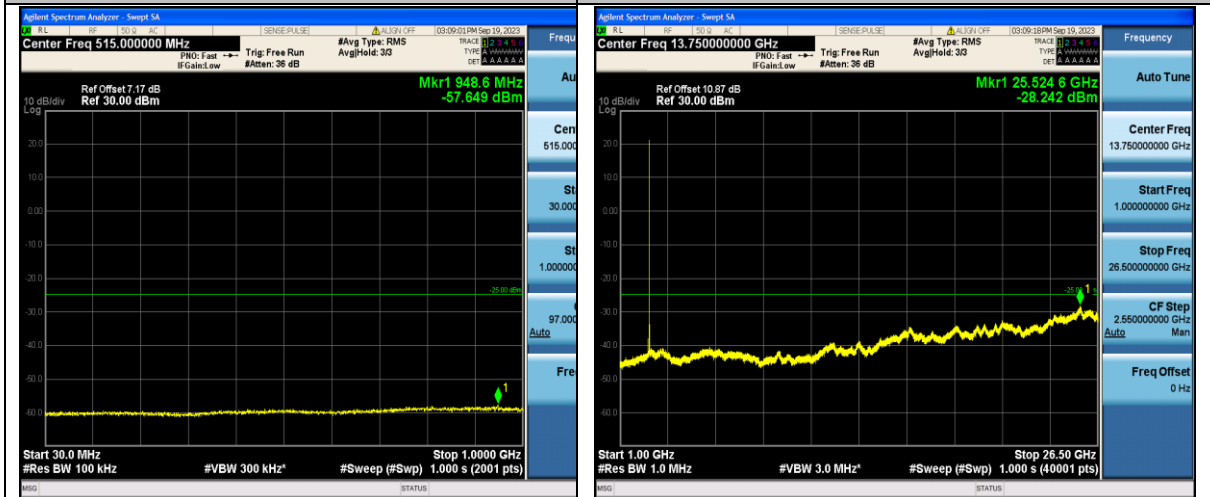
Band7_15MHz_16QAM_21375_1RB#0_30~1000_30~1000
