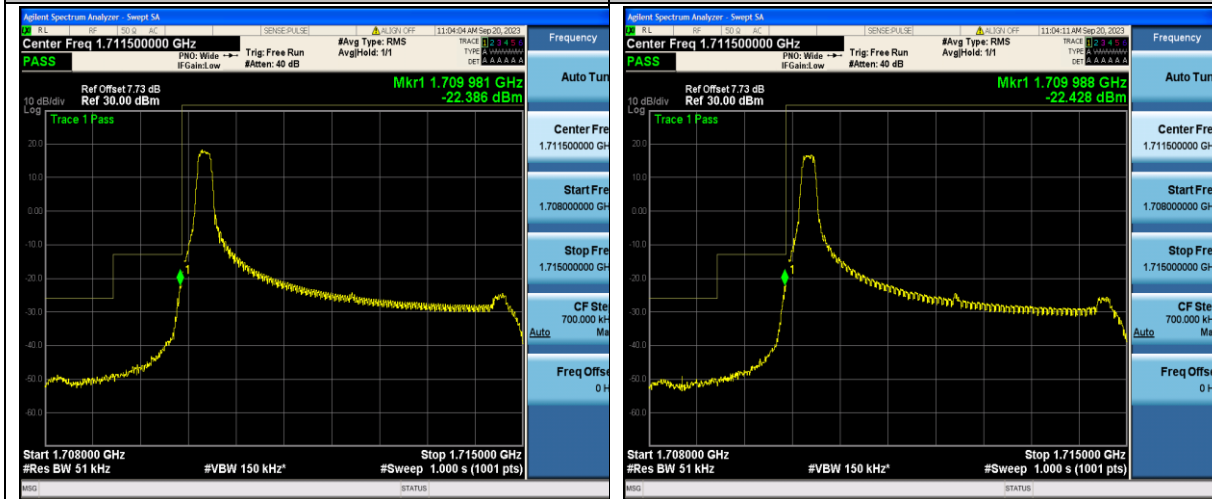
Band66_5MHz_QPSK_131997_1RB#0
