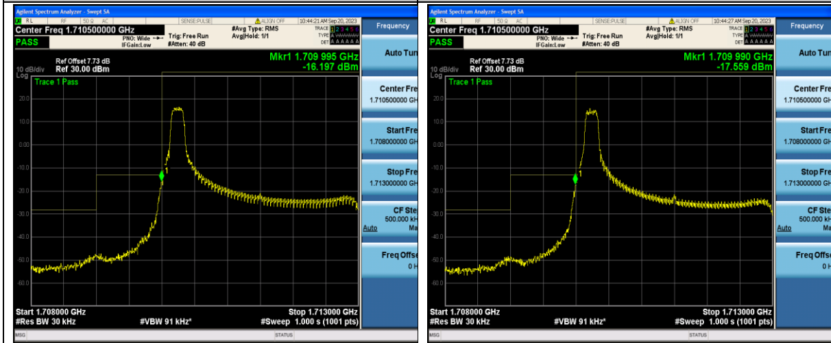
Band66_3MHz_QPSK_131987_1RB#0
