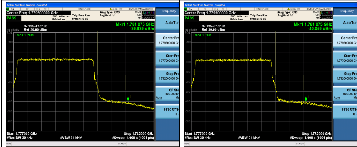
Band66_3MHz_QPSK_132657_15RB#0
