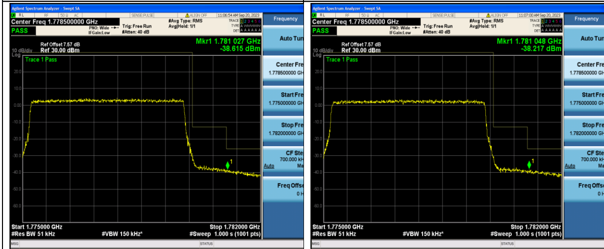
Band66_5MHz_QPSK_132647_25RB#0
