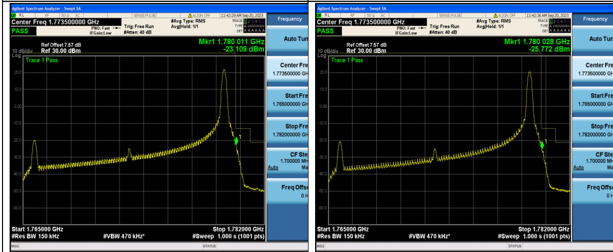
Band66_15MHz_QPSK_132597_1RB#74
