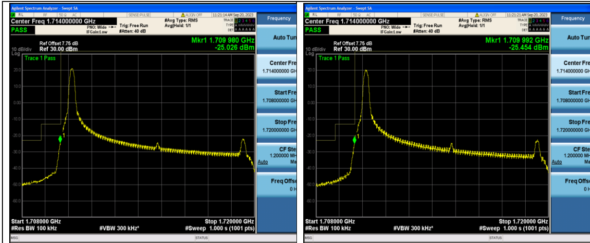
Band66_10MHz_QPSK_132022_1RB#0
