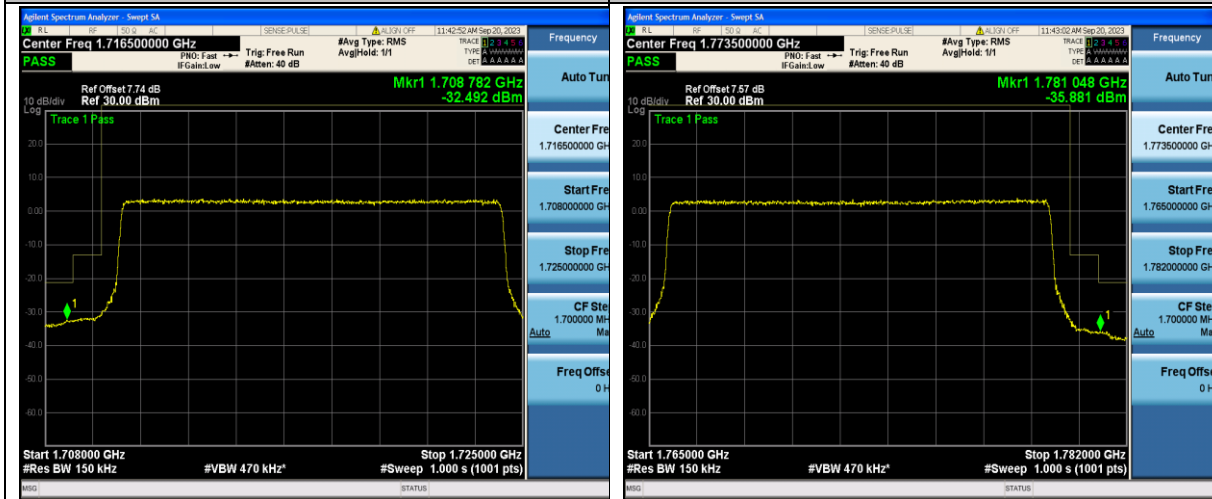
Band66_15MHz_QPSK_132047_75RB#0
