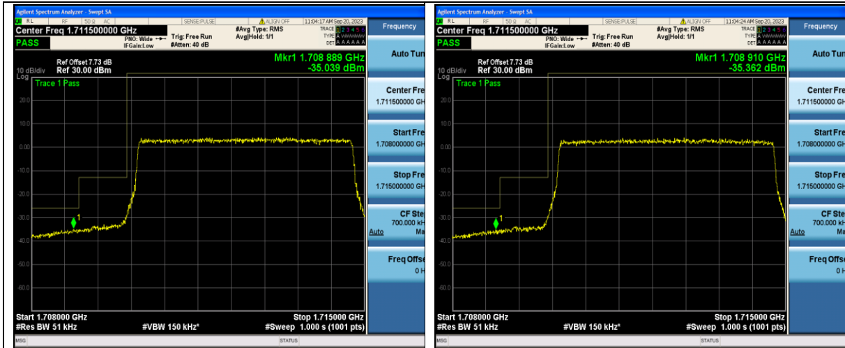
Band66_5MHz_QPSK_131997_25RB#0
