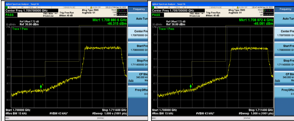
Band66_1.4MHz_QPSK_131979_6RB#0
