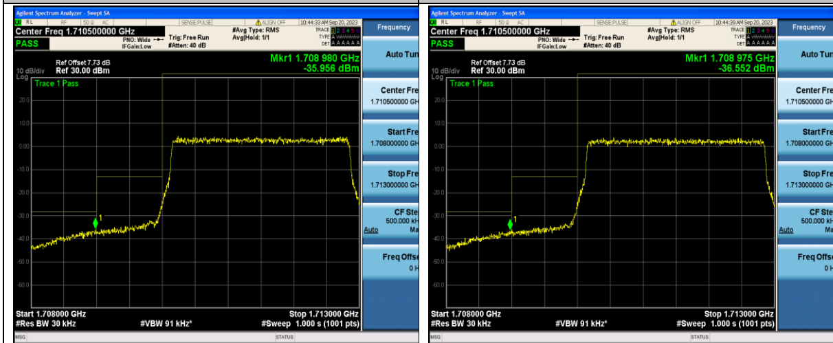
Band66_3MHz_QPSK_131987_15RB#0
