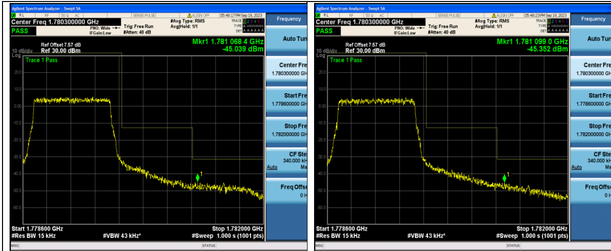
Band66_1.4MHz_QPSK_132665_6RB#0
