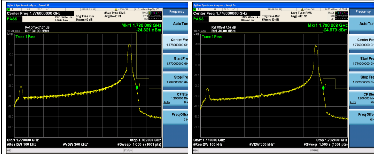
Band66_10MHz_QPSK_132622_1RB#49
