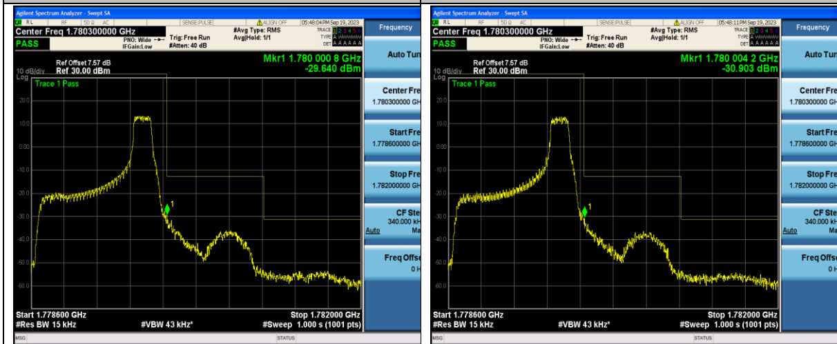
Band66_1.4MHz_QPSK_132665_1RB#5
