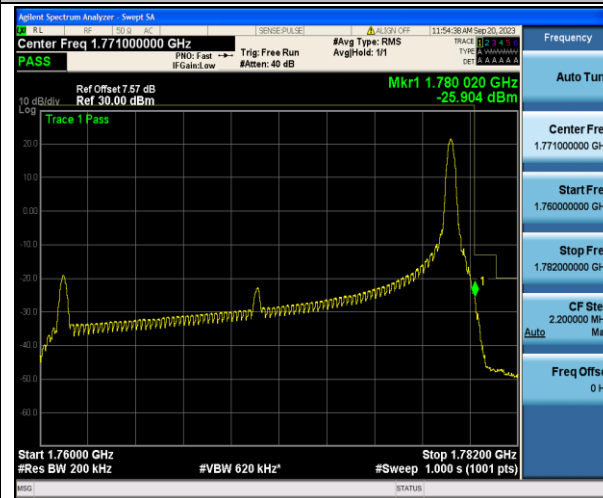
Band66_20MHz_16QAM_132572_1RB#99
