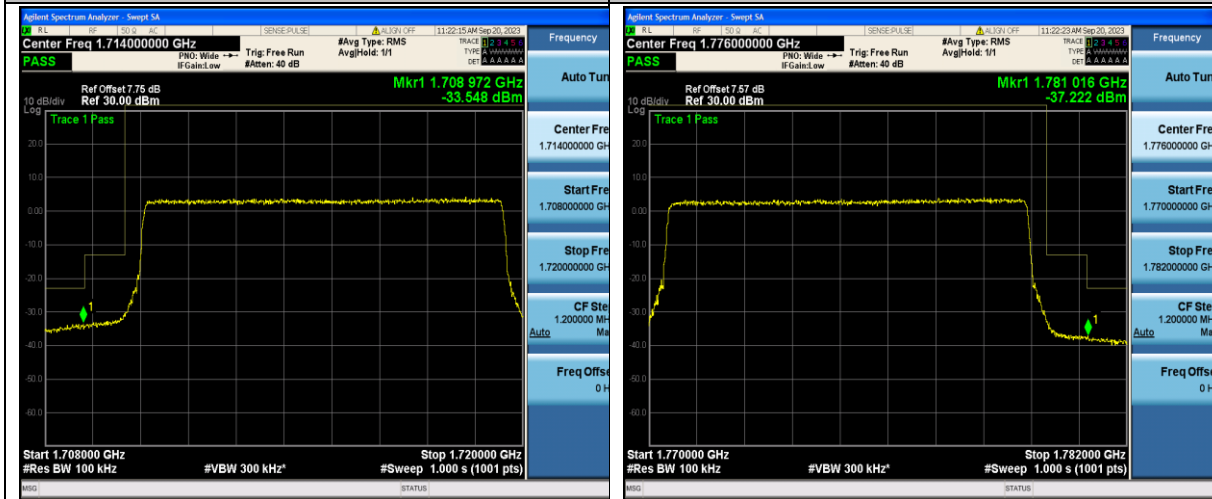
Band66_10MHz_QPSK_132022_50RB#0
