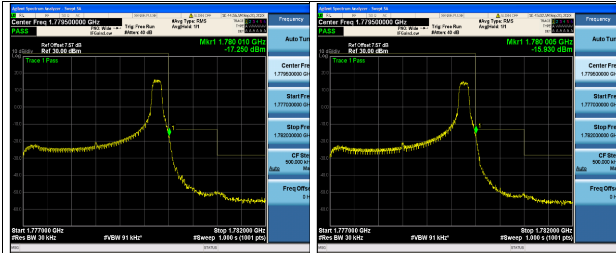
Band66_3MHz_QPSK_132657_1RB#14
