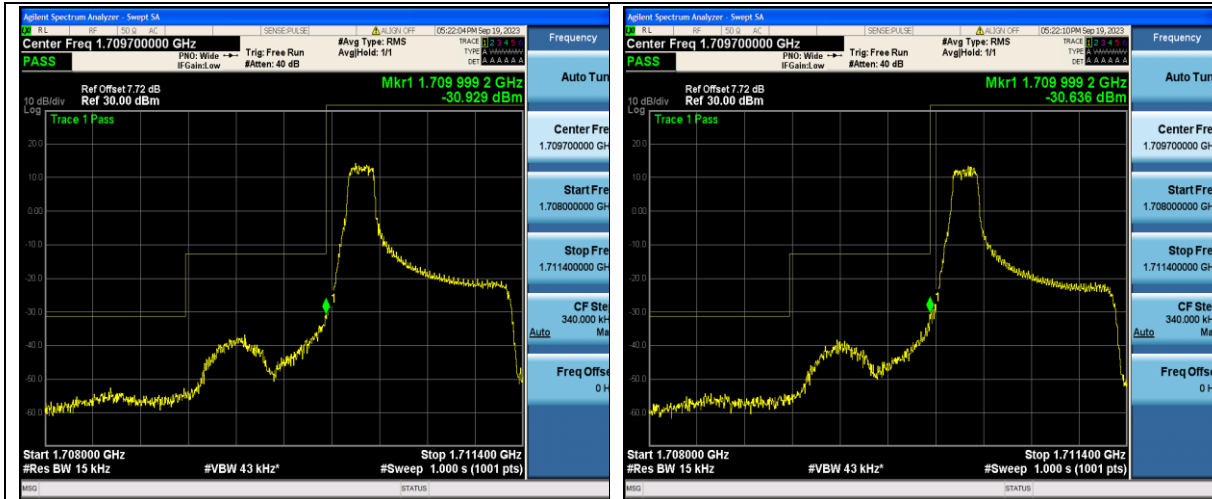
Band66_1.4MHz_QPSK_131979_1RB#0
