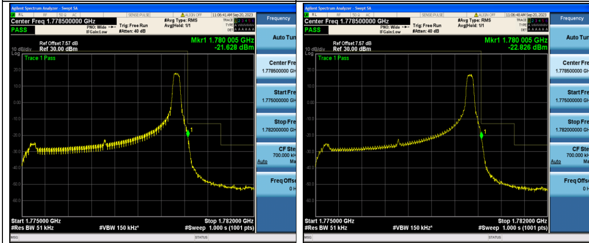
Band66_5MHz_QPSK_132647_1RB#24
