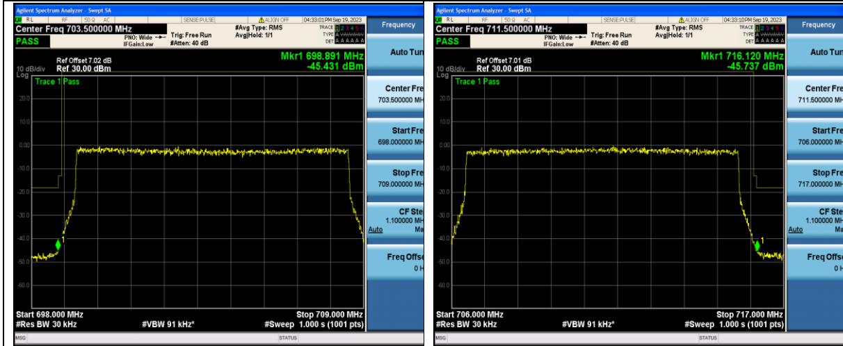
Band12_10MHz_QPSK_23060_50RB#0
