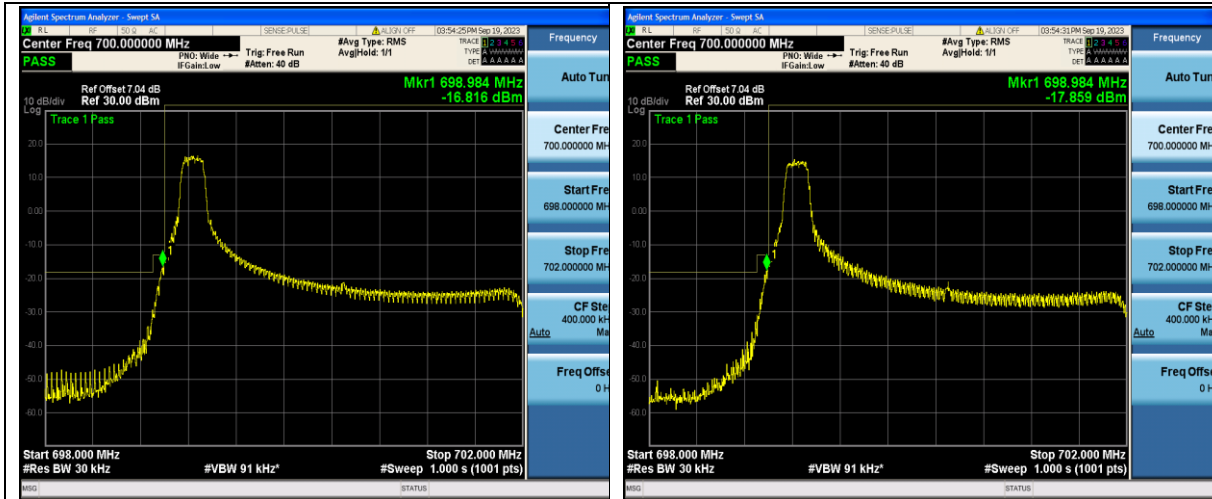
Band12_3MHz_QPSK_23025_1RB#0
