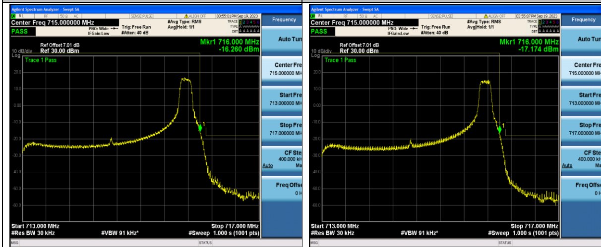
Band12_3MHz_QPSK_23165_1RB#14
