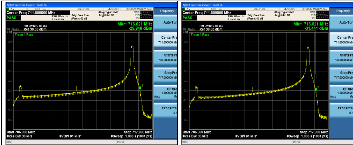
Band12_10MHz_QPSK_23130_1RB#49
