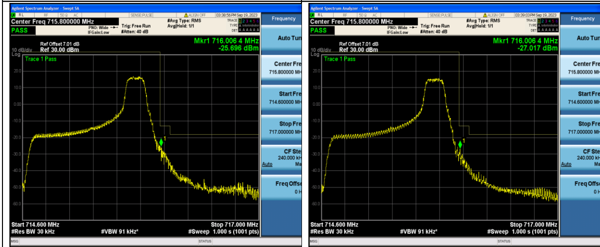
Band12_1.4MHz_QPSK_23173_1RB#5
