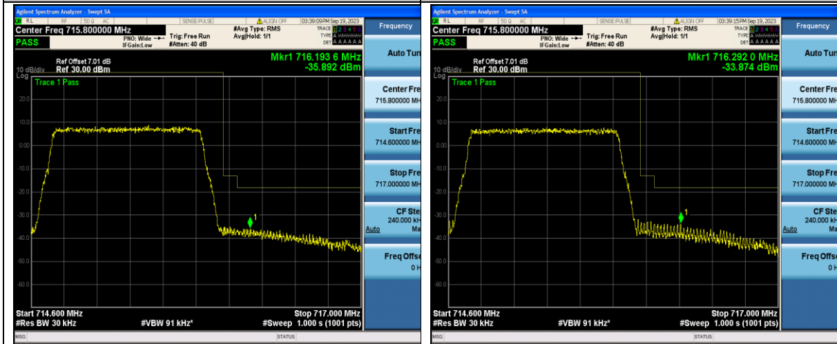
Band12_1.4MHz_QPSK_23173_6RB#0
