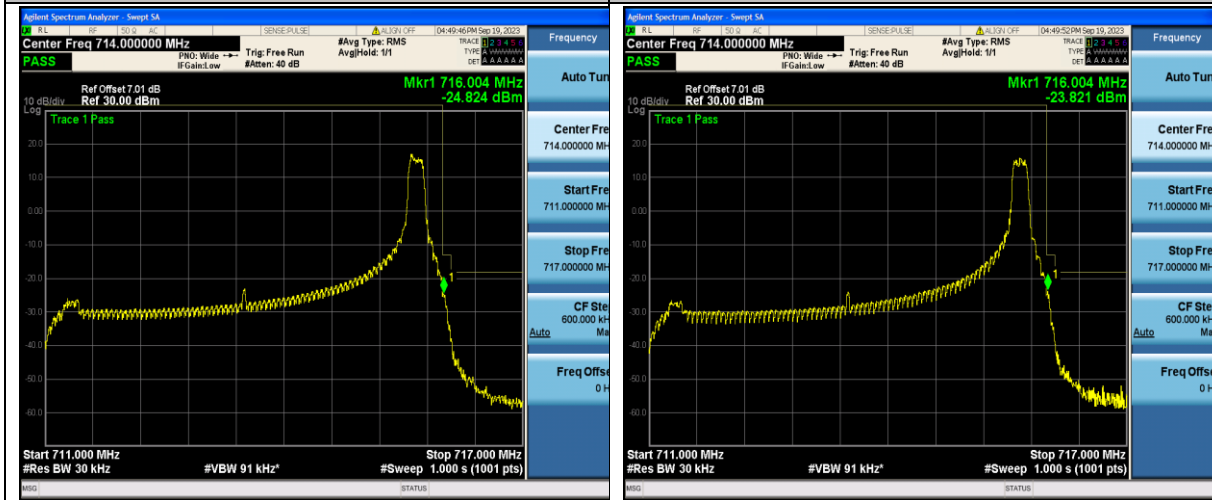
Band17_5MHz_QPSK_23825_1RB#24
