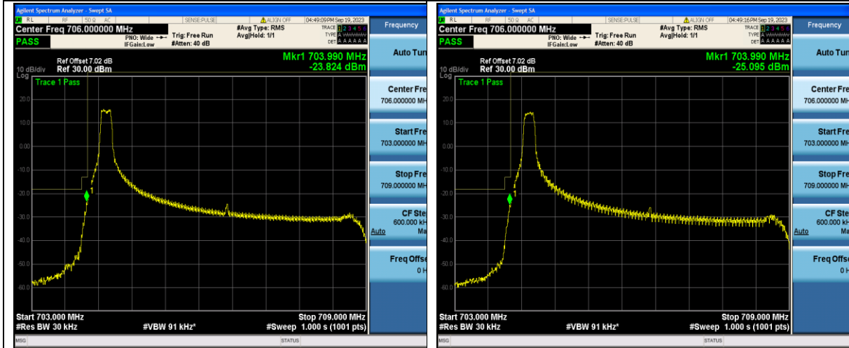
Band17_5MHz_QPSK_23755_1RB#0
