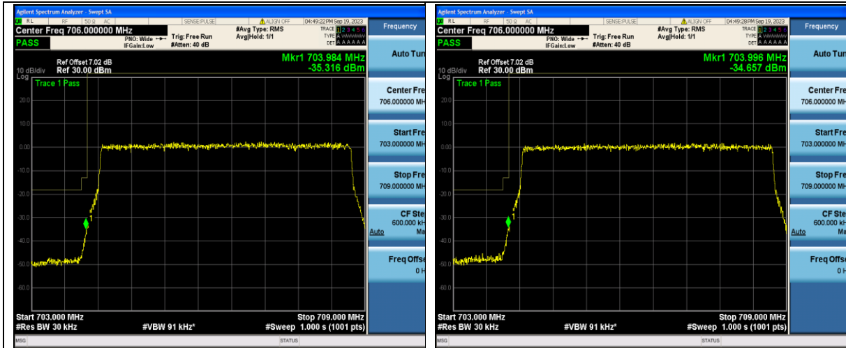
Band17_5MHz_QPSK_23755_25RB#0
