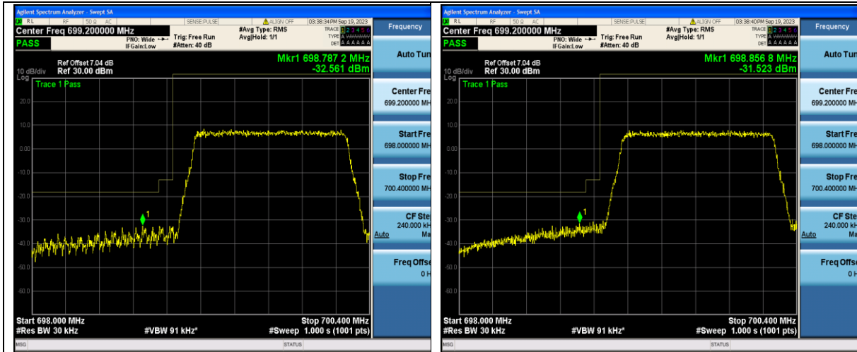
Band12_1.4MHz_QPSK_23017_6RB#0
