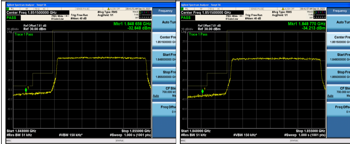
Band2_5MHz_QPSK_18625_25RB#0
