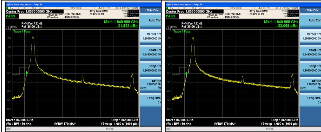
Band2_15MHz_QPSK_18675_1RB#0
