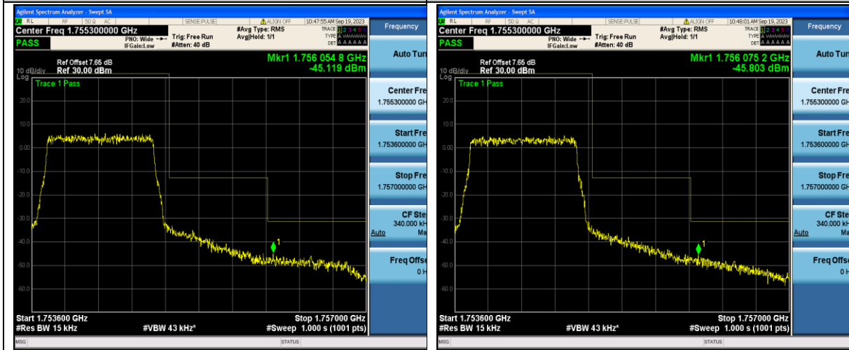
Band4_1.4MHz_QPSK_20393_6RB#0
