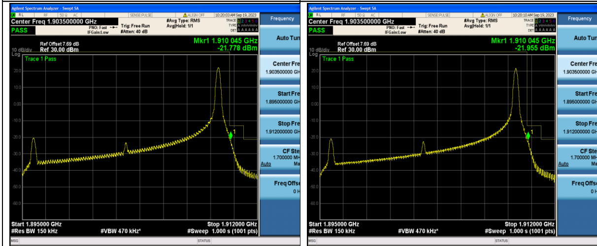
Band2_15MHz_QPSK_19125_1RB#74
