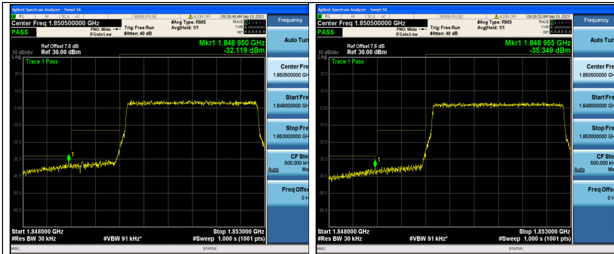
Band2_3MHz_QPSK_18615_15RB#0
