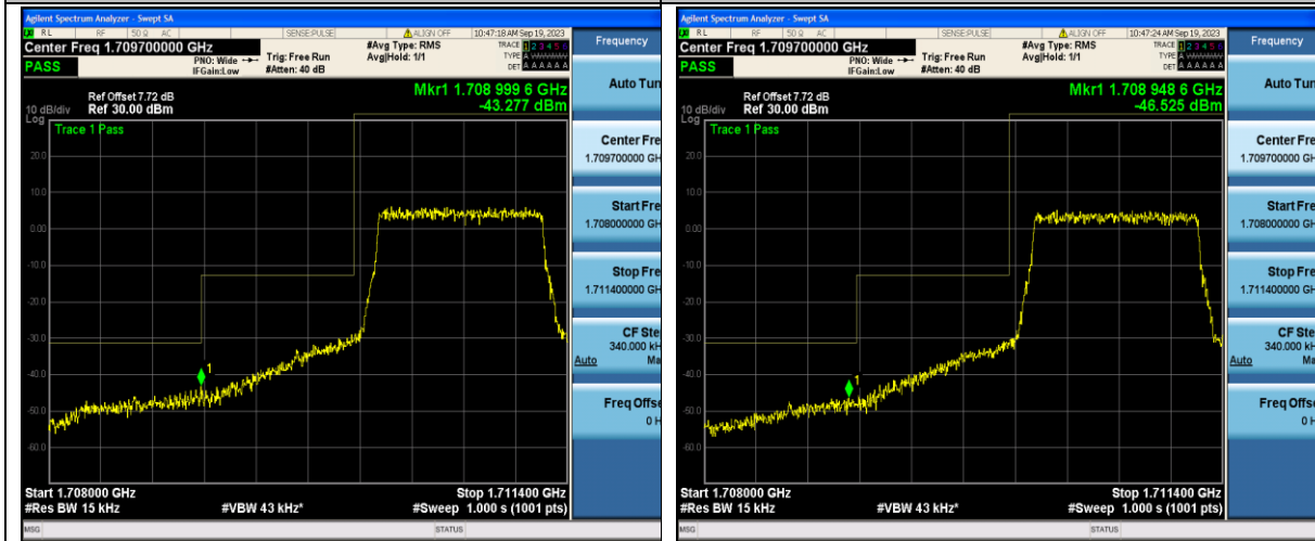
Band4_1.4MHz_QPSK_19957_6RB#0
