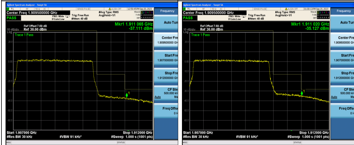
Band2_3MHz_QPSK_19185_15RB#0
