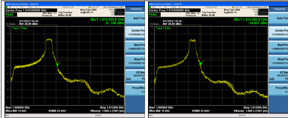
Band2_1.4MHz_QPSK_19193_1RB#5
