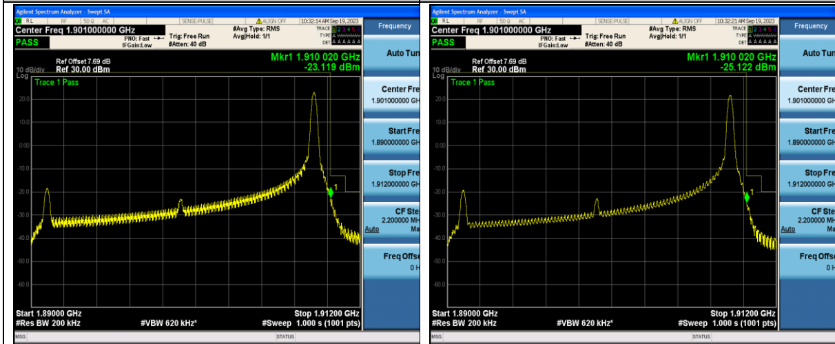
Band2_20MHz_QPSK_19100_1RB#99
