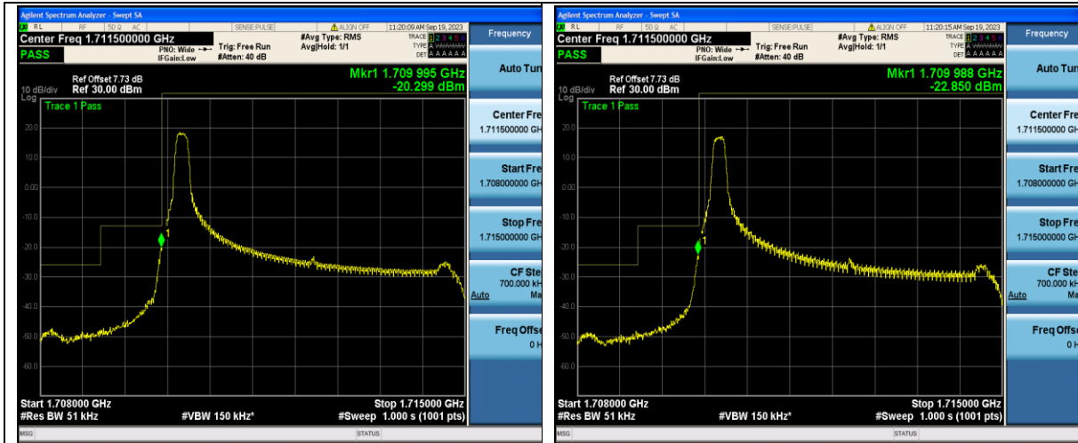
Band4_5MHz_QPSK_19975_1RB#0
