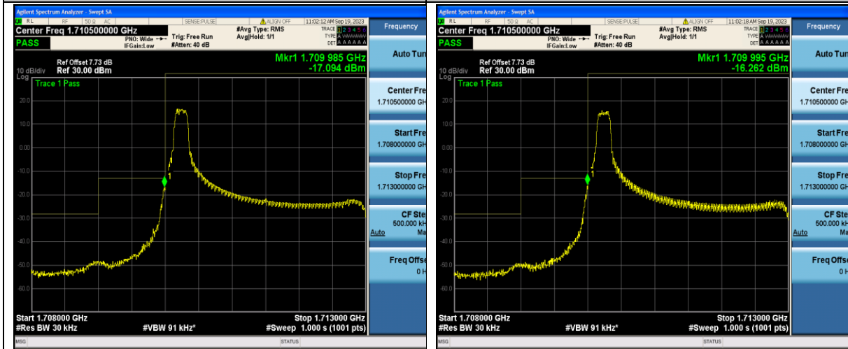
Band4_3MHz_QPSK_19965_1RB#0
