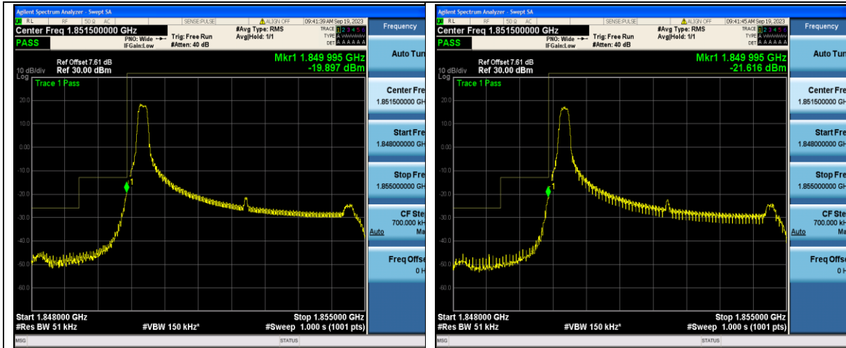
Band2_5MHz_QPSK_18625_1RB#0
