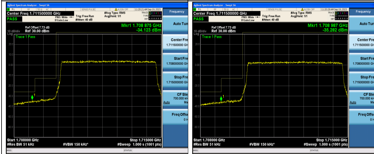
Band4_5MHz_QPSK_19975_25RB#0
