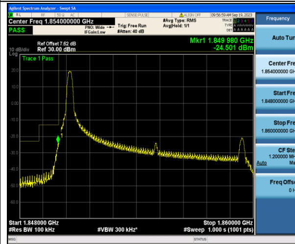
Band2_10MHz_16QAM_18650_1RB#0
