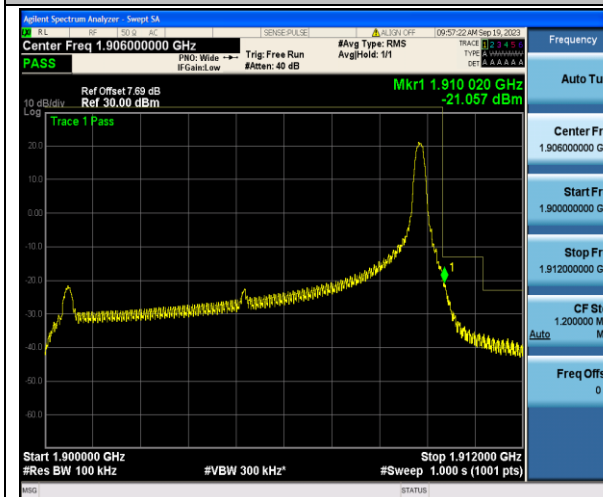
Band2_10MHz_QPSK_19150_1RB#49
