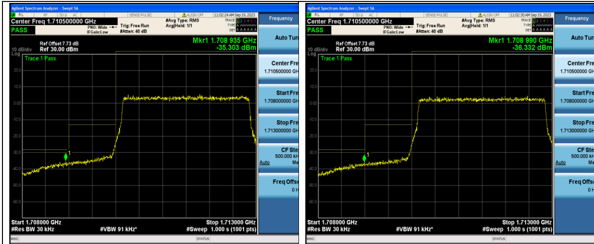
Band4_3MHz_QPSK_19965_15RB#0
