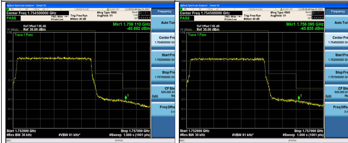
Band4_3MHz_QPSK_20385_15RB#0
