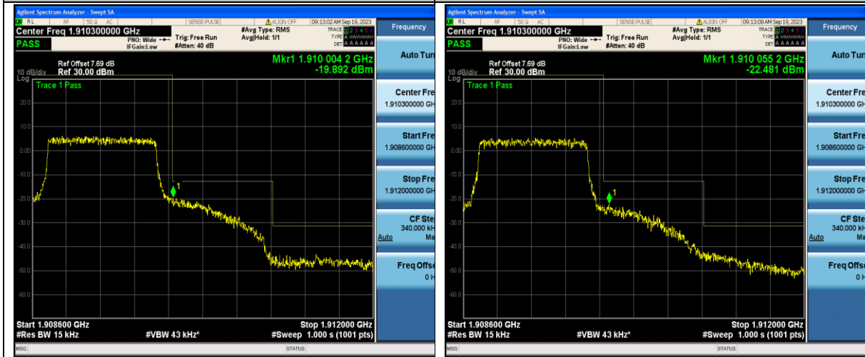
Band2_1.4MHz_QPSK_19193_6RB#0
