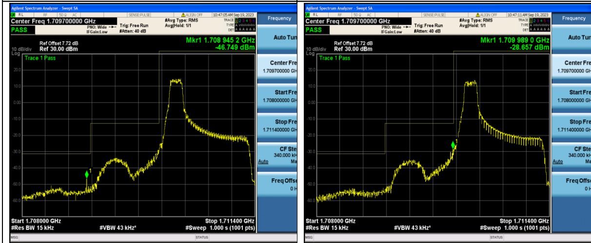
Band4_1.4MHz_QPSK_19957_1RB#0
