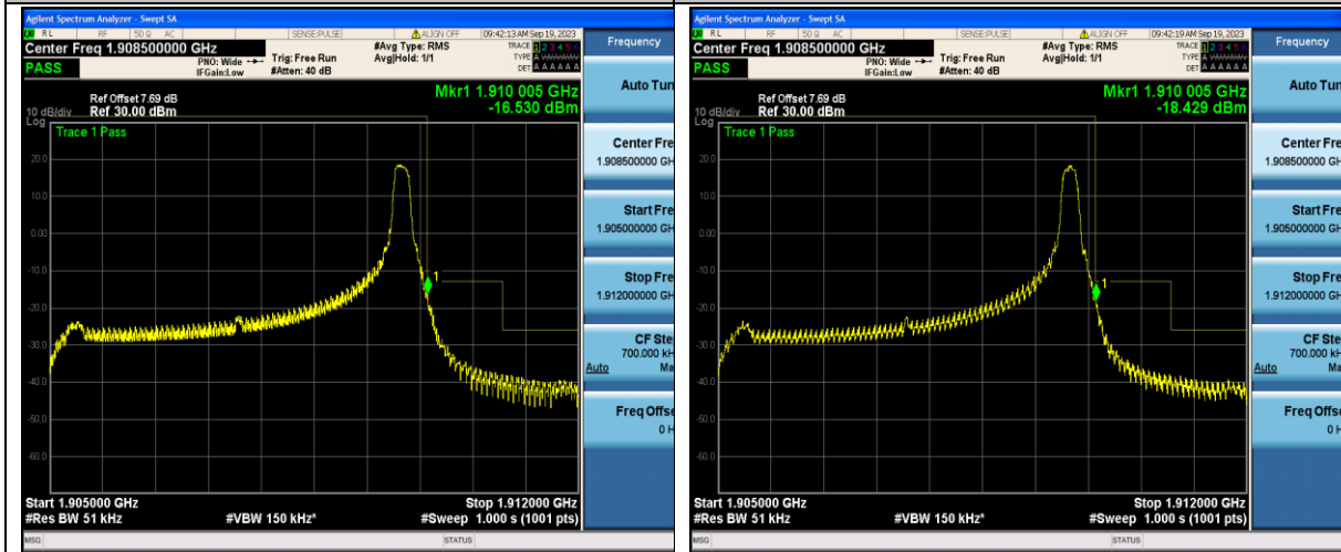
Band2_5MHz_QPSK_19175_1RB#24
