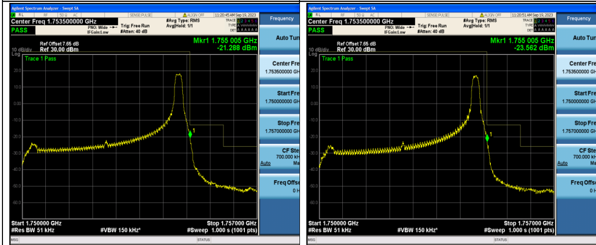
Band4_5MHz_QPSK_20375_1RB#24
