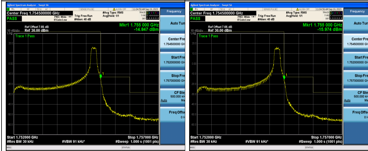
Band4_3MHz_QPSK_20385_1RB#14
