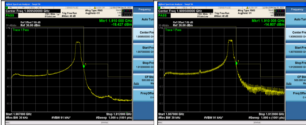
Band2_3MHz_QPSK_19185_1RB#14
