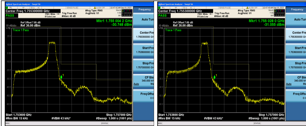
Band4_1.4MHz_QPSK_20393_1RB#5
