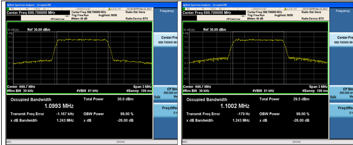
Band12-1.4MHz-QPSK-23017-6RB#0-PASS
