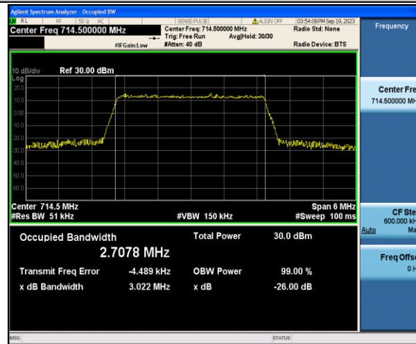
Band12-3MHz-16QAM-23165-15RB#0-PASS
