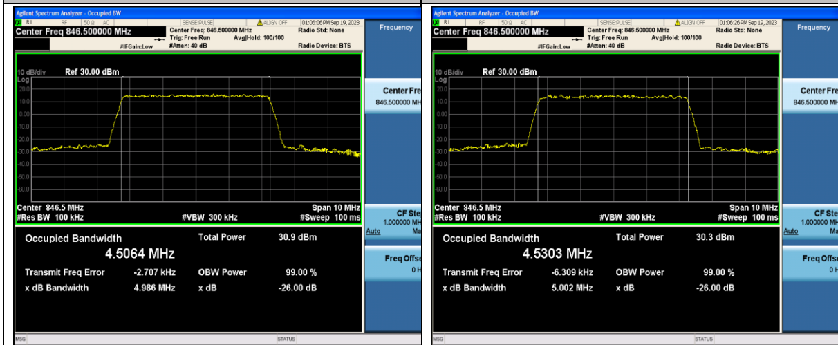
Band5-5MHz-QPSK-20625-25RB#0-PASS
