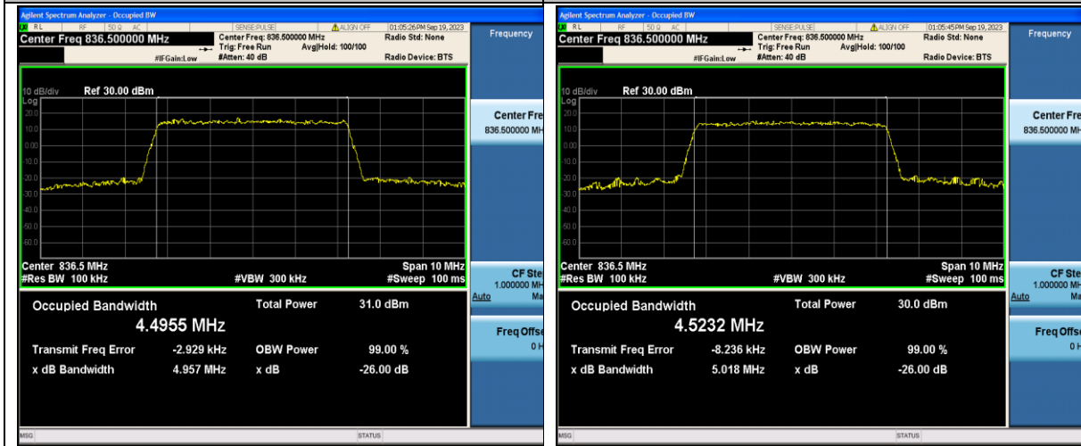
Band5-5MHz-QPSK-20525-25RB#0-PASS
