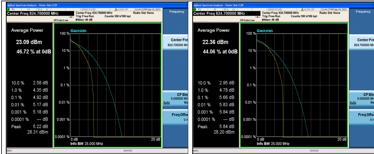
Band5-1.4MHz-QPSK-20407-1RB#0-PASS
