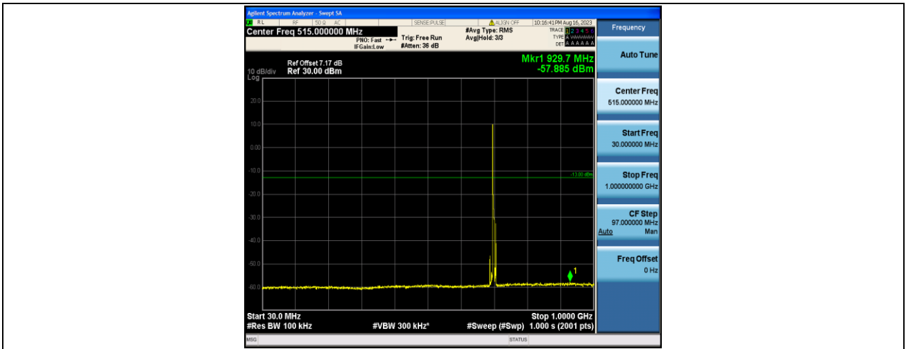
Band17_5MHz_QPSK_23755_1RB#0_30~1000_30~1000
