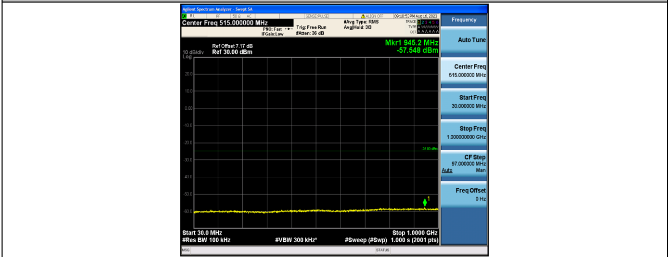
Band7_5MHz_QPSK_21425_1RB#0_30~1000_30~1000
