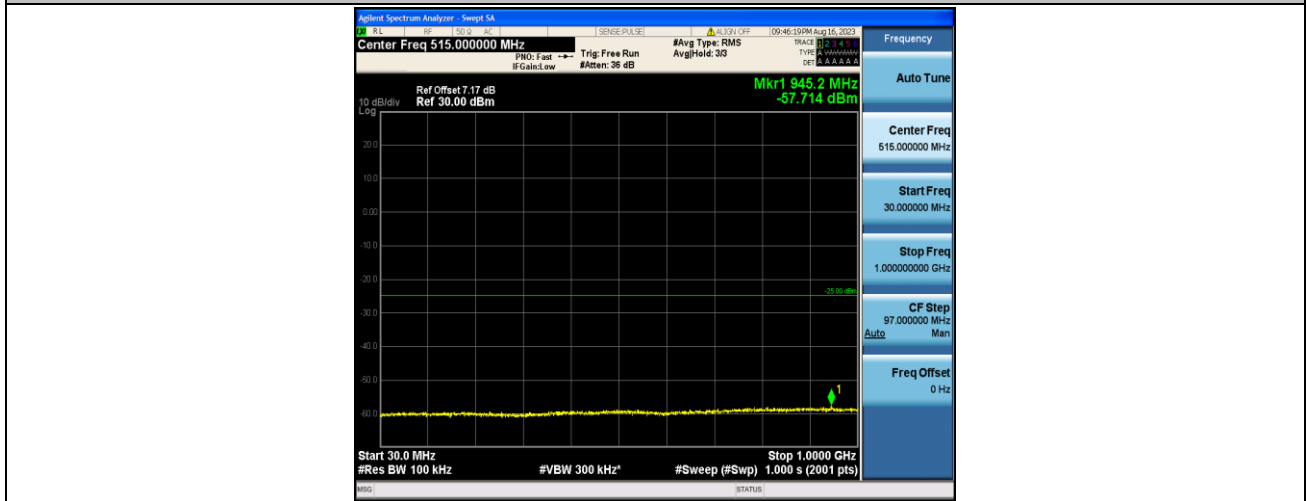
Band7_15MHz_QPSK_21375_1RB#0_30~1000_30~1000
