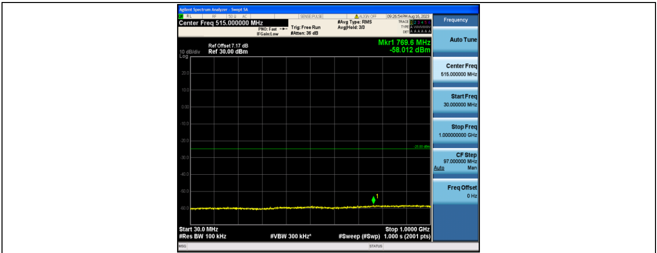
Band7_10MHz_QPSK_20800_1RB#0_30~1000_30~1000
