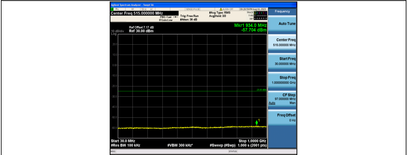
Band7_10MHz_QPSK_21400_1RB#0_30~1000_30~1000
