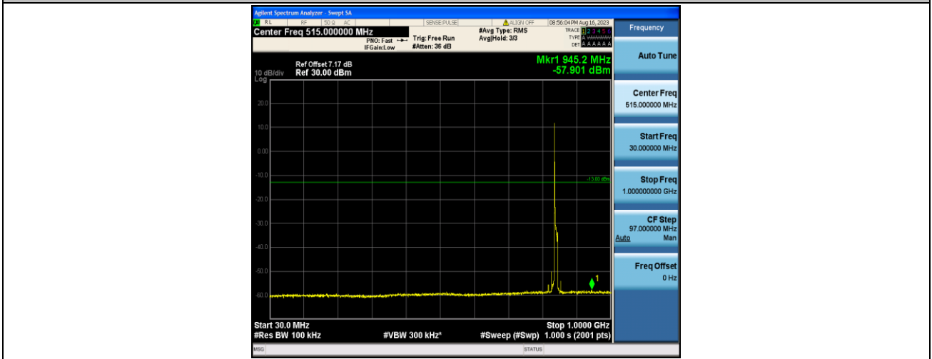
Band5_10MHz_QPSK_20600_1RB#0_30~1000_30~1000
