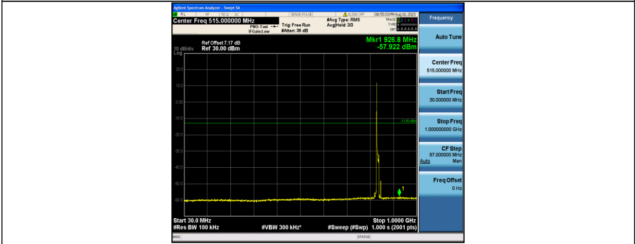
Band5_10MHz_QPSK_20525_1RB#0_30~1000_30~1000
