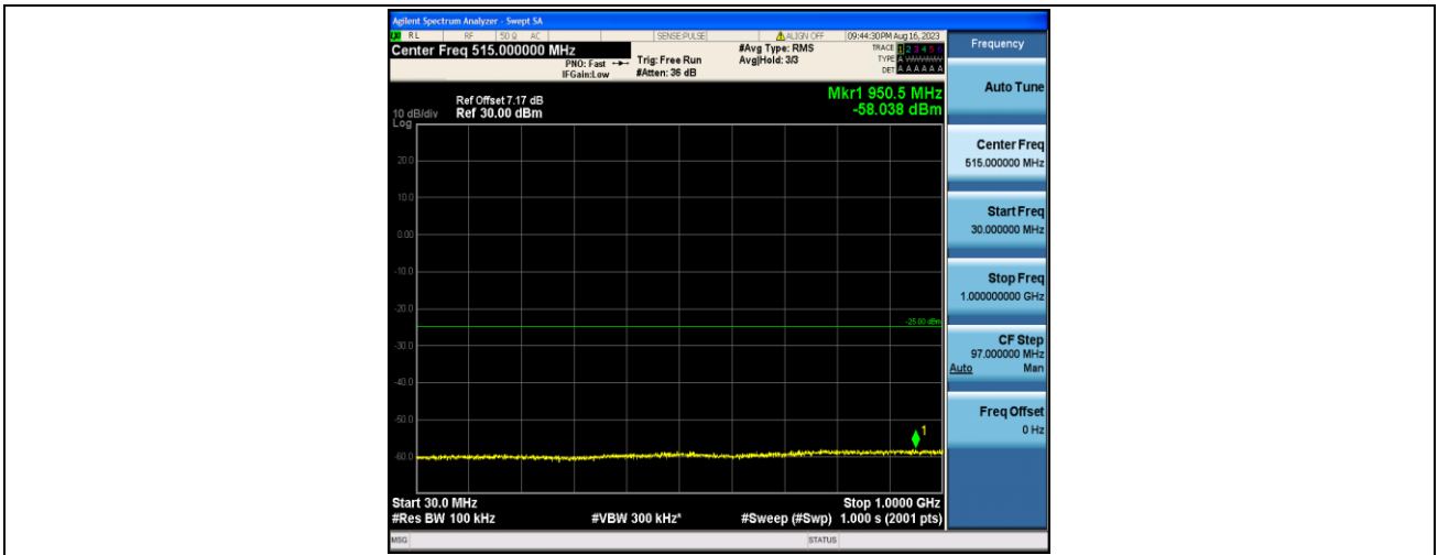
Band7_15MHz_QPSK_20825_1RB#0_30~1000_30~1000
