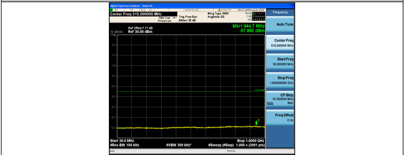
Band7_5MHz_16QAM_21425_1RB#0_30~1000_30~1000
