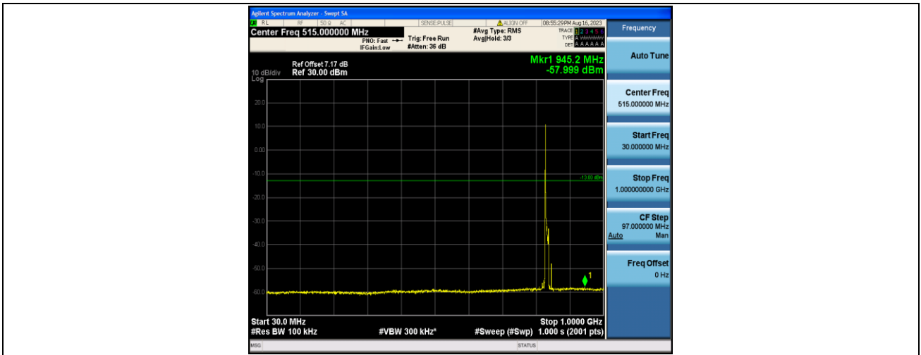
Band5_10MHz_16QAM_20525_1RB#0_30~1000_30~1000
