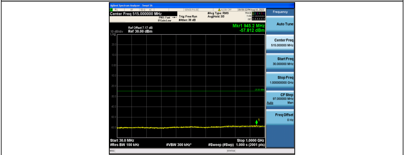
Band7_20MHz_16QAM_20850_1RB#0_30~1000_30~1000
