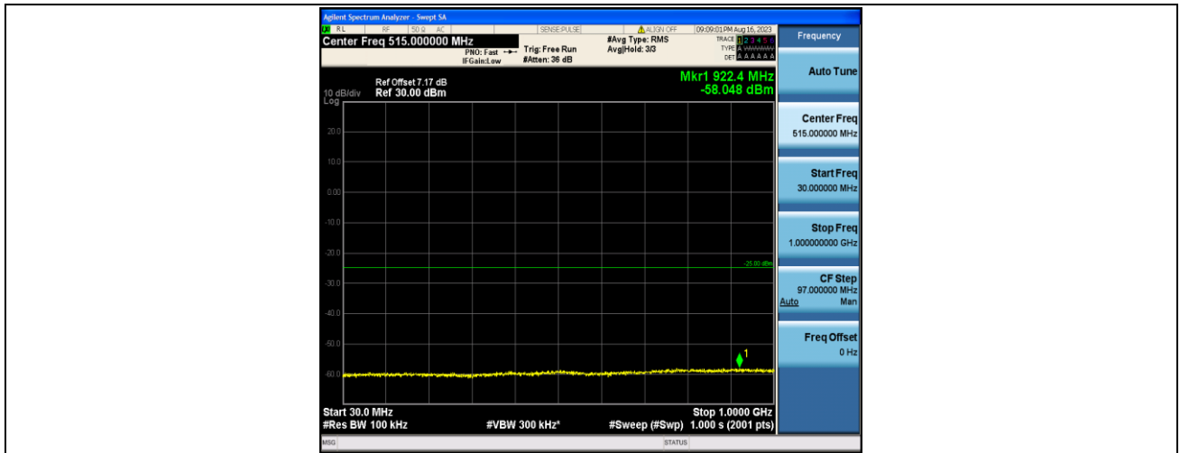
Band7_5MHz_QPSK_20775_1RB#0_30~1000_30~1000
