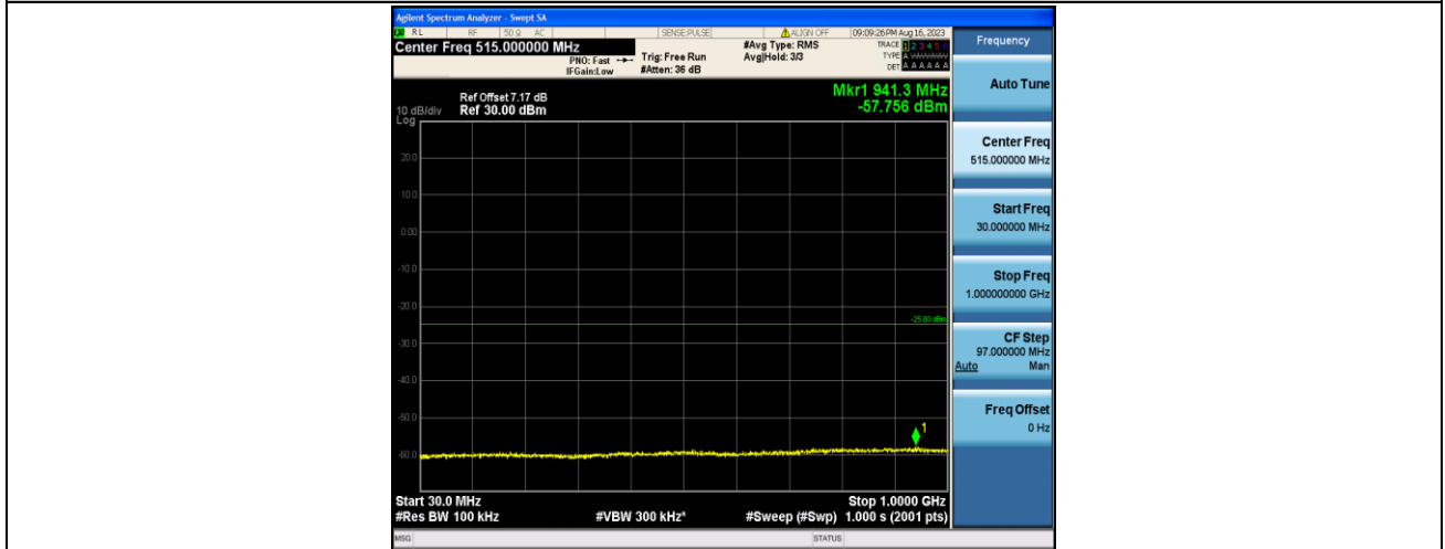
Band7_5MHz_16QAM_20775_1RB#0_30~1000_30~1000
