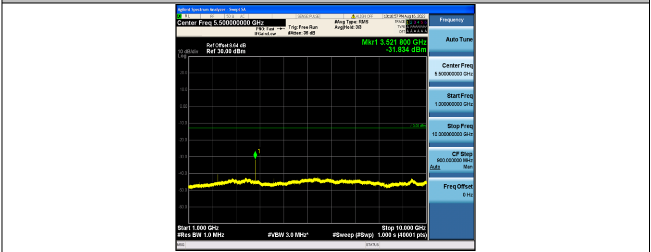
Band17_5MHz_QPSK_23755_1RB#0_1000~10000_1000~10000
