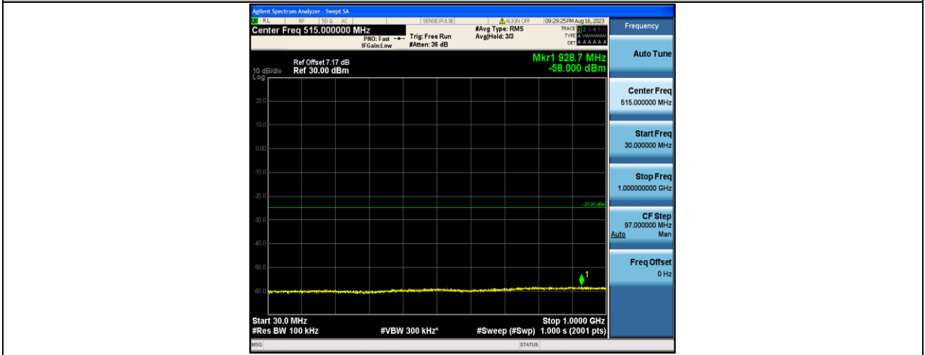
Band7_10MHz_16QAM_21400_1RB#0_30~1000_30~1000
