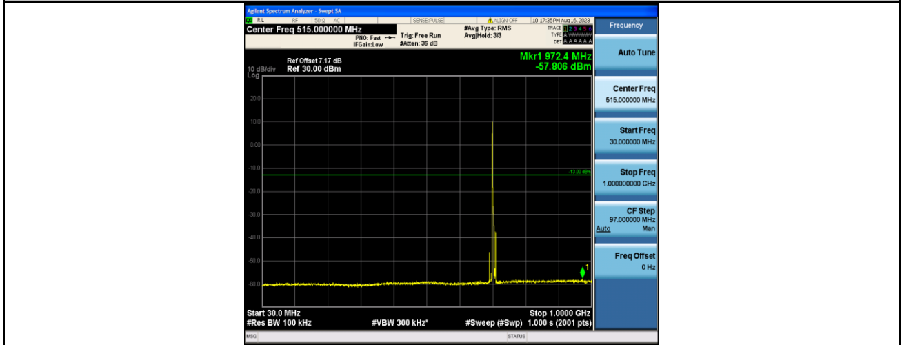
Band17_5MHz_QPSK_23790_1RB#0_30~1000_30~1000
