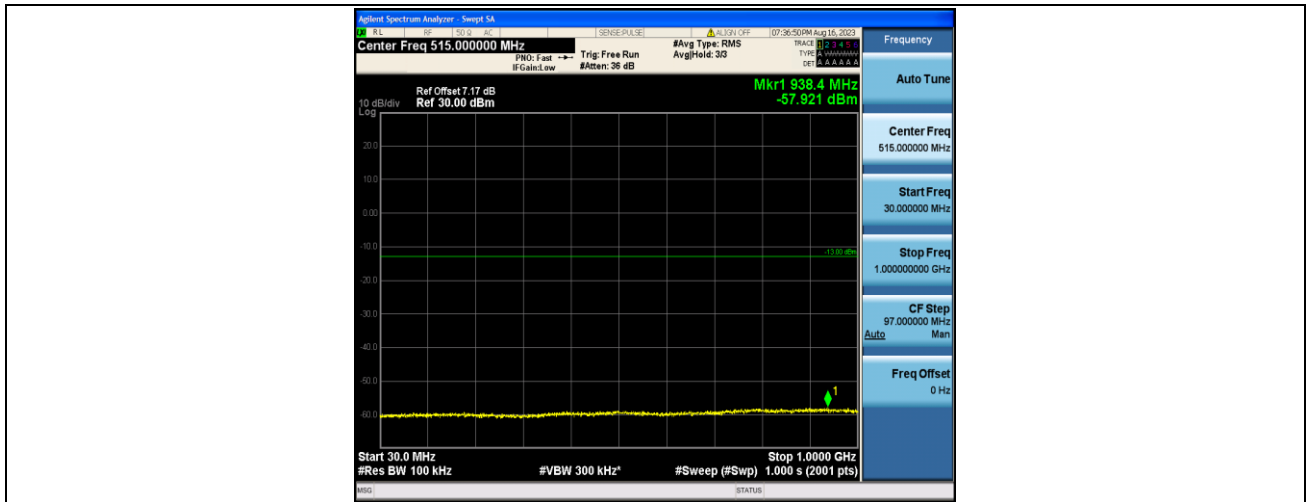
Band4_15MHz_16QAM_20175_1RB#0_30~1000_30~1000
