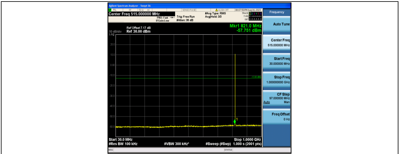
Band5_1.4MHz_QPSK_20407_1RB#0_30~1000_30~1000
