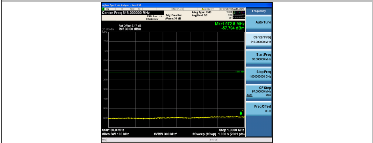
Band4_15MHz_QPSK_20325_1RB#0_30~1000_30~1000
