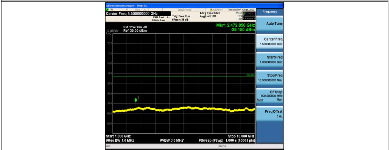
Band5_1.4MHz_QPSK_20407_1RB#0_1000~10000_1000~10000
