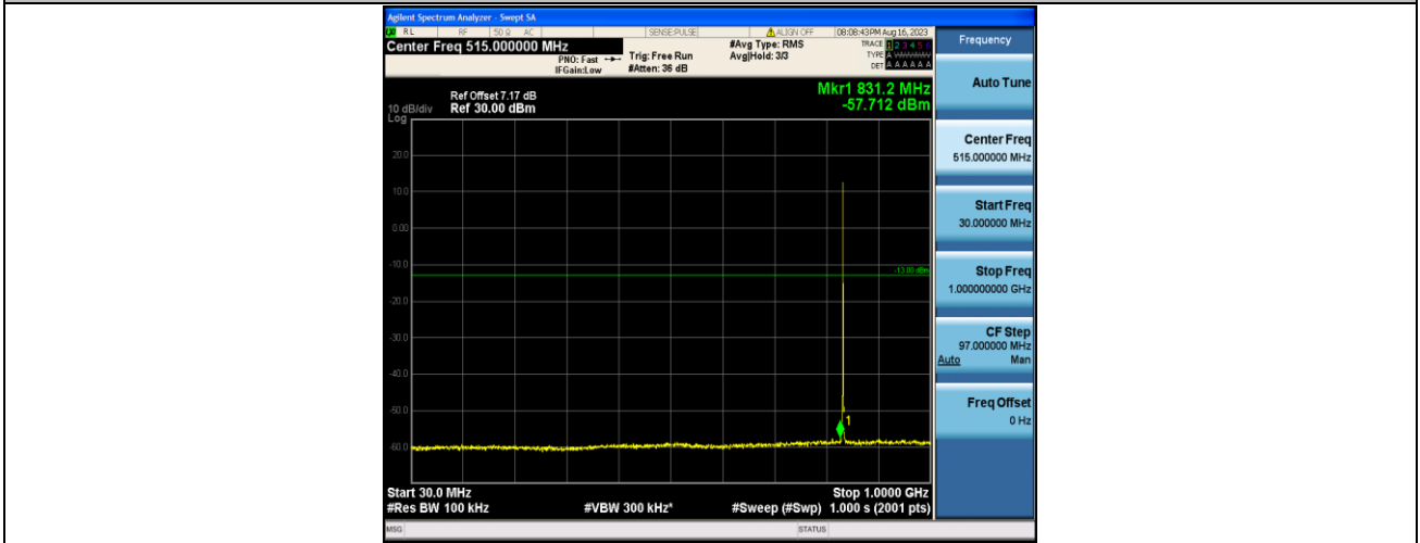
Band5_1.4MHz_QPSK_20525_1RB#0_30~1000_30~1000
