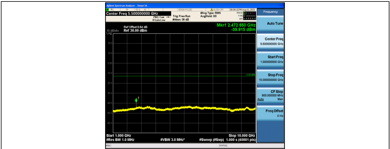
Band5_1.4MHz_16QAM_20407_1RB#0_1000~10000_1000~10000
