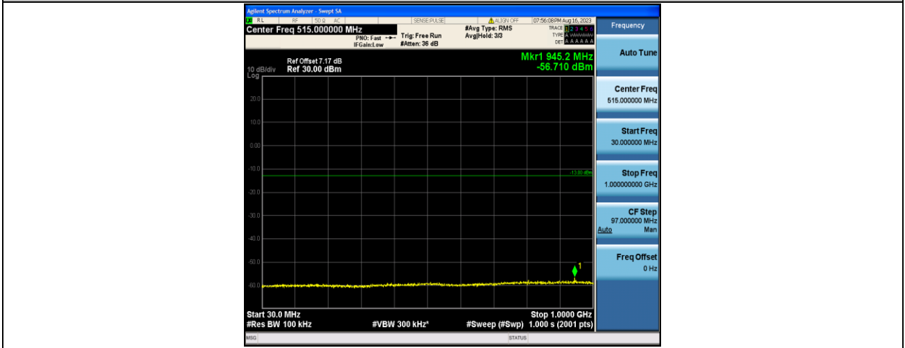
Band4_20MHz_16QAM_20300_1RB#0_30~1000_30~1000
