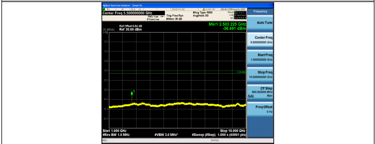
Band5_5MHz_16QAM_20525_1RB#0_1000~10000_1000~10000
