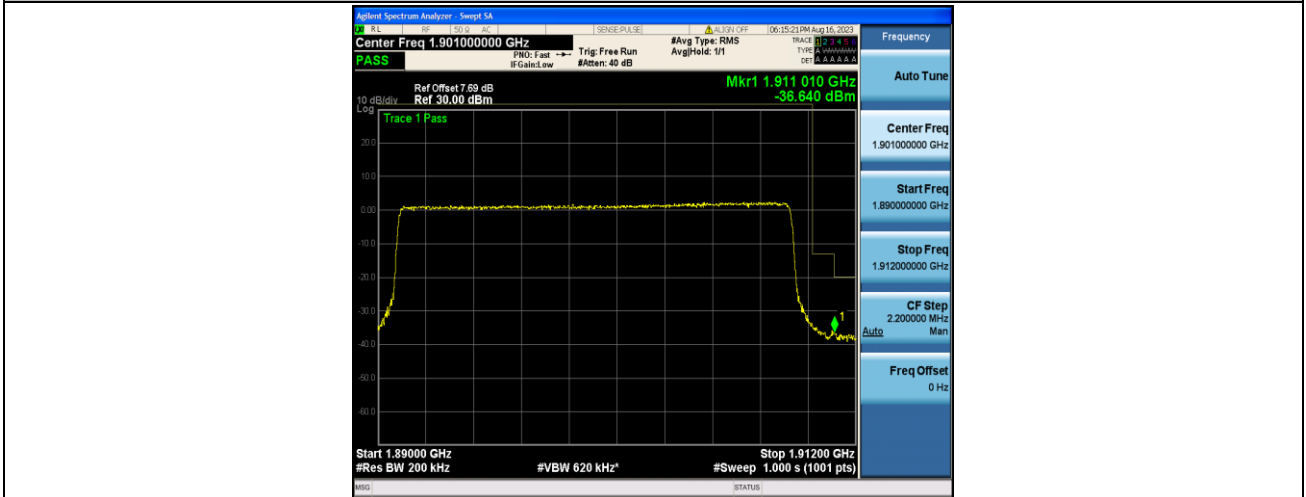
Band2_20MHz_QPSK_19100_100RB#0
