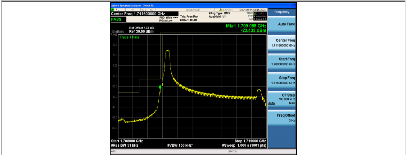
Band4_5MHz_16QAM_19975_1RB#0
