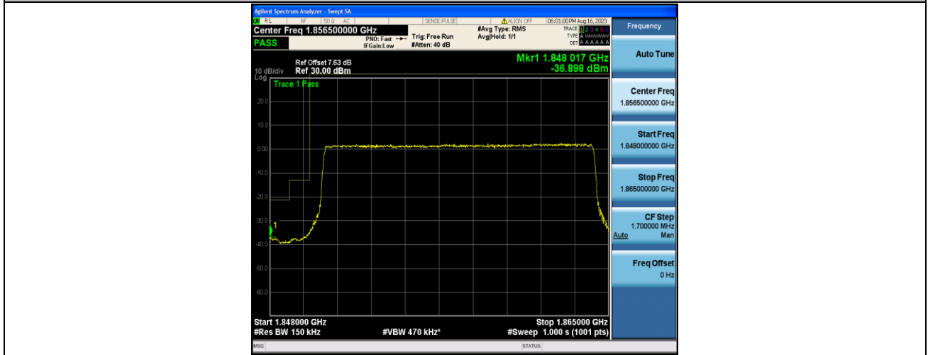
Band2_15MHz_QPSK_18675_75RB#0
