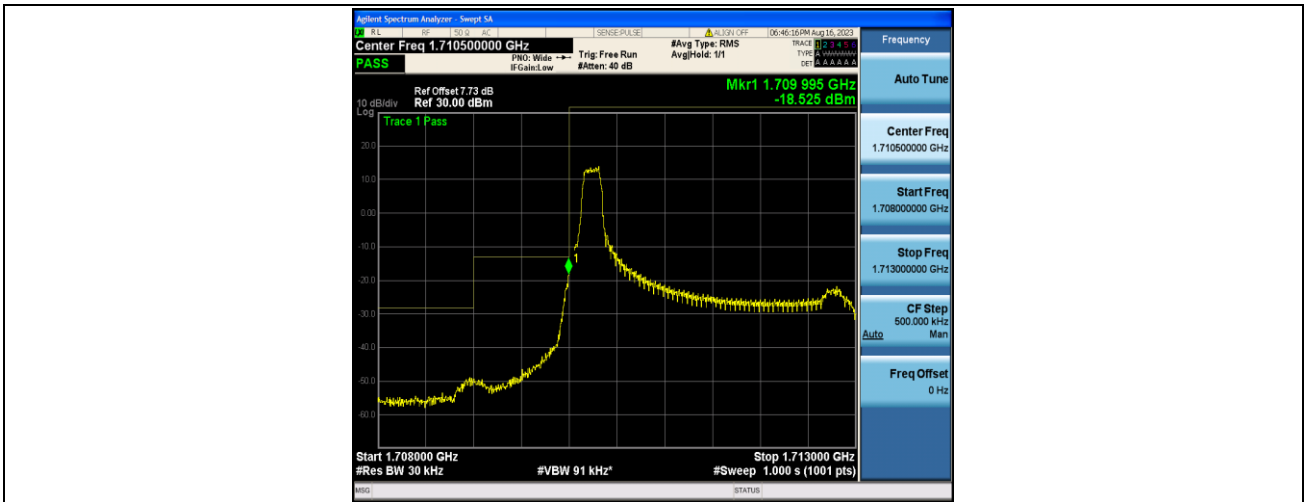
Band4_3MHz_16QAM_19965_1RB#0
