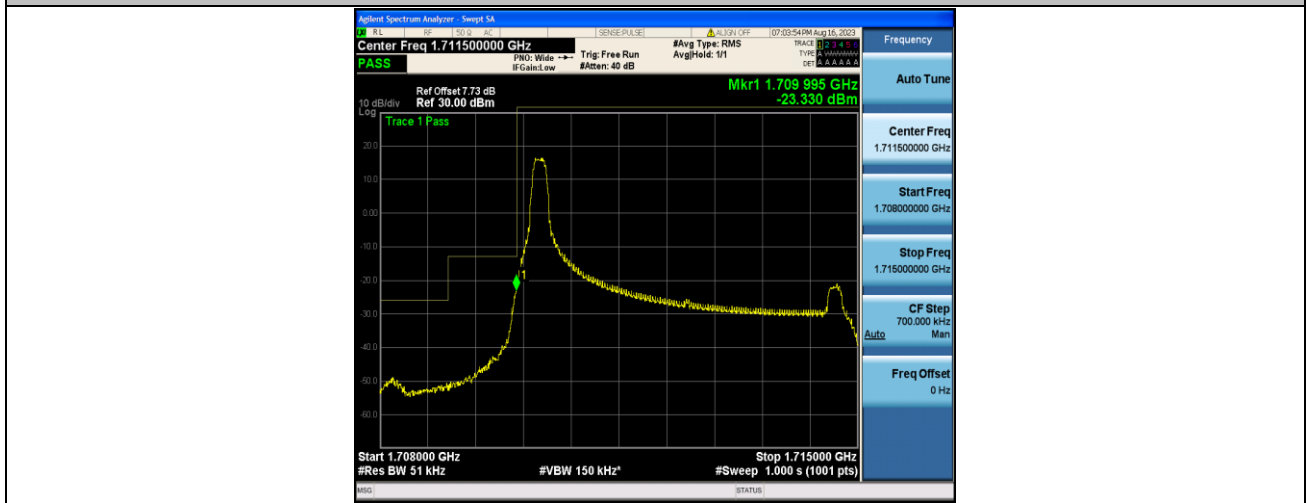
Band4_5MHz_QPSK_19975_1RB#0
