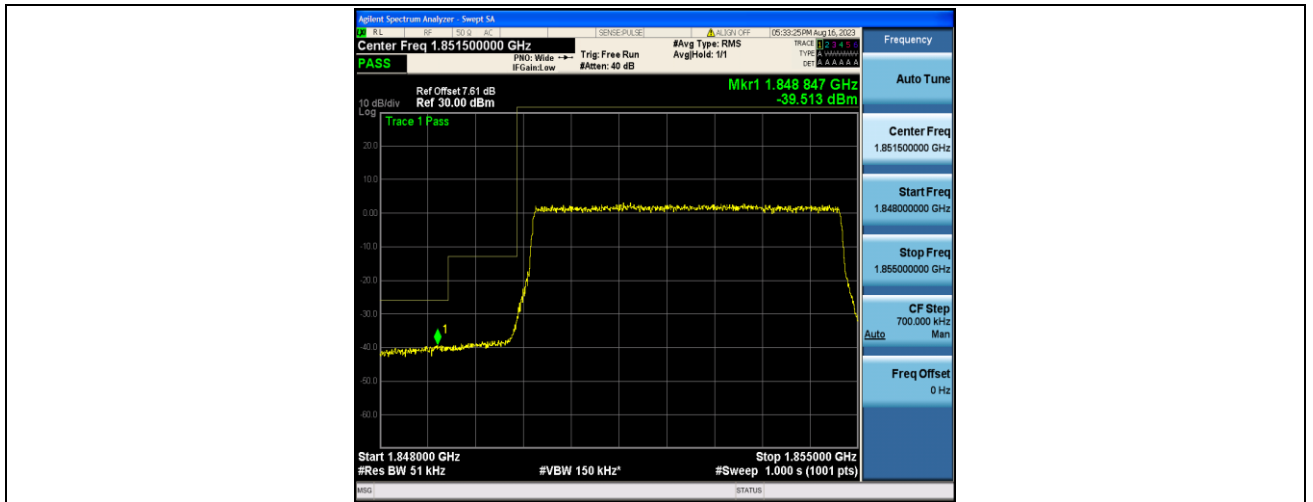
Band2_5MHz_QPSK_18625_25RB#0
