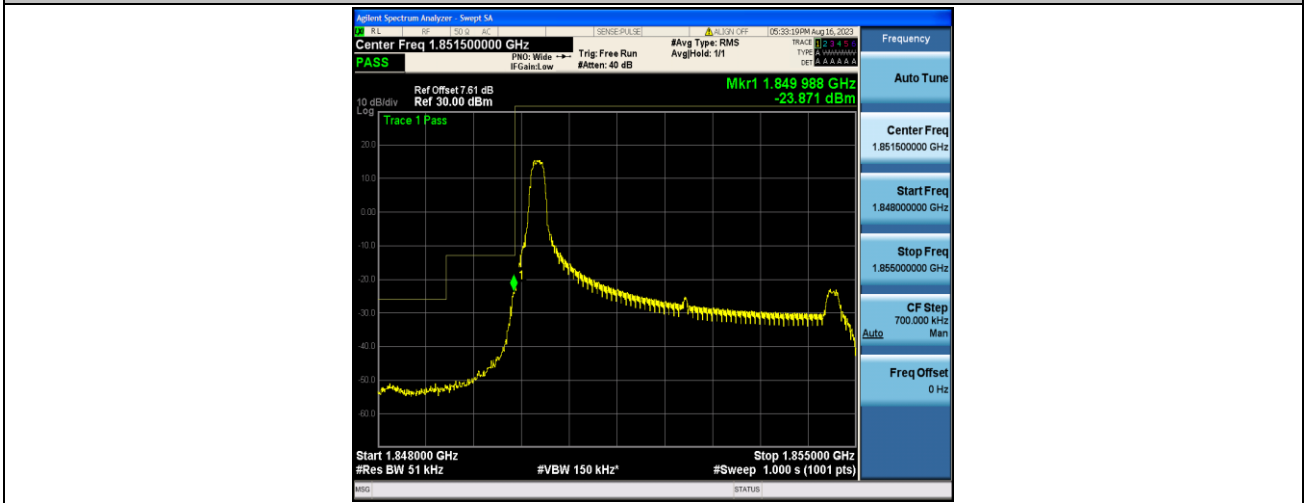
Band2_5MHz_16QAM_18625_1RB#0
