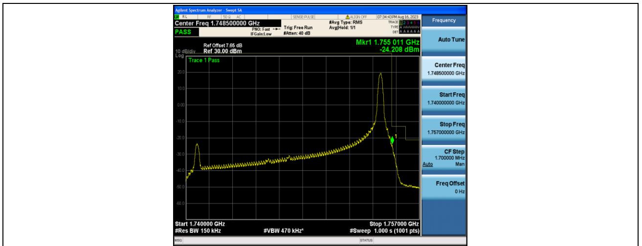
Band4_15MHz_16QAM_20325_1RB#74
