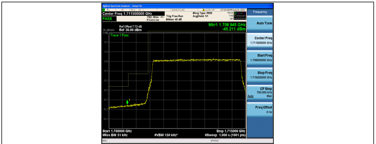
Band4_5MHz_QPSK_19975_25RB#0
