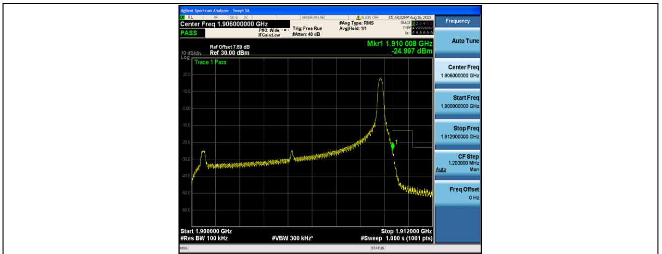
Band2_10MHz_16QAM_19150_1RB#49
