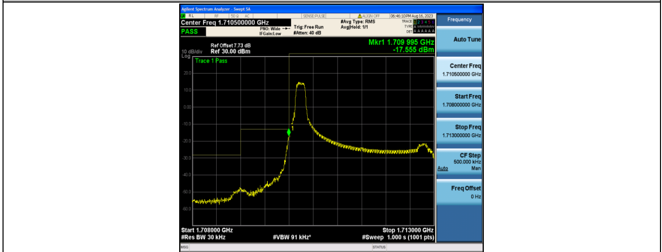
Band4_3MHz_QPSK_19965_1RB#0
