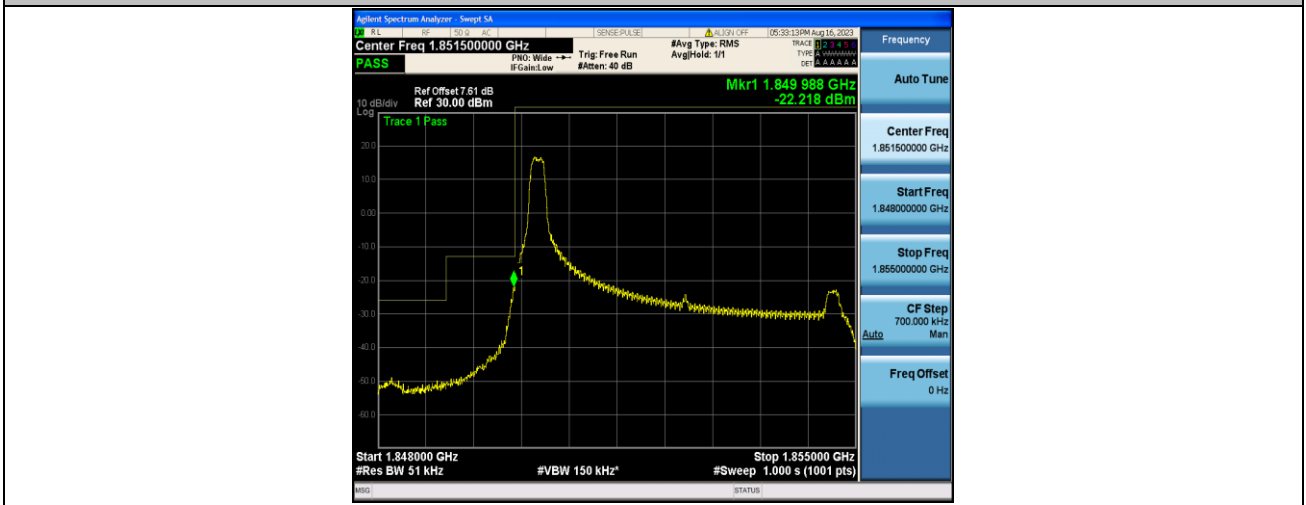
Band2_5MHz_QPSK_18625_1RB#0
