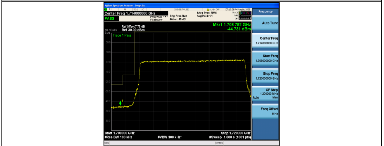
Band4_10MHz_QPSK_20000_50RB#0
