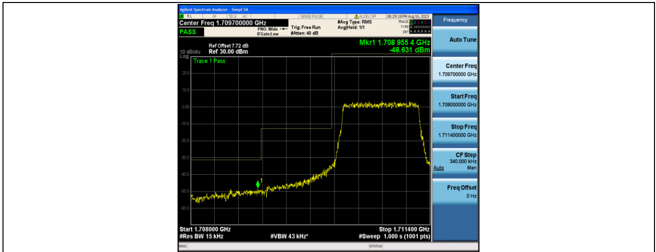
Band4_1.4MHz_16QAM_19957_6RB#0
