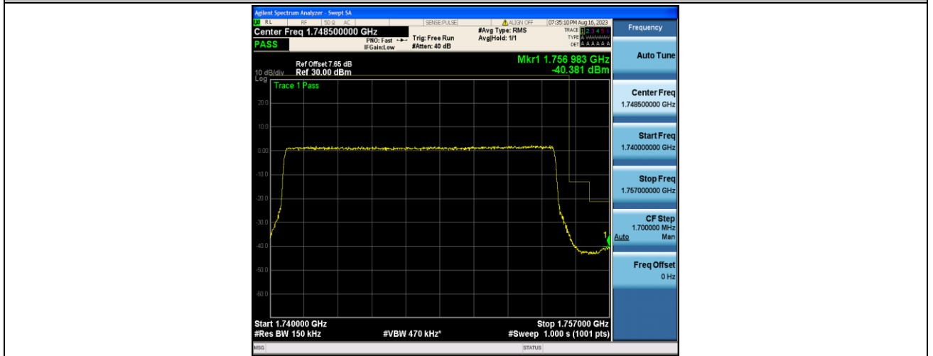
Band4_15MHz_QPSK_20325_75RB#0
