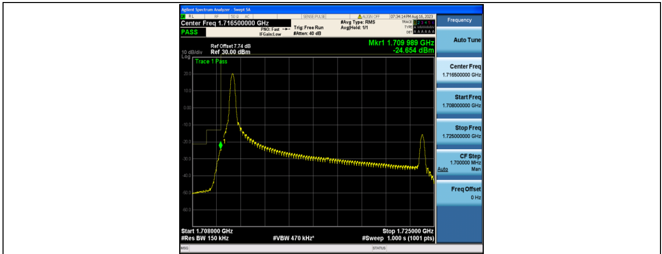
Band4_15MHz_QPSK_20025_1RB#0
