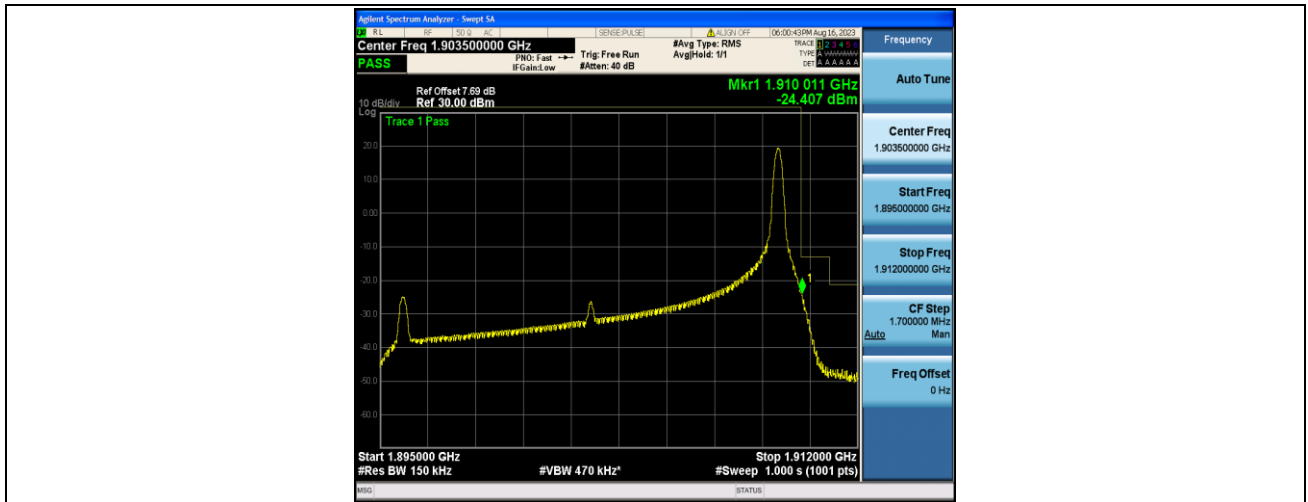
Band2_15MHz_16QAM_19125_1RB#74
