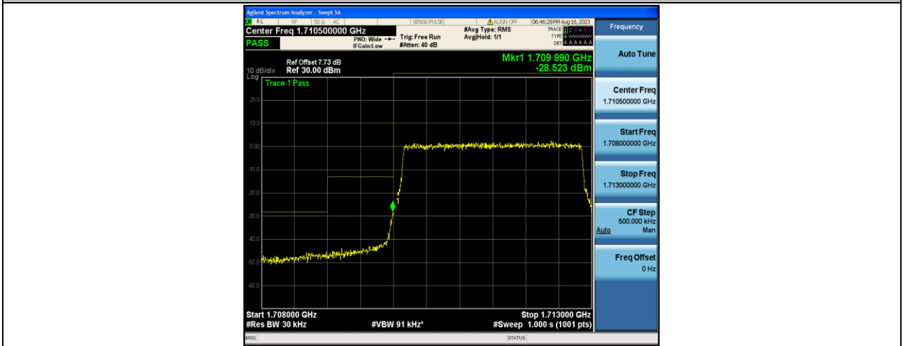
Band4_3MHz_16QAM_19965_15RB#0
