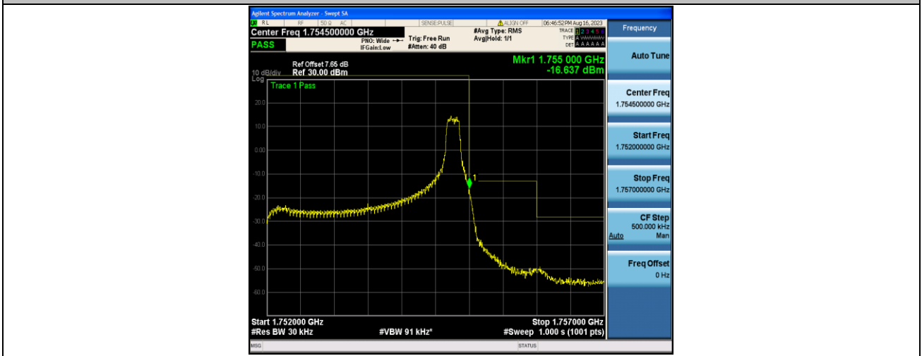
Band4_3MHz_16QAM_20385_1RB#14
