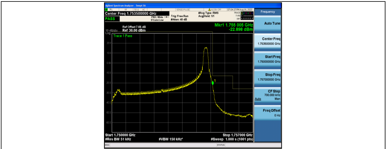
Band4_5MHz_16QAM_20375_1RB#24
