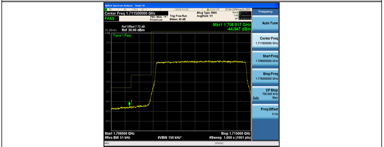
Band4_5MHz_16QAM_19975_25RB#0
