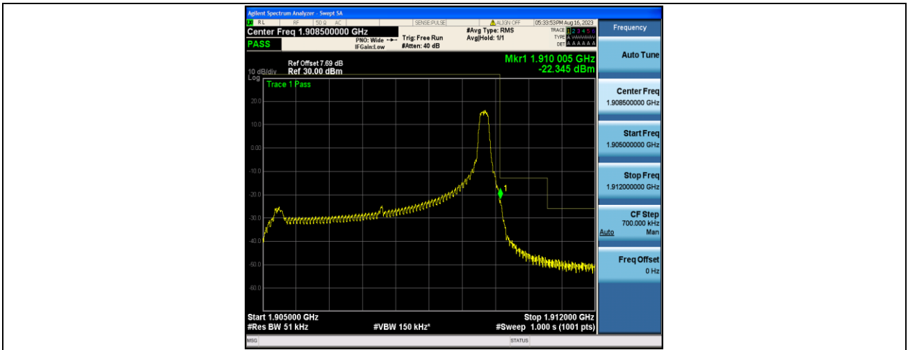
Band2_5MHz_16QAM_19175_1RB#24
