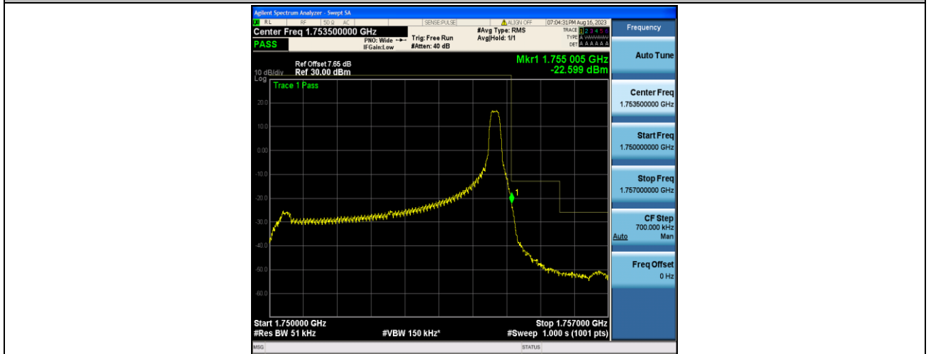
Band4_5MHz_QPSK_20375_1RB#24
