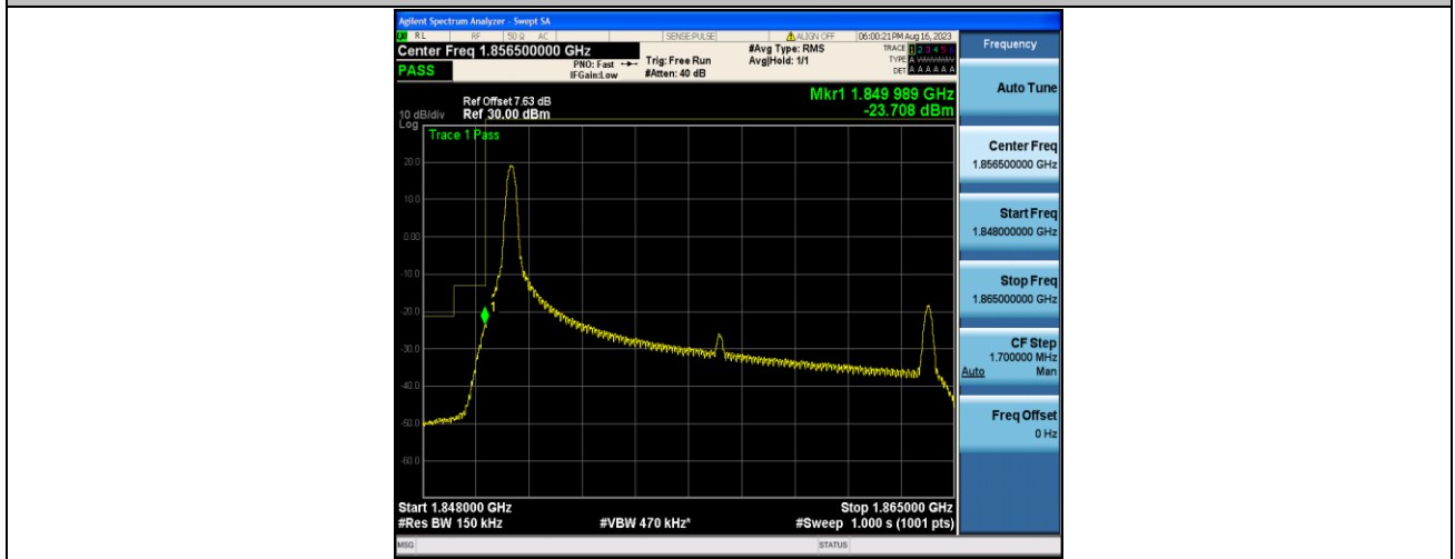
Band2_15MHz_16QAM_18675_1RB#0
