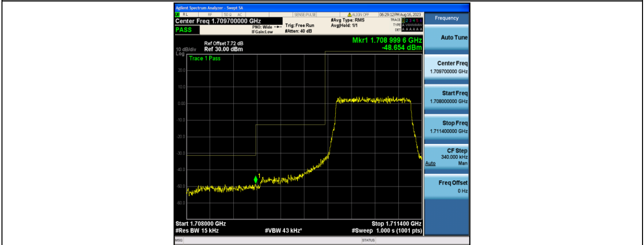
Band4_1.4MHz_QPSK_19957_6RB#0
