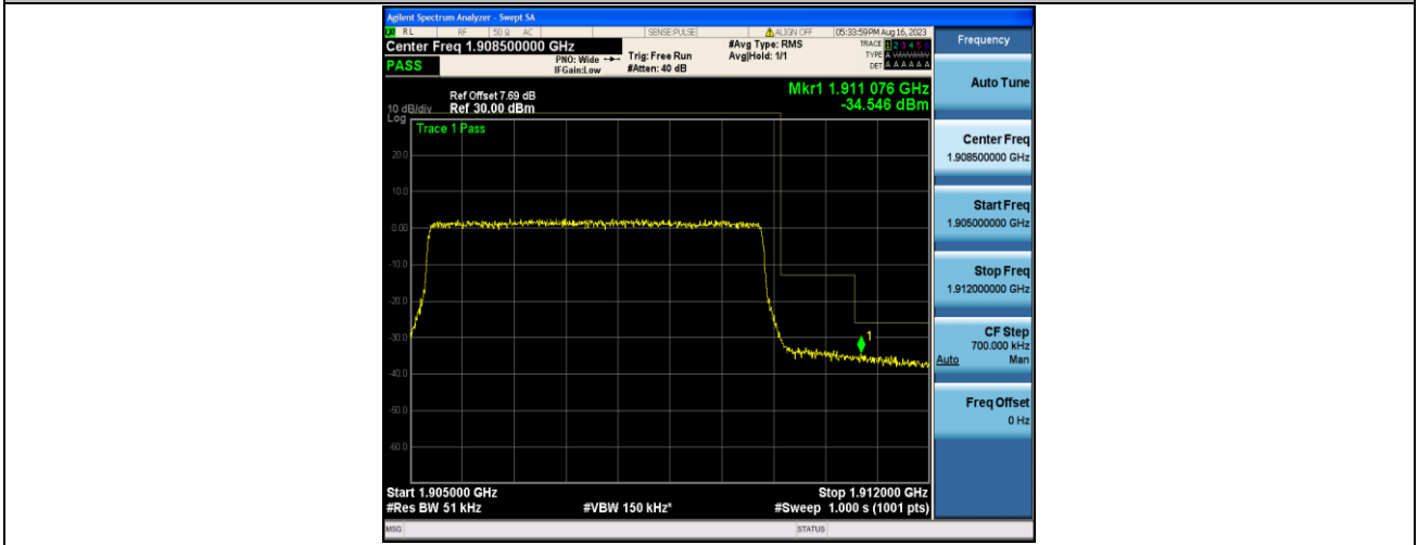
Band2_5MHz_QPSK_19175_25RB#0
