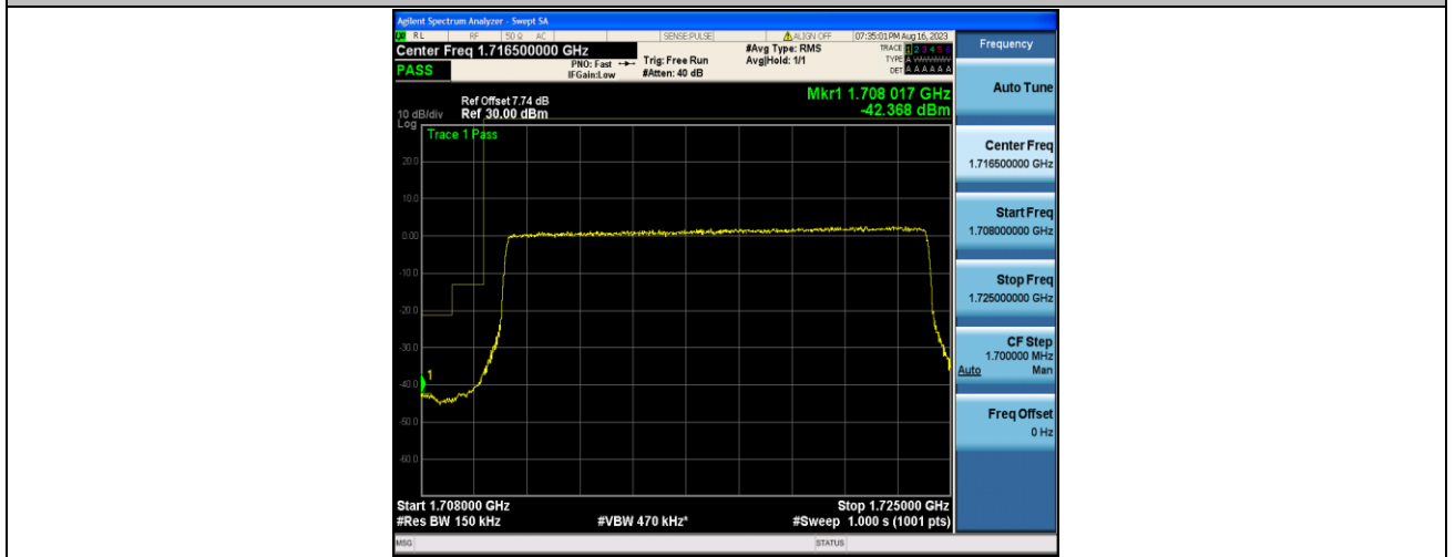
Band4_15MHz_QPSK_20025_75RB#0
