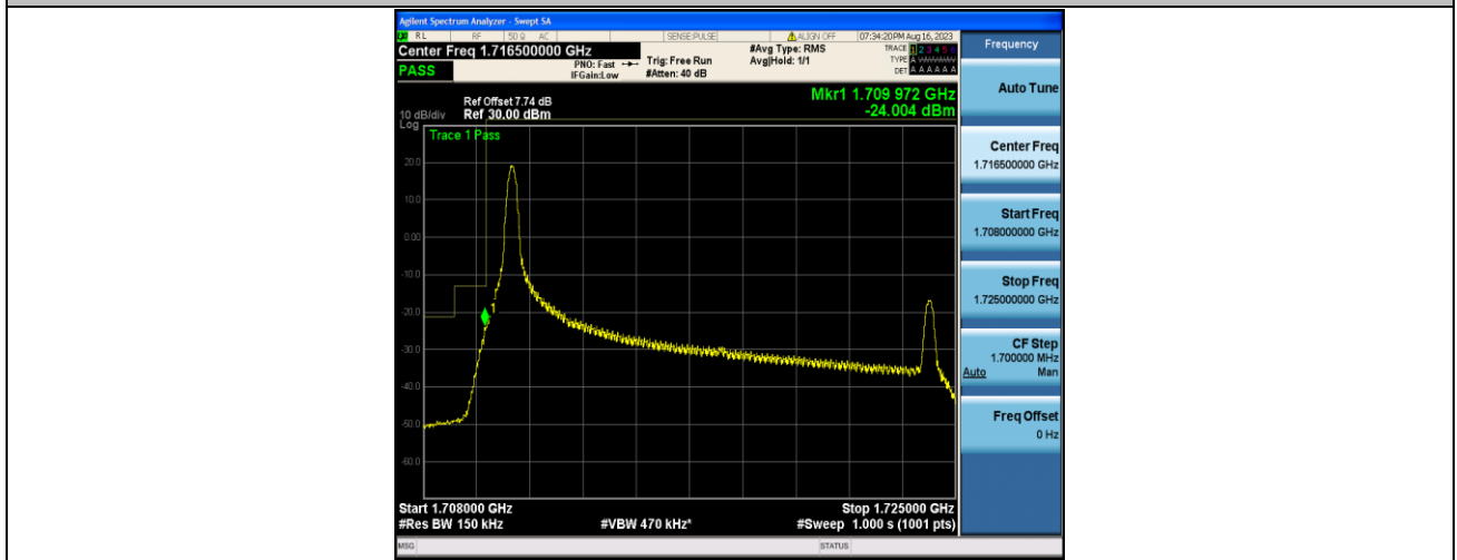
Band4_15MHz_16QAM_20025_1RB#0
