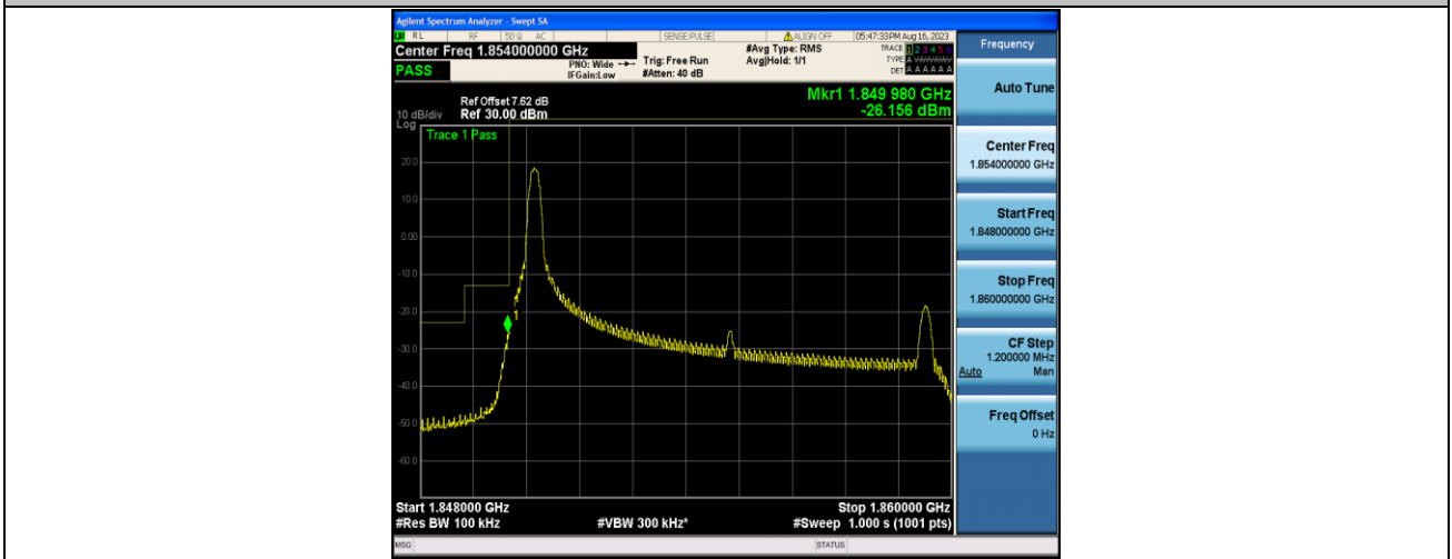
Band2_10MHz_16QAM_18650_1RB#0
