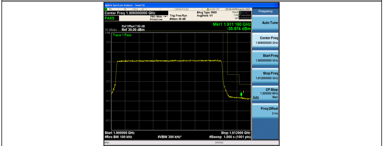
Band2_10MHz_QPSK_19150_50RB#0
