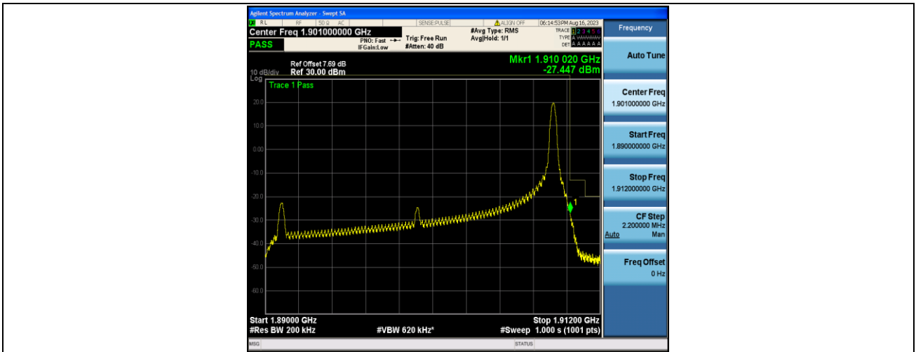
Band2_20MHz_16QAM_19100_1RB#99
