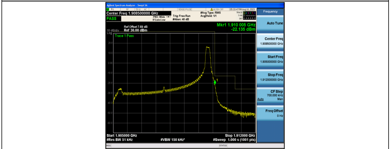
Band2_5MHz_QPSK_19175_1RB#24
