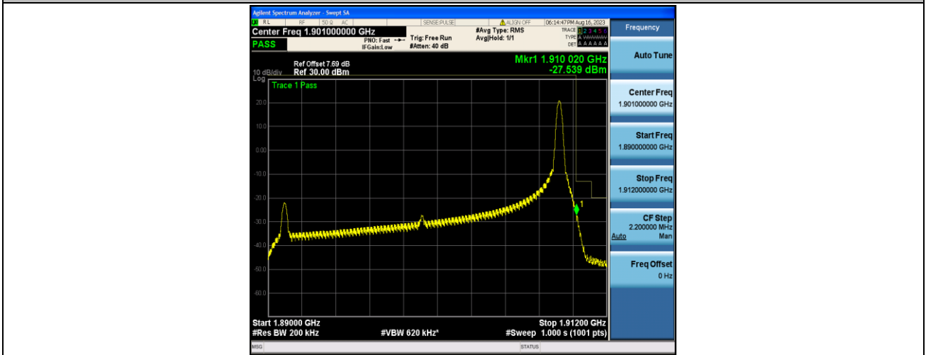
Band2_20MHz_QPSK_19100_1RB#99
