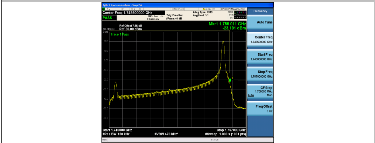
Band4_15MHz_QPSK_20325_1RB#74
