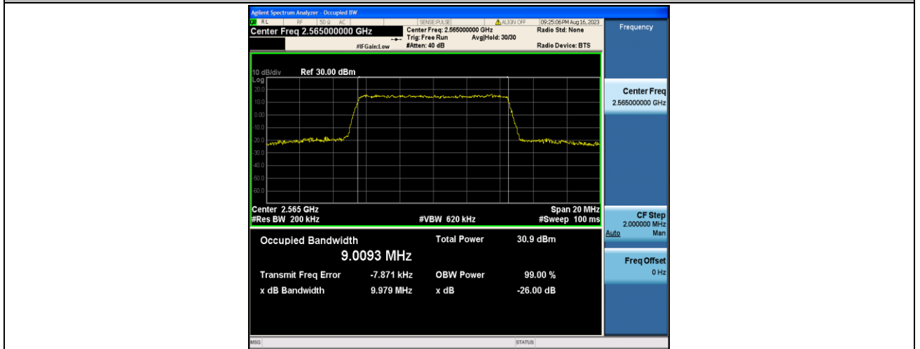
Band7-10MHz-QPSK-21400-50RB#0-PASS
