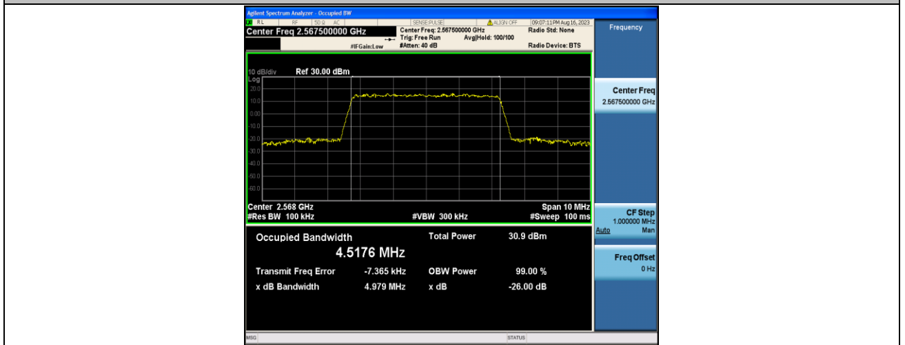
Band7-5MHz-QPSK-21425-25RB#0-PASS
