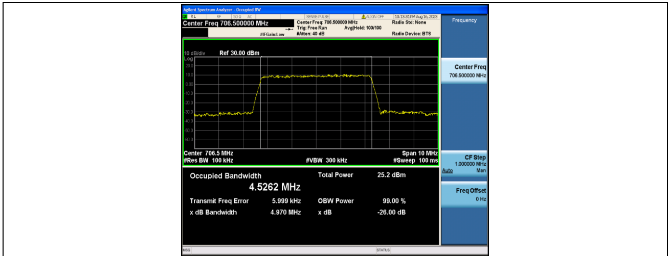
Band17-5MHz-QPSK-23755-25RB#0-PASS
