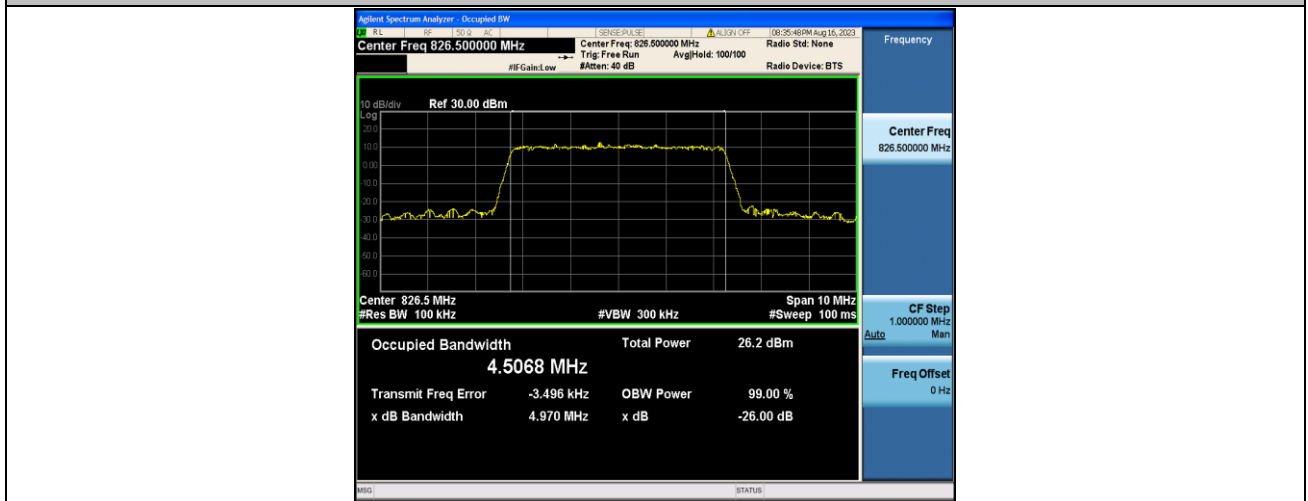
Band5-5MHz-16QAM-20425-25RB#0-PASS
