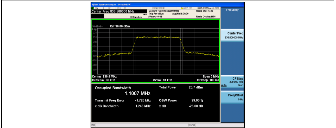
Band5-1.4MHz-QPSK-20525-6RB#0-PASS
