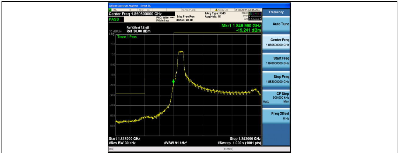
Band2_3MHz_16QAM_18615_1RB#0
