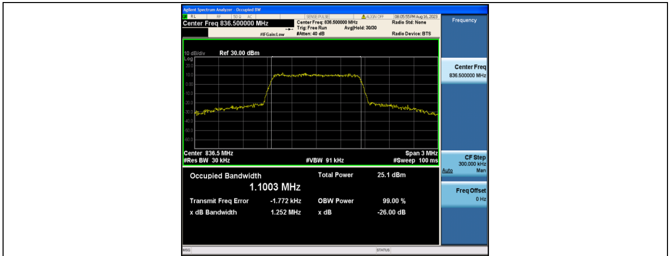
Band5-1.4MHz-16QAM-20525-6RB#0-PASS
