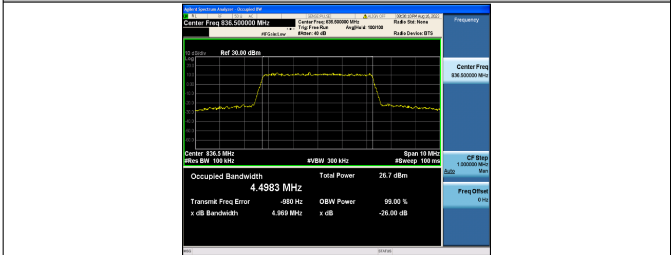
Band5-5MHz-QPSK-20525-25RB#0-PASS
