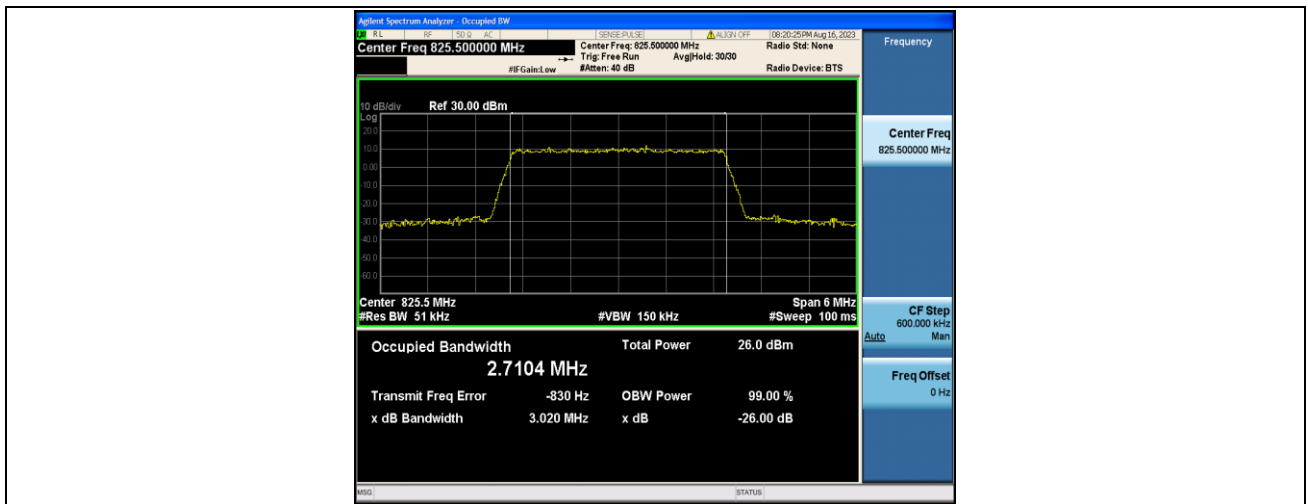
Band5-3MHz-QPSK-20415-15RB#0-PASS
