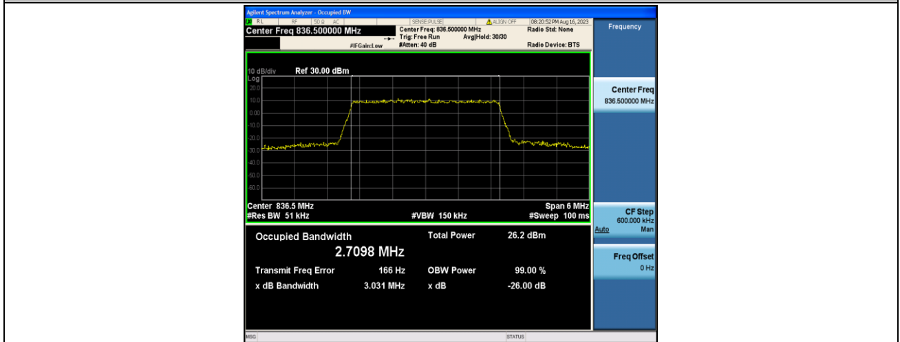
Band5-3MHz-QPSK-20525-15RB#0-PASS
