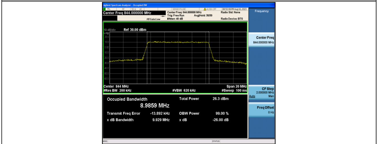
Band5-10MHz-QPSK-20600-50RB#0-PASS
