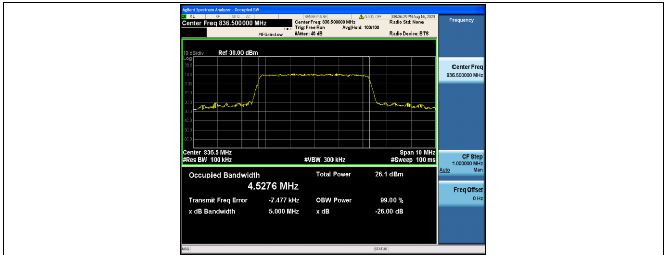
Band5-5MHz-16QAM-20525-25RB#0-PASS
