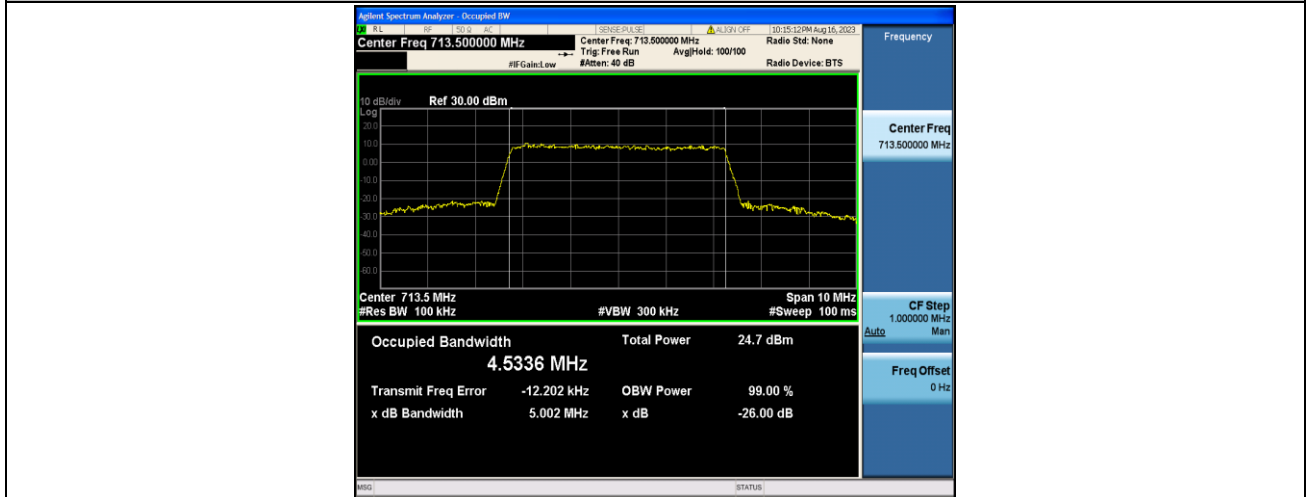
Band17-5MHz-16QAM-23825-25RB#0-PASS
