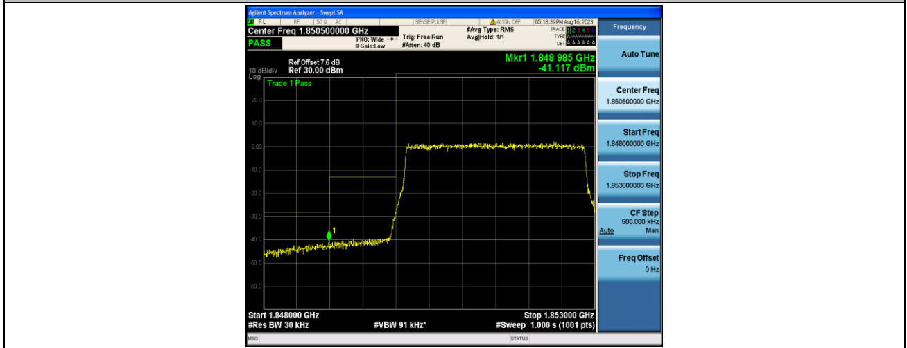
Band2_3MHz_16QAM_18615_15RB#0
