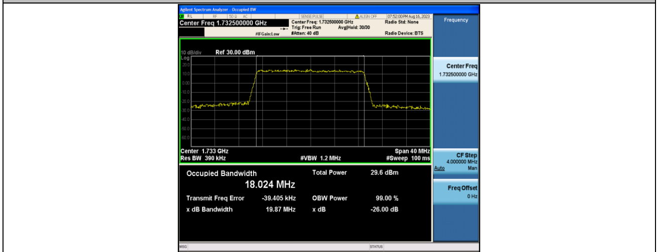
Band4-20MHz-QPSK-20175-100RB#0-PASS
