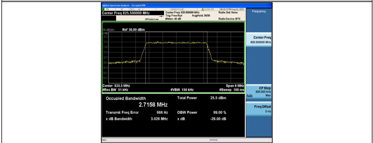
Band5-3MHz-16QAM-20415-15RB#0-PASS
