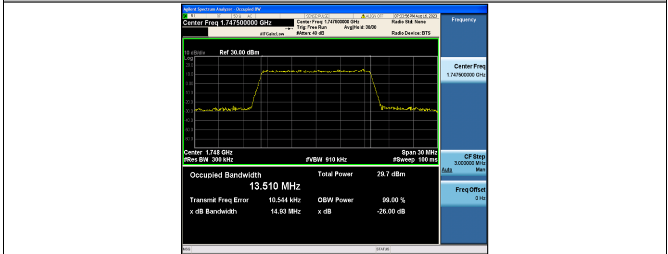
Band4-15MHz-QPSK-20325-75RB#0-PASS
