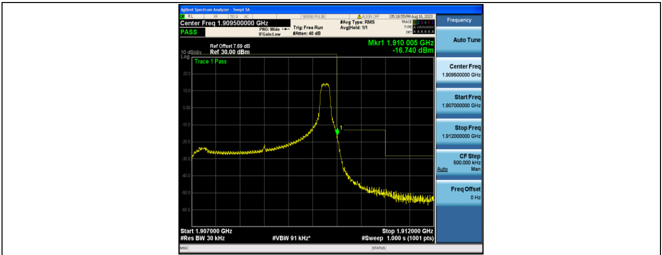
Band2_3MHz_QPSK_19185_1RB#14
