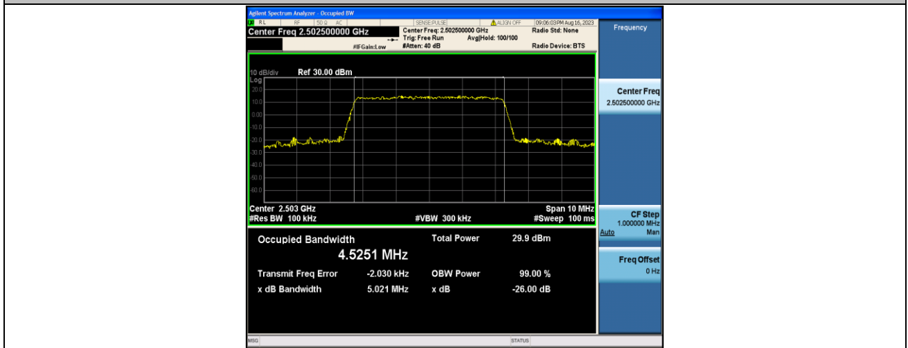
Band7-5MHz-16QAM-20775-25RB#0-PASS
