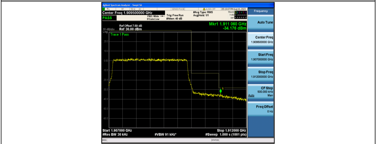
Band2_3MHz_QPSK_19185_15RB#0
