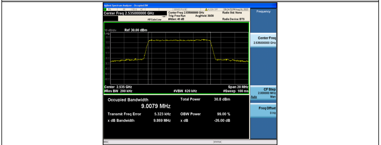
Band7-10MHz-QPSK-21100-50RB#0-PASS
