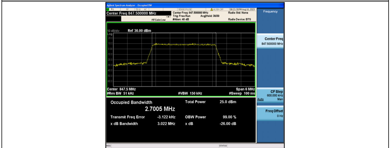
Band5-3MHz-16QAM-20635-15RB#0-PASS
