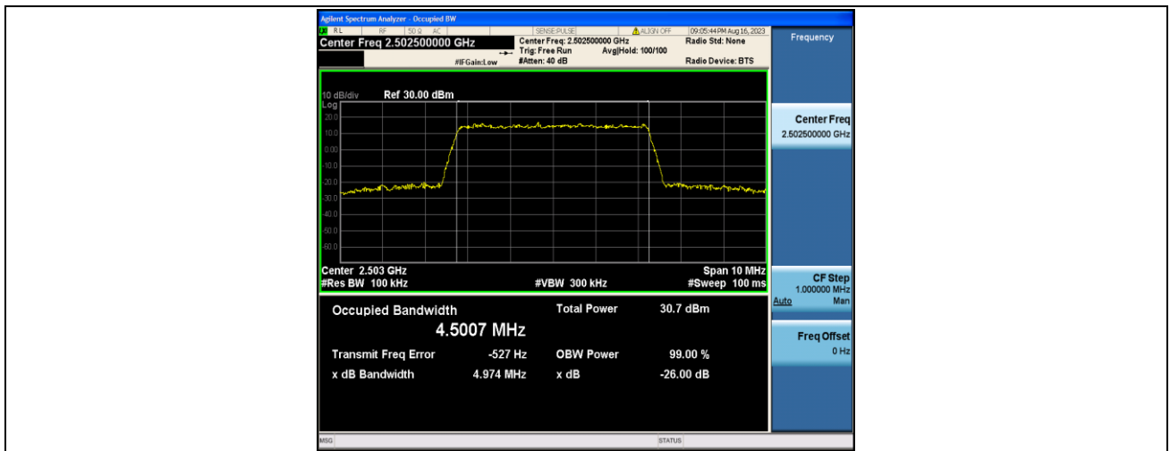
Band7-5MHz-QPSK-20775-25RB#0-PASS
