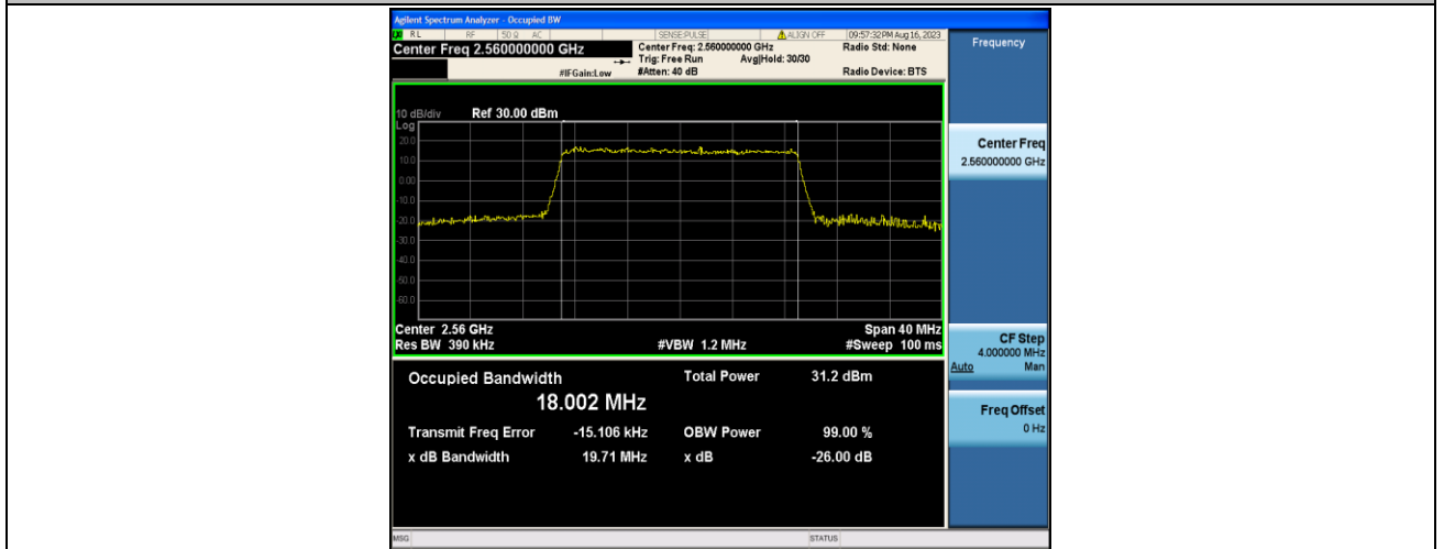
Band7-20MHz-QPSK-21350-100RB#0-PASS
