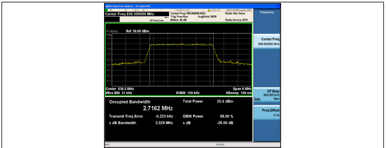
Band5-3MHz-16QAM-20525-15RB#0-PASS
