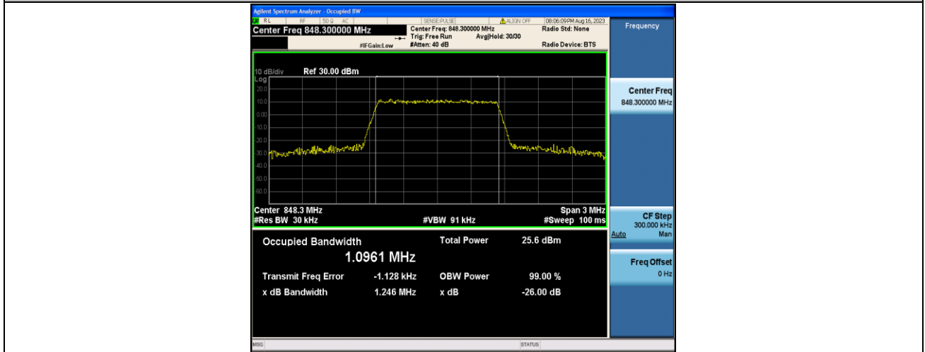
Band5-1.4MHz-QPSK-20643-6RB#0-PASS
