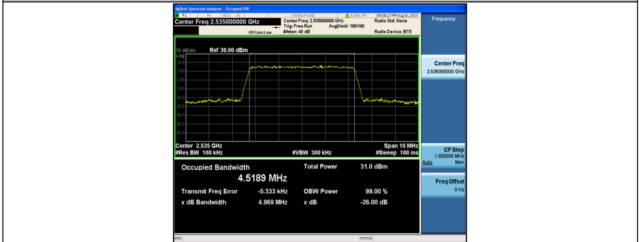
Band7-5MHz-QPSK-21100-25RB#0-PASS
