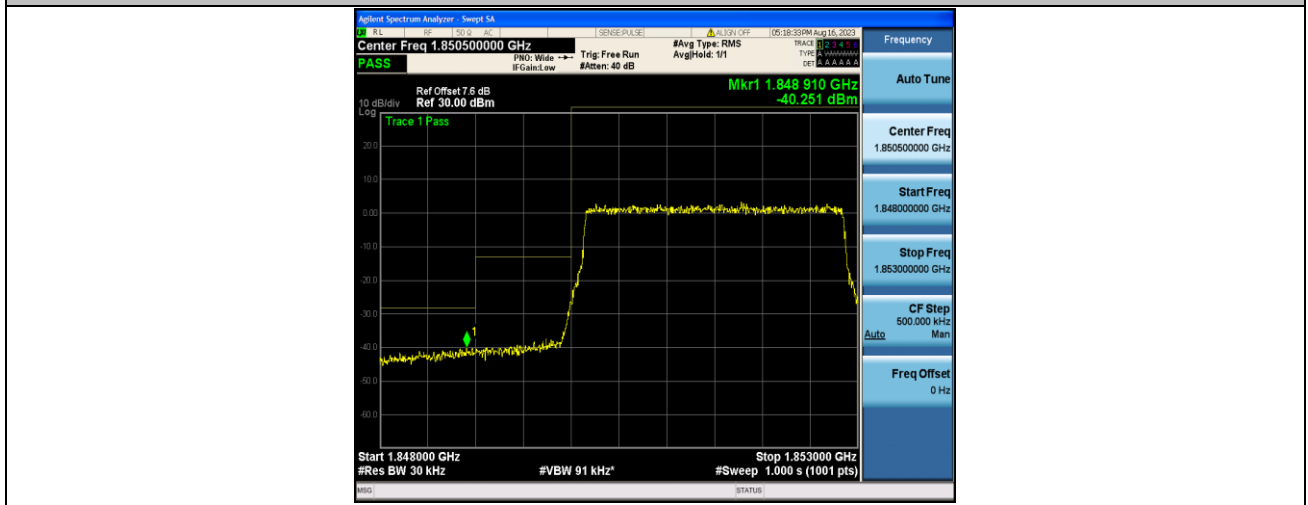
Band2_3MHz_QPSK_18615_15RB#0
