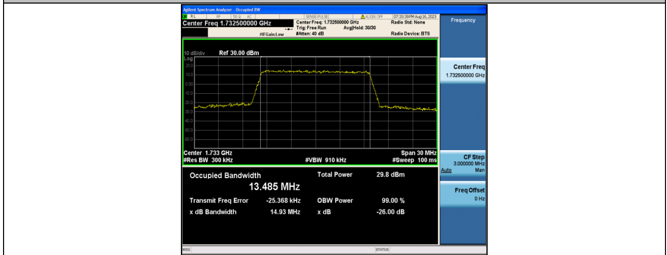
Band4-15MHz-QPSK-20175-75RB#0-PASS
