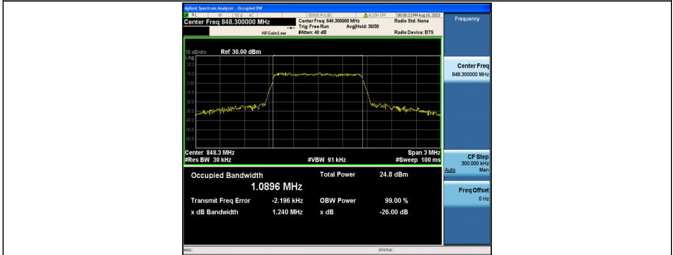
Band5-1.4MHz-16QAM-20643-6RB#0-PASS
