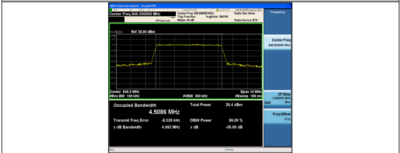
Band5-5MHz-QPSK-20625-25RB#0-PASS
