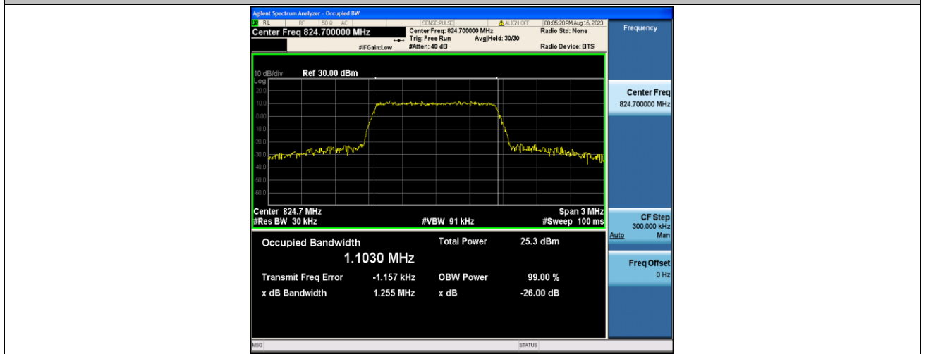
Band5-1.4MHz-16QAM-20407-6RB#0-PASS
