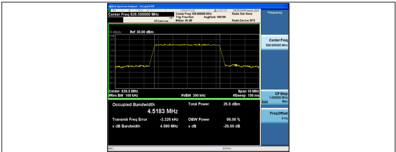
Band5-5MHz-QPSK-20425-25RB#0-PASS
