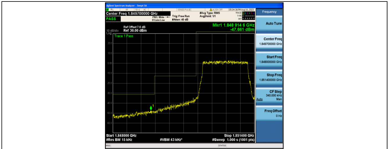
Band2_1.4MHz_16QAM_18607_6RB#0
