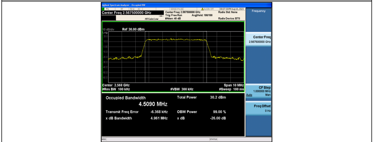
Band7-5MHz-16QAM-21425-25RB#0-PASS
