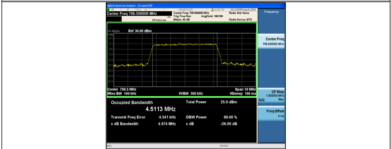
Band17-5MHz-16QAM-23755-25RB#0-PASS
