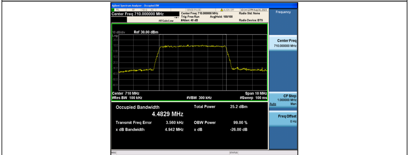
Band17-5MHz-QPSK-23790-25RB#0-PASS
