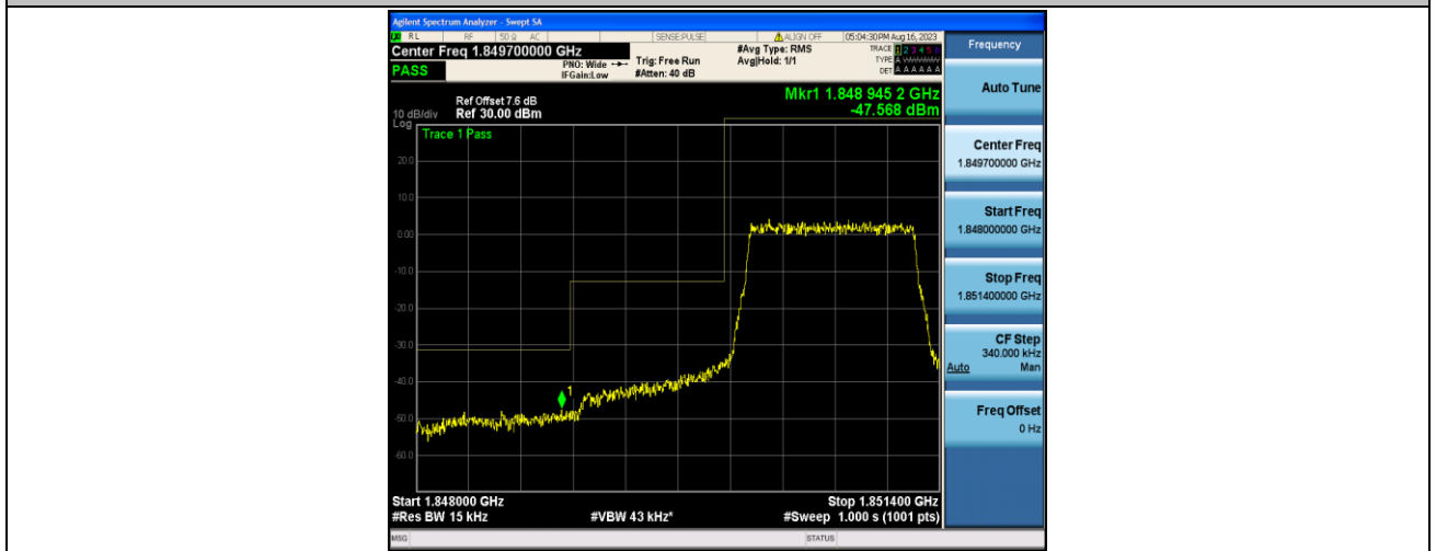
Band2_1.4MHz_QPSK_18607_6RB#0
