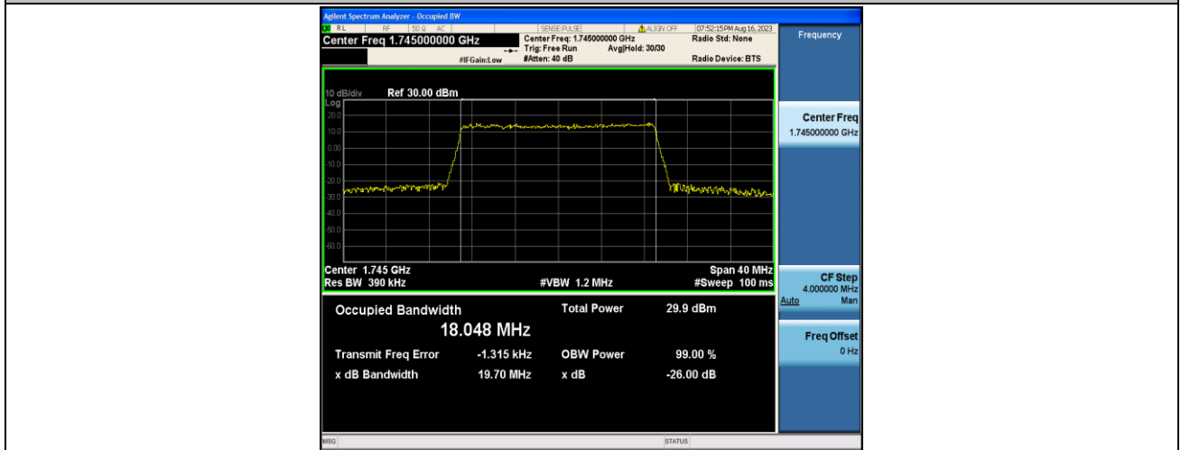
Band4-20MHz-QPSK-20300-100RB#0-PASS
