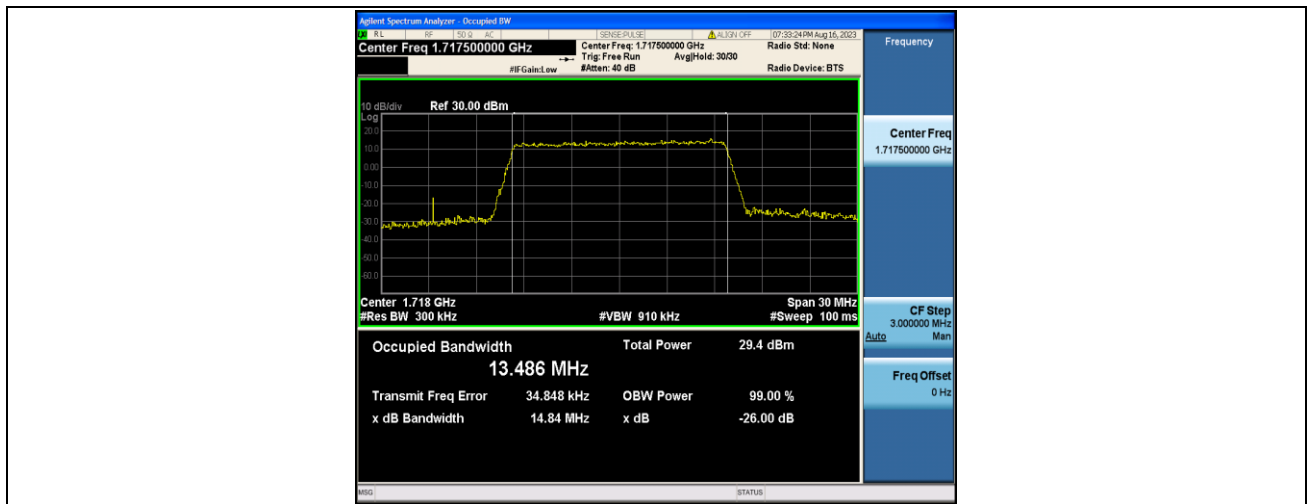
Band4-15MHz-QPSK-20025-75RB#0-PASS
