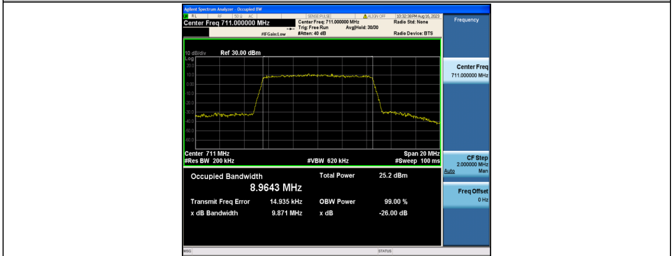
Band17-10MHz-QPSK-23800-50RB#0-PASS
